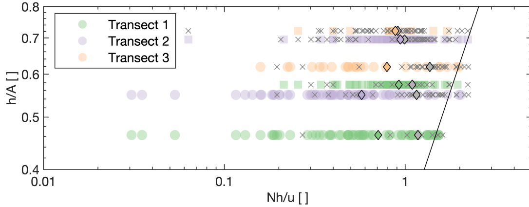
Figure 9. Observational periods with recirculation (colored markers) and without recirculation (gray cross marks) under stratified conditions as a function of mean lee-side slope ( h/A ) and Nh/u . The round markers refer to recirculation at the southwest ridge and the square markers to northeast ridge. The colored diamond markers show the mean value of Nh/u per transect during periods with recirculation and the gray markers the mean for periods without recirculation. The solid black line shows where NA/u = \pi .
