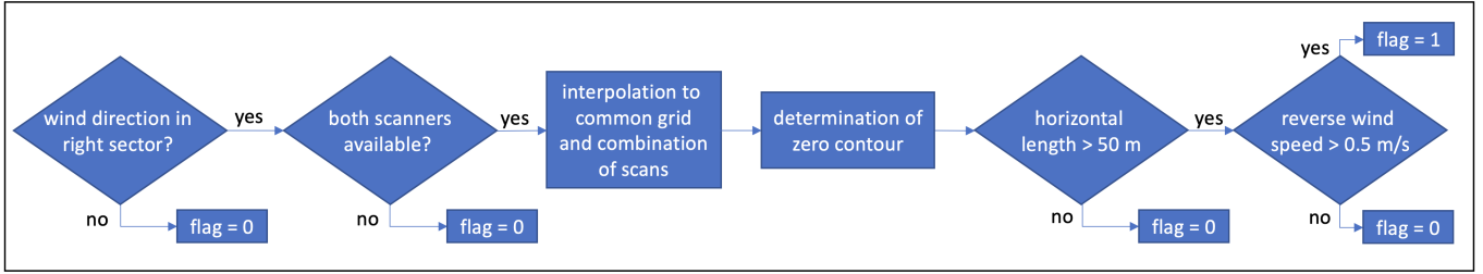
Figure 5. Flow diagram of recirculation zone detection process. Recirculation is detected for periods that are flagged with "1", no recirculation is detected for periods flagged with "0".
