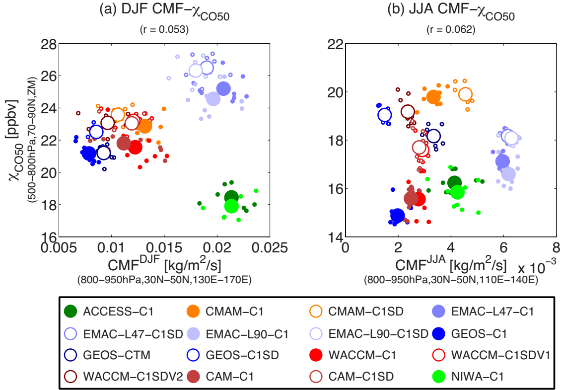
Figure 3. Correlation between Arctic CO50 concentration \chi_{CO50} (units: ppbv) and low-level midlatitude CMF (units: \text{kg}/\text{m}^2/\text{s} ) in (a) DJF and (b) JJA. Arctic \chi_{CO50} is here the vertical average of 500 hPa - 800 hPa, latitudinal average of 70°N - 90°N, and zonal mean (ZM). CMF is here the vertical average of 800 hPa - 950 hPa, latitudinal average of 30°N - 50°N in both DJF and JJA, while longitudinal average window differs between seasons, as DJF CMF highlights the robust convection over the western Pacific Ocean (130°E-170°E) whereas JJA CMF focuses on the maritime convection over the East Asia (110°E-140°E) following Orbe et al. (2018). Large marks denote the 2000-2009 climatology (except GEOS-C1 and GEOS-C1SD) while small marks denote the corresponding interannual variations of each simulation. Results for C1 simulations are shown as filled circles while C1SD simulations are denoted by open circles. Results of least squares fitting based on climatological means are shown as the solid black lines, and the corresponding Pearson correlation coefficients are given in parentheses in the titles. If this correlation coefficient is significant (95%), a corresponding linear regression is derived using the total least square method (Petraš and Bednárová, 2010).
