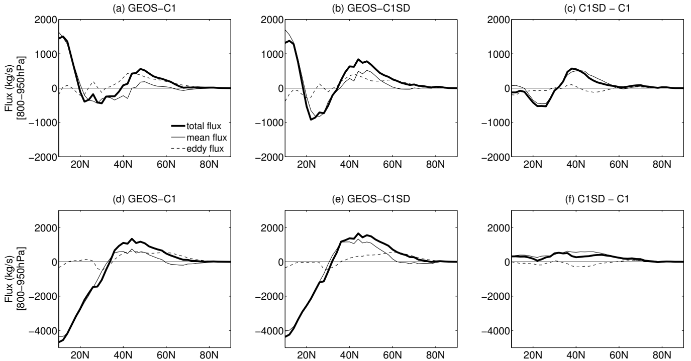
Figure 8. Tracer flux diagnostics showing the total flux \langle \overline{v \chi_{CO50}} \rangle (heavy), zonal mean flux \langle \overline{v \overline{\chi_{CO50}}} \rangle (light, solid) and eddy flux \langle \overline{v' \chi'_{CO50}} \rangle (light, dashed) of CO50 (vertically integrated from 800 hPa to 950 hPa; positive means northward; units: kg/s) in (a) GEOS-C1, (b) GEOS-C1SD, and (c) the difference GEOS-C1SD - GEOS-C1 during summer. (d,e,f) are similar to (a,b,c) but during winter. Results are based on the daily GEOS model output.
