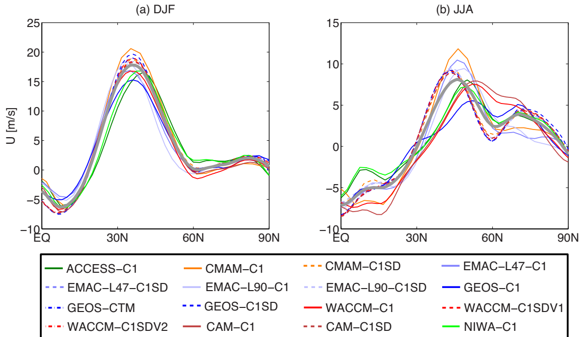
Figure 4. Multi-model spread of latitudinal profile of zonal wind u vertically averaged between 500 hPa and 800 hPa and longitudinally averaged over the Pacific Ocean ( 135^{\circ}\text{E} - 135^{\circ}\text{W} ) during (a) DJF and (b) JJA. C1 simulations are shown in solid lines while C1SD simulations are shown in either dashed or dotted-dashed lines. The corresponding ensemble means are depicted as the heavy gray lines.
