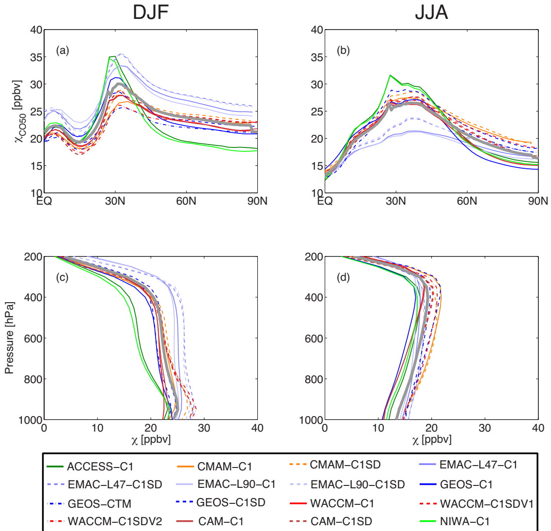
Figure 2. (a,b) Latitudinal and (c,d) vertical variations of zonal mean CO50 concentration \chi_{CO50} (units: ppbv) for each model during (a,c) DJF and (b,d) JJA. The corresponding ensemble means are depicted as the heavy gray lines. In (a,b), \chi_{CO50} are averaged in the middle and lower troposphere (500-800 hPa); whereas in (c,d), \chi_{CO50} are averaged over the Arctic (70°N-90°N). Note that C1 simulations are shown as solid lines while C1SD simulations are shown as dashed or dotted-dashed lines.
