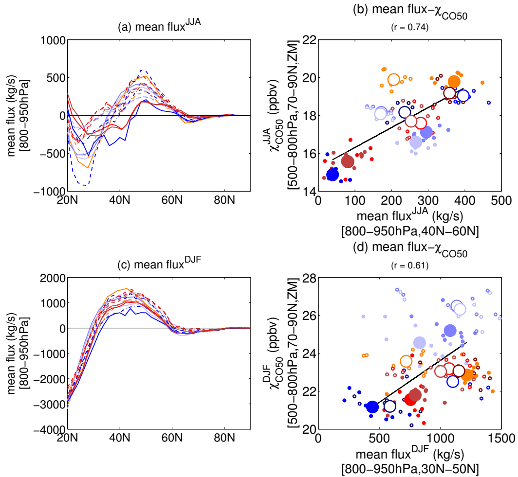
Figure 9. Approximated zonal-mean flux using monthly output: (a,c) latitudinal profile of \langle \bar{v} \overline{\chi_{CO50}} \rangle (units: kg/s); (b,d) correlation between the zonal-mean flux (latitudinal average of 40°N - 60°N during JJA and 30°N - 50°N during DJF) and the Arctic CO50 concentration (vertical average of 500 hPa - 800 hPa, latitudinal average of 70°N - 90°N, and zonal mean (ZM), units: ppbv), during JJA in (a,b) and during DJF in (c,d).
