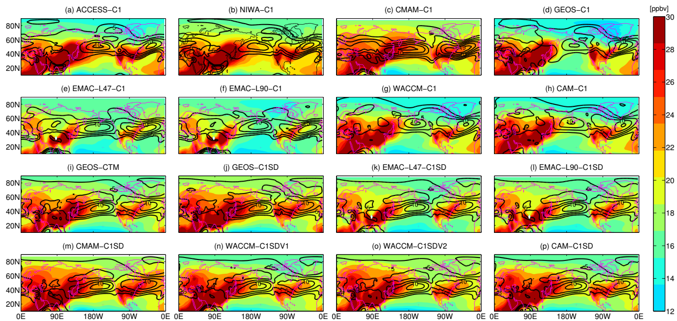
Figure 5. Maps of 500 hPa - 800 hPa averaged CO 50 distribution (shades, units: ppbv) and the corresponding 500-800 hPa averaged u during JJA in each CCM simulation. C1 simulations are shown in the top two rows while C1SD simulations are shown in the bottom two rows.
