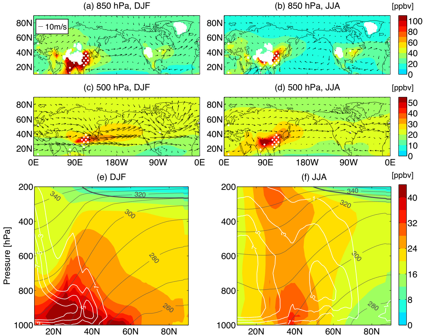
Figure 1. Ensemble mean of the horizontal distribution of CO50 concentration (shades, units: ppbv) at levels of (a,b) 850 hPa and (c,d) 500 hPa, and ensemble mean of the zonal-mean CO50 concentration cross sections (e,f) during (a,c,e) DJF and (b,d,f) JJA. In (a,b,c,d), horizontal winds ( u,v ) are overlaid as vectors and regions of CO50 sources are highlighted by white stipples within which CO50 emission fluxes are larger than 0.4 \times 10^{-9} \text{ kg/m}^2/\text{s} . In (e,f), isentropic surfaces are overlaid as dark gray isopleths (units: K), the tropopause is marked as the bold dark gray curve, and regional convective mass flux (CMF) over the East Asia ( 110^\circ\text{E} - 140^\circ\text{E} ) are denoted by white contours (units: 10^{-3} \text{ kg/m}^2/\text{s} ).
