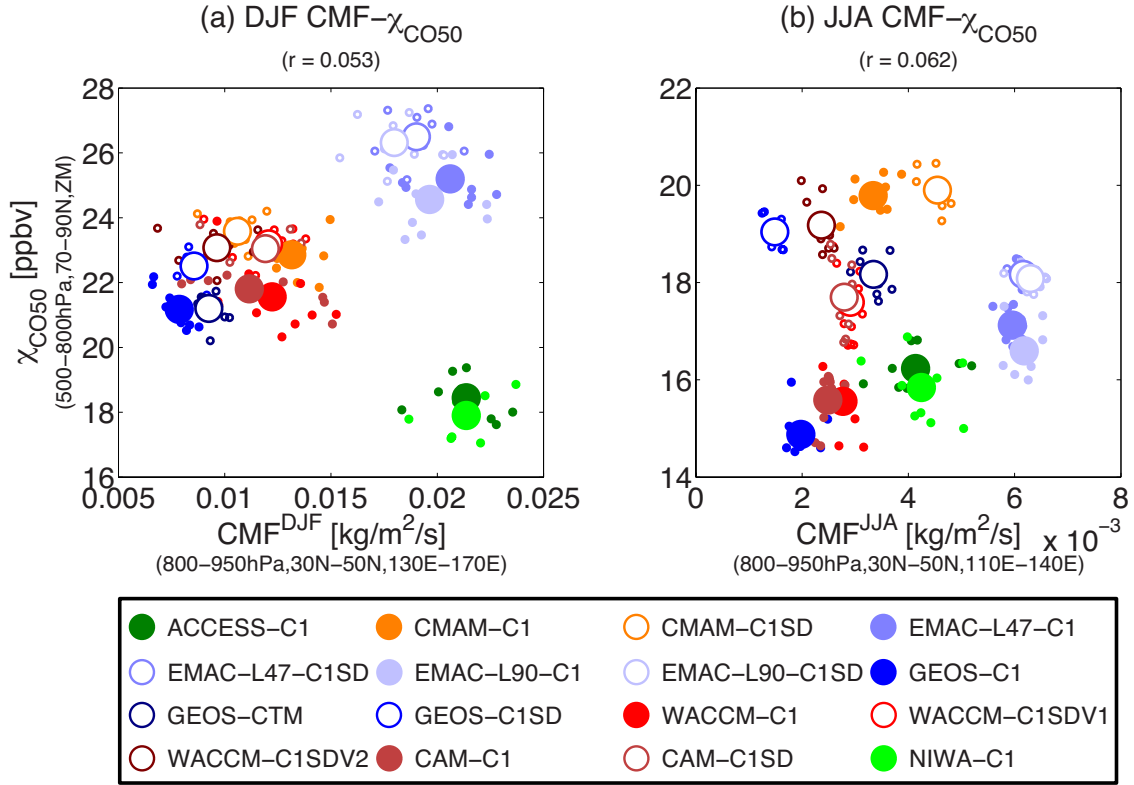
Figure 3. Correlation between Arctic CO 50 concentration \chi_{\text{CO}_50} (units: ppbv) and low-level midlatitude CMF (units: kg/m 2 /s) in (a) DJF and (b) JJA. Arctic \chi_{\text{CO}_50} is here the vertical average of 500 hPa - 800 hPa, latitudinal average of 70°N - 90°N, and zonal mean (ZM). CMF is here the vertical average of 800 hPa - 950 hPa, latitudinal average of 30°N - 50°N in both DJF and JJA, while longitudinal average window differs between seasons, as DJF CMF highlights the robust convection over the western Pacific Ocean (130°E-170°E) whereas JJA CMF focuses on the maritime convection over the East Asia (110°E-140°E) following Orbe et al. (2018). Large marks denote the 2000-2009 climatology (except GEOS-C1 and GEOS-C1SD) while small marks denote the corresponding interannual variations of each simulation. Results of least squares fitting based on climatological means are shown as the solid black lines, and the corresponding Pearson correlation coefficients are given in parentheses in the titles. If this correlation coefficient is significant (95%), a corresponding linear regression is derived using the total least square method (Petráš and Bednárová, 2010).
