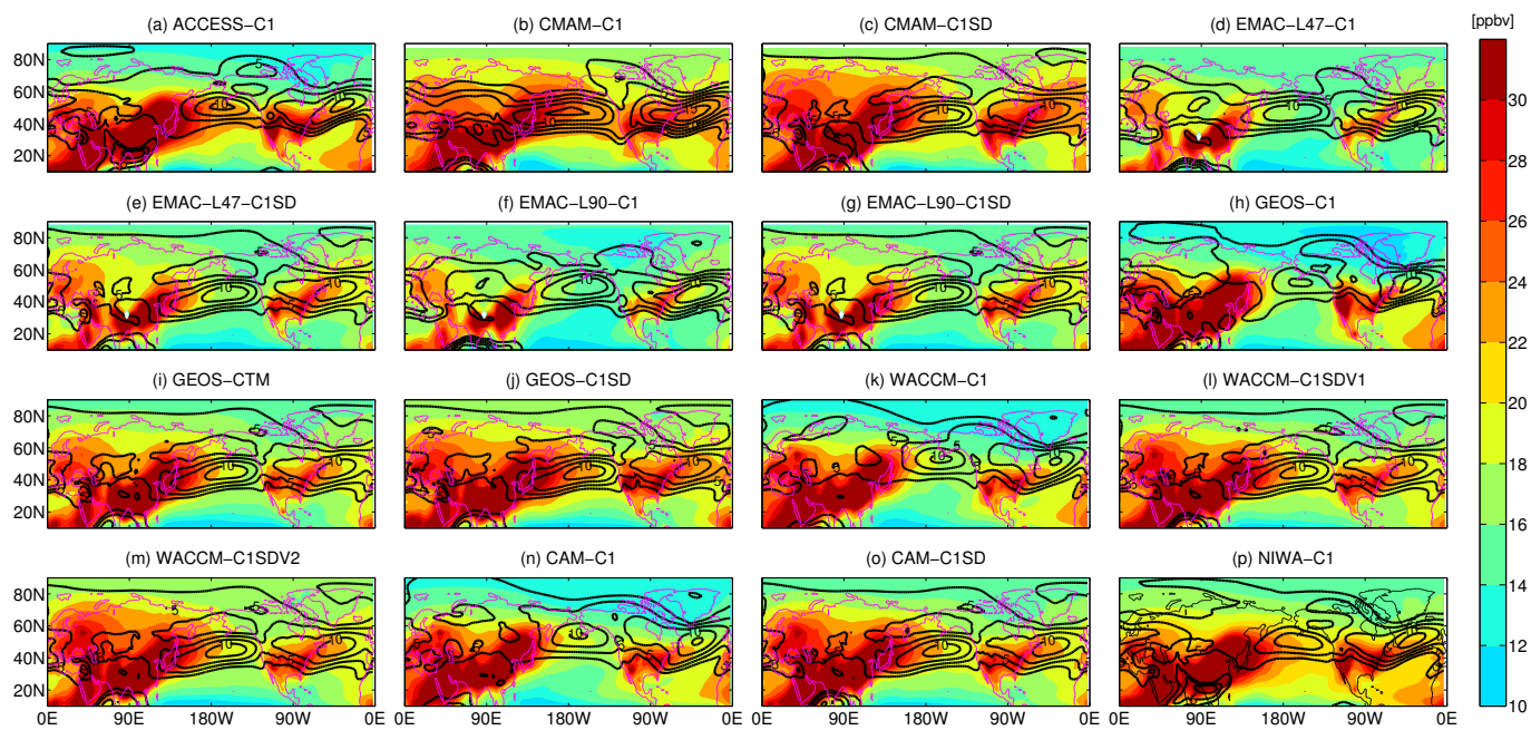
Figure 5. Maps of 500 hPa - 800 hPa averaged CO 50 distribution (shades, units: ppbv) and the corresponding 500-800 hPa averaged u during JJA in each CCMI simulation.
