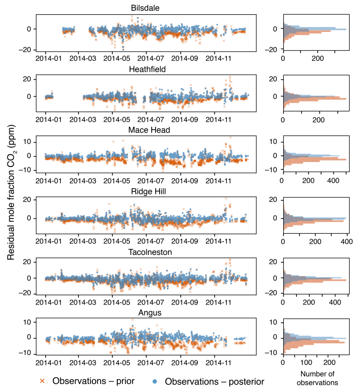
Figure S13: Left: Residual mole fractions for prior and posterior modelled \text{CO}_2 concentrations in 2014 using JULES prior biospheric fluxes. Right: Histogram of prior residuals (orange) and posterior residuals (blue). The mean of the histogram represents the mean bias.
