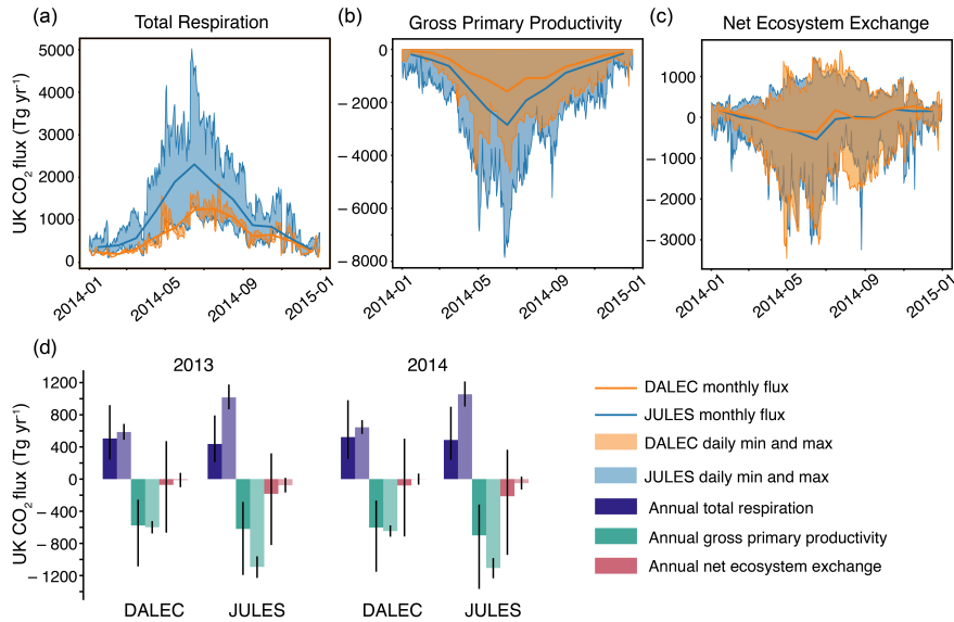
Figure S9: Posterior UK fluxes in 2014. (a-c) Comparison of monthly fluxes and minimum and maximum daily values for TER, GPP and NEE respectively resulting from JULES inversion (blue) and DALEC inversion (orange). (d) Annual CO 2 fluxes for TER, GPP and NEE for 2013 and 2014 from DALEC and JULES inversions. Dark bars denote prior annual fluxes, light bars denote posterior annual fluxes. Uncertainty bars represent 5 th – 95 th percentile.
