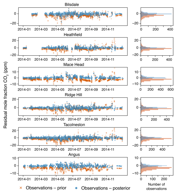
Figure S12: Left: Residual mole fractions for prior and posterior modelled \text{CO}_2 concentrations in 2014 using DALEC prior biospheric fluxes. Right: Histogram of prior residuals (orange) and posterior residuals (blue). The mean of the histogram represents the mean bias.
