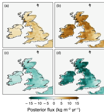
Figure S8: Posterior TER and GPP flux maps averaged over summer 2014 (June – August 2014). (a) Summer TER flux from DALEC inversion. (b) Summer TER flux from JULES inversion. (c) Summer GPP flux from DALEC inversion. (d) Summer GPP flux from JULES inversion.
