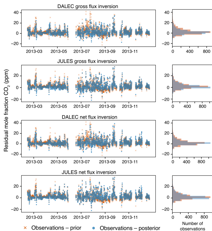
Figure S14: Left: Residual mole fractions for modelled \text{CO}_2 concentrations at Weybourne in 2013 using prior DALEC and JULES fluxes, and posterior DALEC and JULES fluxes from both the gross (scaling GPP and TER separately) and net (scaling just NEE) flux inversions. Weybourne data was not included in the inversions. Right: Histogram of residuals. The mean of the histogram represents the mean bias.
