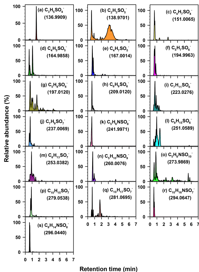
Figure 3. Extracted chromatograms of 19 major organosulfate species obtained from a PM 2.5 sample collected in Atlanta using HR TS19 -ToF (at 0.01 Da error) TS20 . Extracted chromatograms of the remaining 13 major organosulfate species are shown in Hettiyadura et al. (2017) for a PM 2.5 sample collected in Centreville. MS data, structures, and VOC precursors of these organosulfates are given in Table 1.
