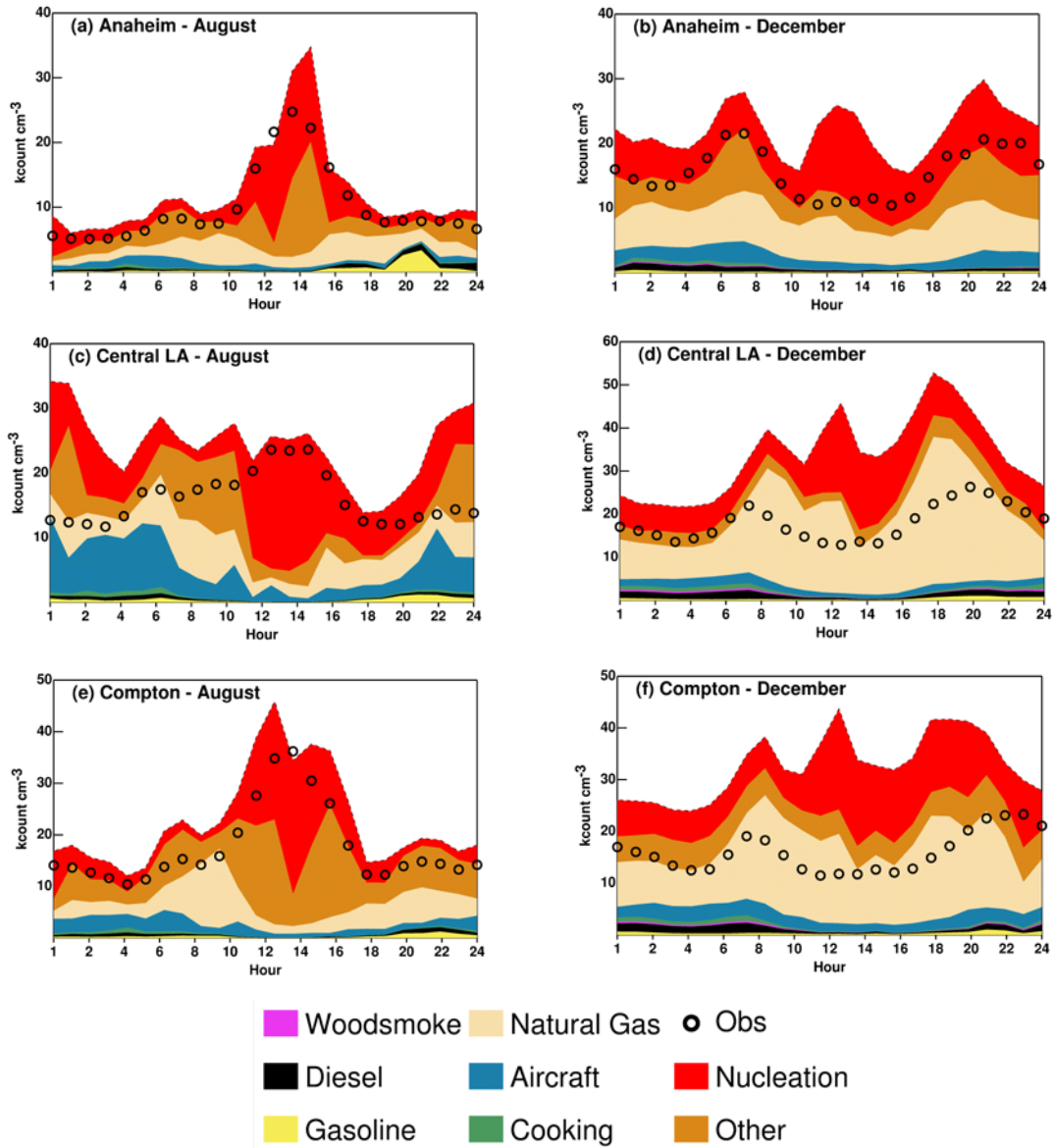
545 Figure 16: Diurnal variations of measured N_7 and predicted "best-fit" N_{10} averaged for August 2012 (left column) and December 2012 (right column) at Anaheim, Central LA, and Compton.
