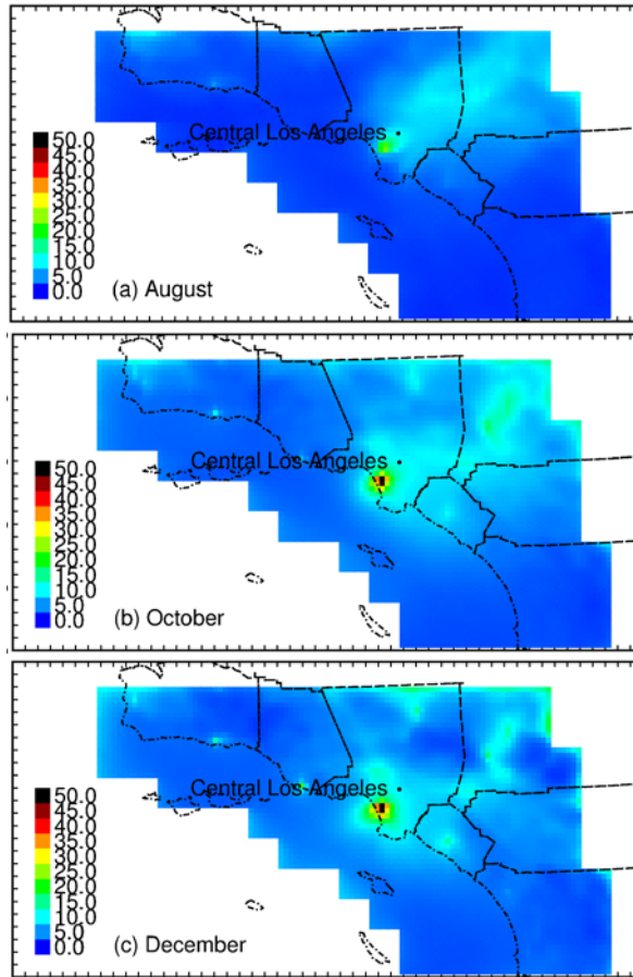
620 Figure 20: Seasonal variation of nucleated particle concentrations in Southern California. Units are \text{kcount cm}^{-3} .
