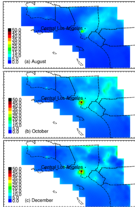
Figure 20: Seasonal variation of nucleated particle concentrations in Southern California. Units are kcount cm -3 .
