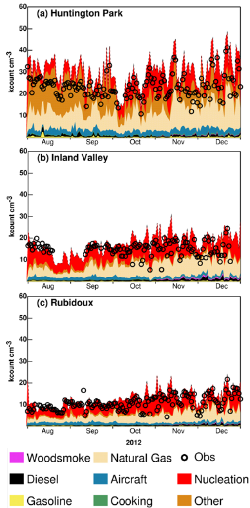
Figure 9: Seasonal variation of measured \text{N}_7 (black circles) and major source contributions to “best-fit” \text{N}_{10} at Huntington, Inland-Valley, and Rubidoux, respectively.
