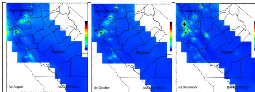
Figure 21: Seasonal variation of nucleated particle concentrations in Northern California. Units are kcount cm -3 .
