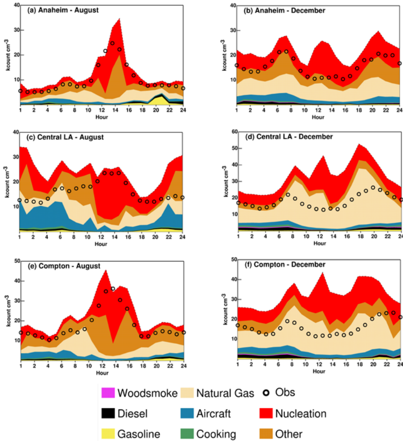
Figure 164-63: Diurnal variations of measured N_{7+1000} and predicted "best-fit" PNC-N_{10} averaged for August 2012 (left column) and December 2012 (right column) at Anaheim, Central LA, and Compton.
