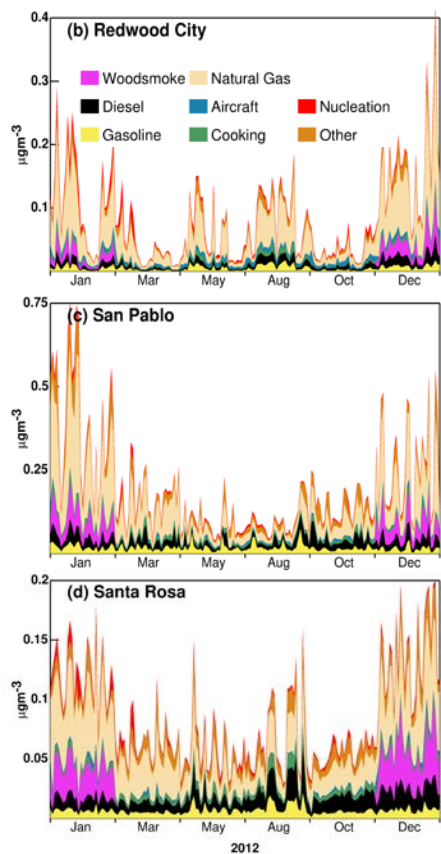
Figure 10107: Seasonal variation of major source contributions to PM 0.1 at Livermore, Redwood City, San Pablo and Santa Rosa, respectively. Results within each month have daily time resolution.
