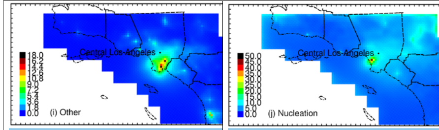
Figure 18. Spatial distribution of particle number from major sources in Southern California (unit: kcount cm -3 ).
