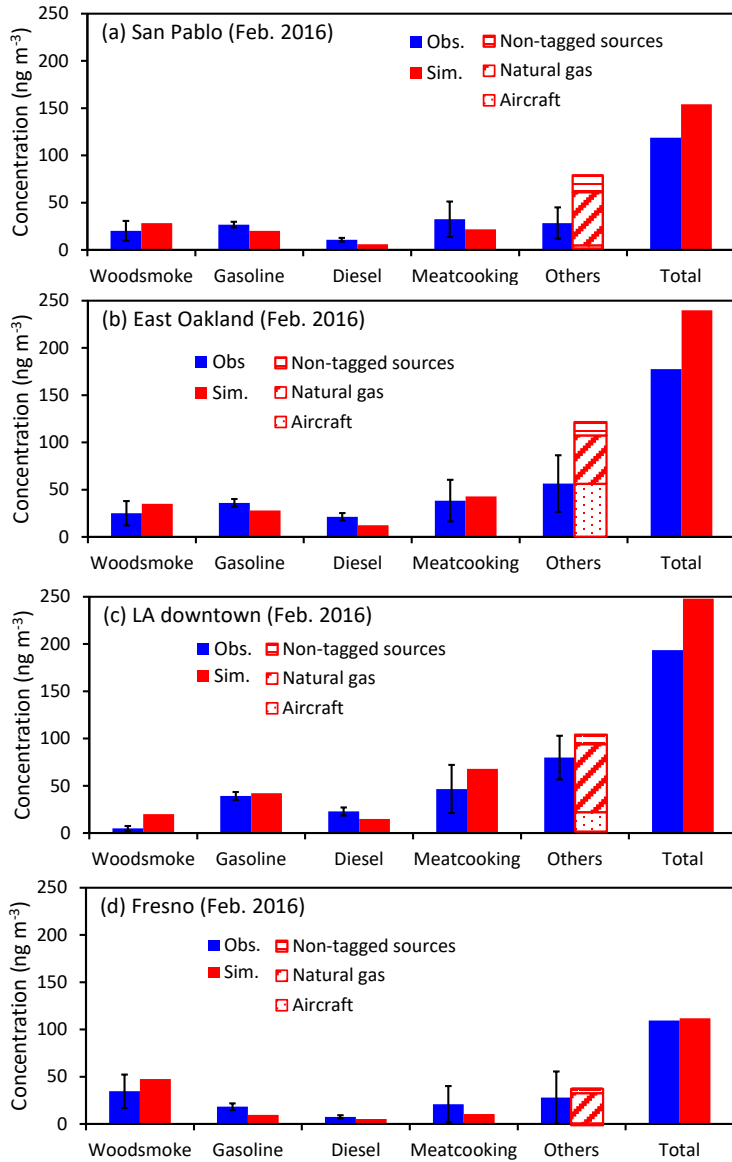
Figure 663: Source contribution to PM 0.1 predicted by the CMB receptor model and the UCD/CIT model at four sites in California in February 2016. CMB results are calculated using 3-day average measurements composited for a full month.
