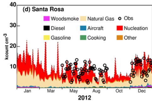
Figure 774: Seasonal variation of measured N_{7-1000} (black circles) and major source contributions to “best-fit” PNC-N_{10} at Livermore, Redwood City, San Pablo and Santa Rosa, respectively. Results within each month have daily time resolution.
