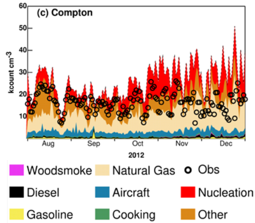
Figure 885: Seasonal variation of measured N_{7-4000} (black circles) and major source contributions to “best-fit” PNC-N_{10} at Anaheim, Central LA, and Compton, respectively. Results within each month have daily time resolution.
