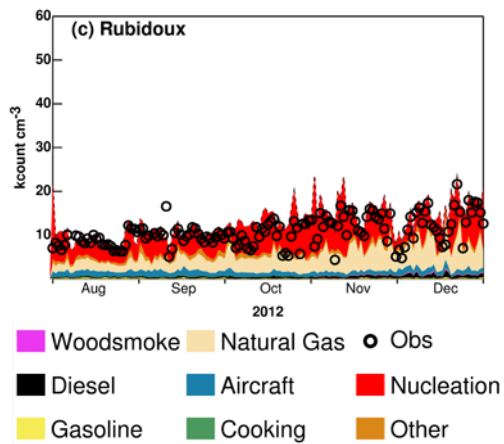
Figure 996: Seasonal variation of measured N_{7-4000} (black circles) and major source contributions to “best-fit” PNC-N_{10} at Huntington, Inland-Valley, and Rubidoux, respectively. Results within each month have daily time resolution.
