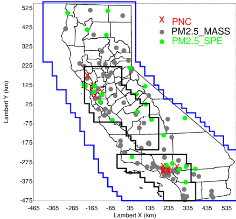
Figure 224: Modeling domains. Blue lines outline the CA_24 km domain, black lines outline the SoCAB_4 km (bottom) and SJV_4 km domains (top). Red crosses represent ten particle number concentration (PNC) x sites (four sites operated by staff at the Bay Area Air Quality Management District (BAAQMD) and six sites from the Multiple Air 210 Toxics Exposure Study IV (MATES IV) ). Detailed location information for the PNC x sites is listed in Table S3. Green dots represent BAAQMD PM 2.5 speciation network sites and the Interagency Monitoring of Protected Visual Environments (IMPROVE) sites; gray dots represent the PM 2.5 federal reference method (FRM) sites.
