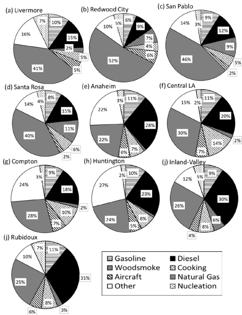
Figure 14-44: The relative source contributions to PM 0.1 seasonally averaged at Livermore, Redwood City, San Pablo and Santa Rosa, Anaheim, Central LA, Compton, 610 Huntington, Inland-Valley and Rubidoux, respectively. Averaging time included all days shown in Figures 10-12 127-9. Values not displayed are \leq 1\% .
