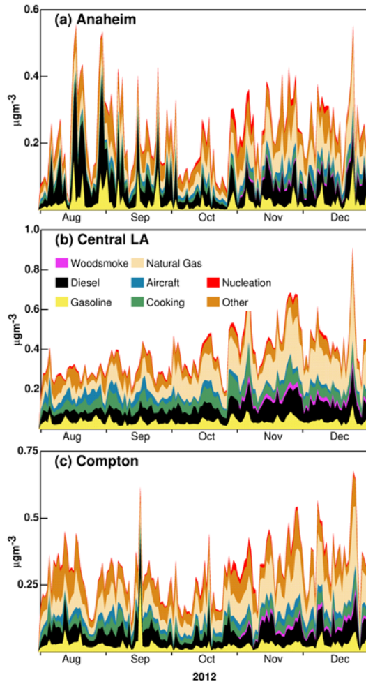
Figure 11118: Seasonal variation of major source contributions to PM 0.1 at Anaheim, Central LA, and Compton, respectively. Results within each month have daily time resolution.
