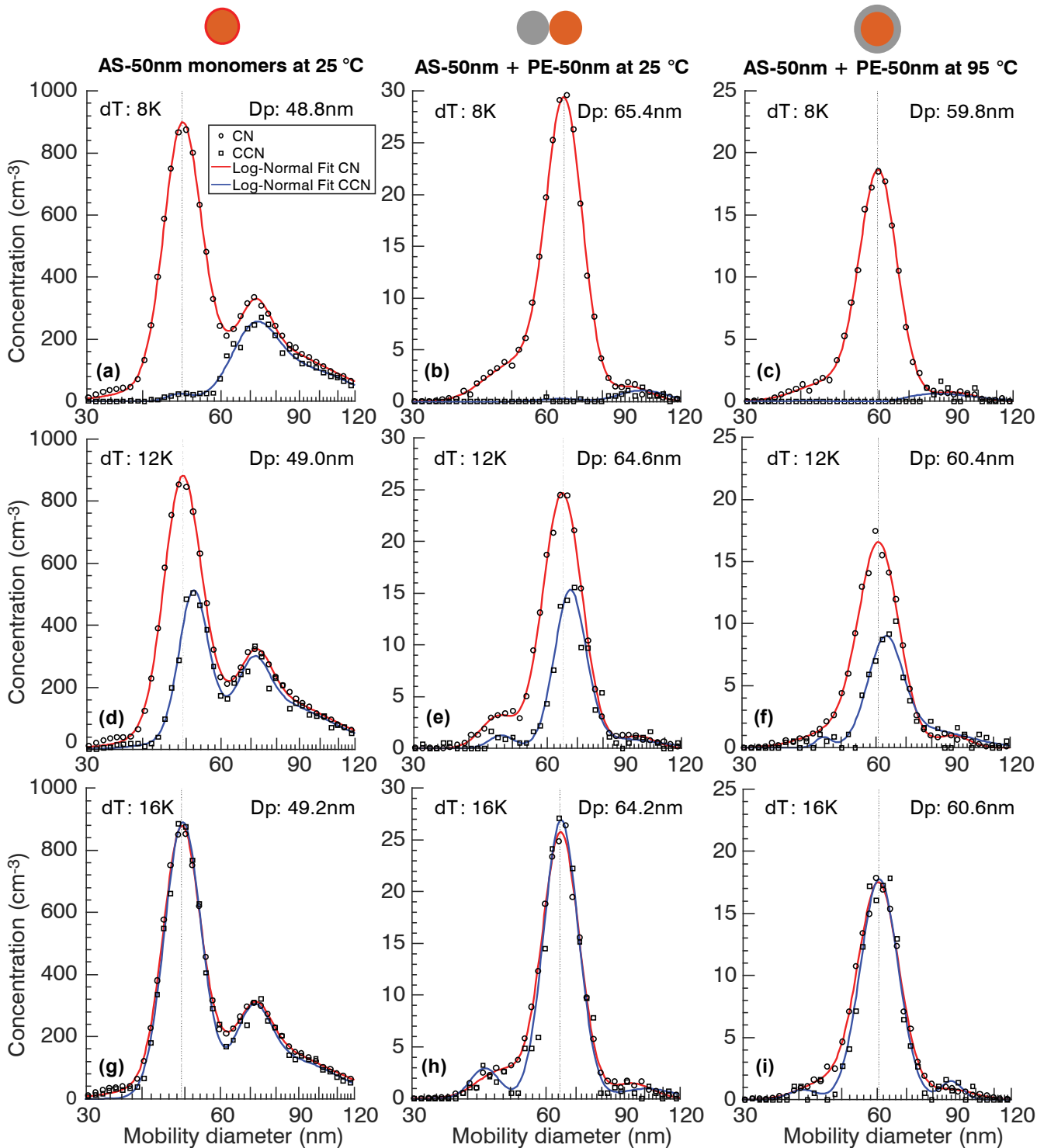
665 Figure 3: CN and CCN size-distributions at three different CCNc column temperature gradients corresponding to water supersaturations measured after the thermal conditioning of particles.
