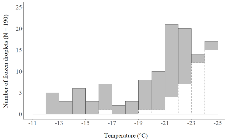
5 Figure 2. Number of planar, branched ice crystals that re-froze on a cold-stage after having been molten (grey bars with solid contour), thereby confirming they contained an INP active within the respective 1 °C temperature step. Of 190 crystals analysed, 24 re-froze at -17 °C or warmer (INP -17 ). The white bars with dashed contour indicate the number of frozen control droplets. The total number of control droplets was 190 as well.
