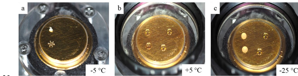
Figure 1. Illustration of one ice crystal droplet freezing experiment. Transparent droplets are liquid. (a) Two single crystals on the cold-stage (note: the cold-stage was set to below 0 °C for this image and the upper crystal is not a dendrite). (b) Melted ice crystals with addition of 3 \mu L ultrapure water to increase the detection volume (left) and two 3 \mu L control droplets of the same ultrapure water (right). (c) The frozen sample (left) and supercooled control (right) droplets after cooling to -25 °C.
