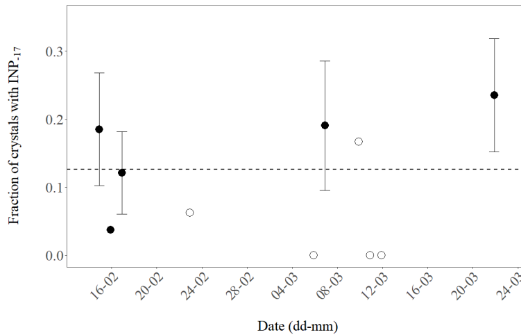
10 Figure 3. Daily fraction of ice crystals with INPs active at -17 °C or warmer (INP -17 ) observed for 10 days during February and March 2018. The number of crystals analysed per day was between 21 and 34 (closed symbols) or less (3 to 16, open symbols). Error bars indicate an estimate of the standard deviation (proportional to \sqrt{\text{INP}_{-17}} ) for days when at least four crystals with INP -17 were found. The dashed line shows the mean value of the pooled data (190 analysed crystals).
