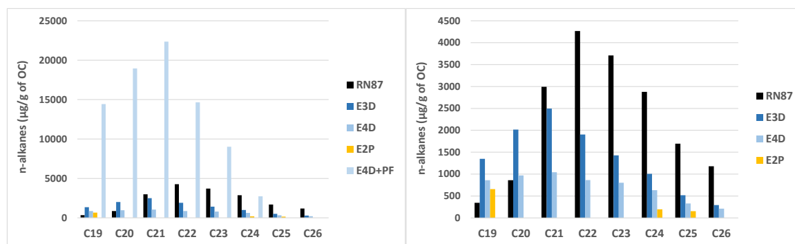
Figure 5: n-alkanes emissions normalized by OC emissions at the traffic site (RN87/E712) and from the exhaust of a Diesel Euro 3 vehicle (E3D), a Diesel Euro 4 vehicle (E4D), a Diesel Euro 4 vehicle equipped with a particle filter (E4D+PF) (on the left only) and a Euro 2 Petrol vehicles.
