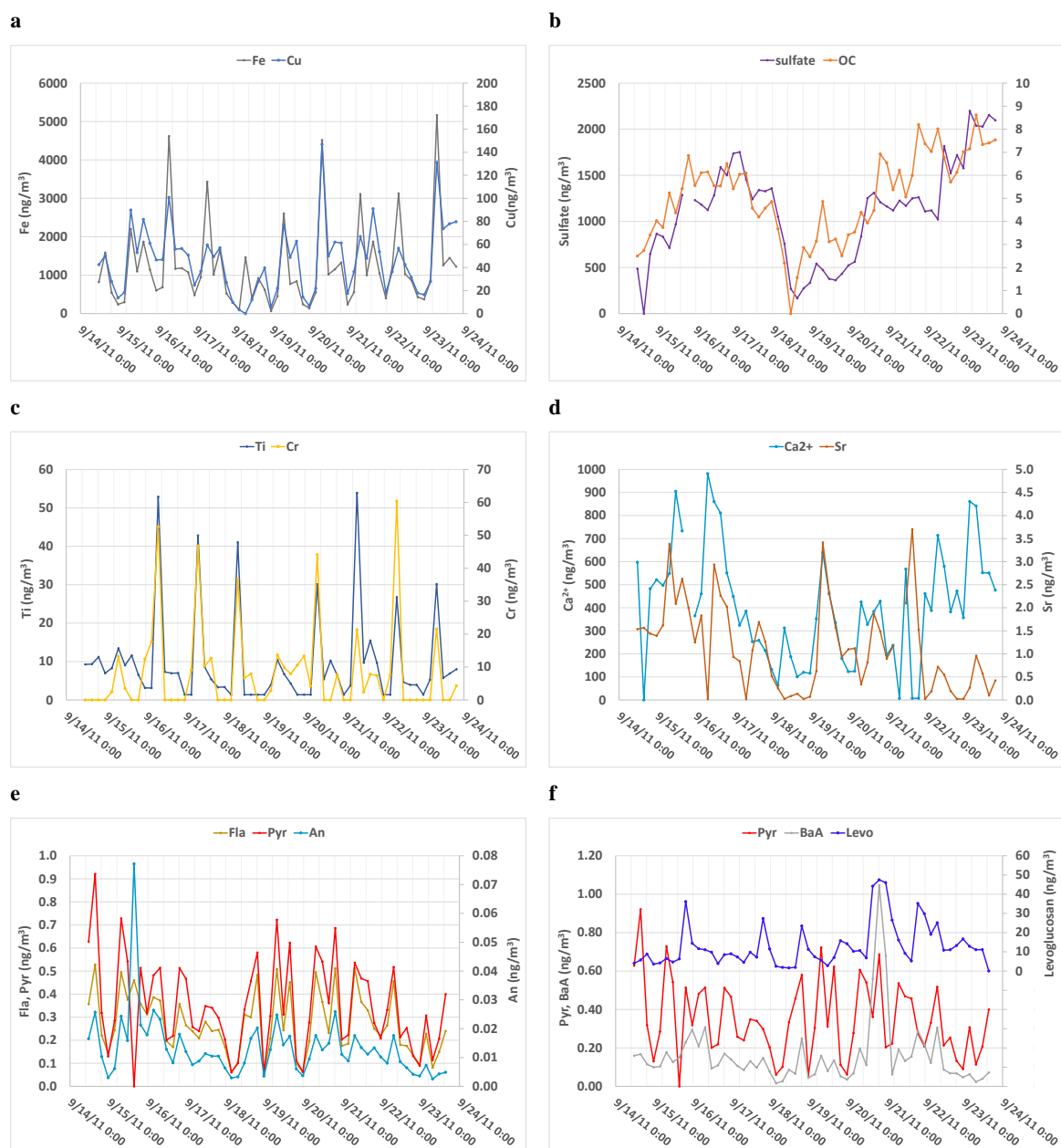
Figure 2: 4-hour concentrations measured at the traffic site: a: iron and copper; b: sulfate and organic carbon; c: chromium and titanium; d: calcium and strontium; e: fluoranthene, pyrene and anthracene; f: pyrene, benzo(a)anthracene and levoglucosan.
