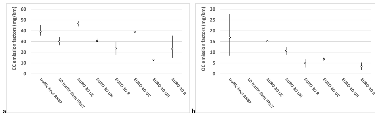
Figure 4: Emission factors for EC (a) and OC (b) for the mixed traffic fleet and the light duty traffic of the RN87/E712 freeway and from the chassis dynamometer measurements of exhaust emissions of EURO 3 and EURO 4 vehicles for respectively urban cold (UC), urban hot (UH) and road (R) driving cycles. The emission factor for OC for the LD traffic fleet could not be determined and no data available for the hot driving conditions for the Euro 4 diesel vehicles.
