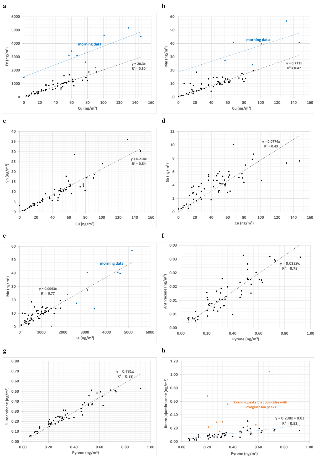
Figure 3 : Scatterplots and linear relationships for a few species : a : iron vs. copper ; b : manganese vs. copper ; c : tin vs. copper ; d : antimony vs. copper ; e : manganese vs. iron ; f : anthracene vs. Pyrene ; g : fluoranthene vs. Pyrene ; h : benzo(a)anthracene vs. pyrene
