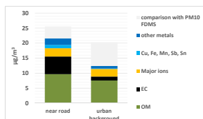
Figure 2. Median concentrations measured at the roadside site (Echirolles) and urban background site (Les Fâmes) and comparison with respective median TEOM-FDMS PM 10 concentrations. OM is computed using the factor 1.8 estimated for Grenoble city (Favez et al., 2010).
