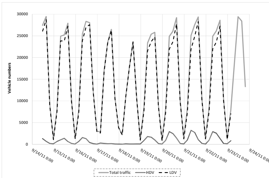
Figure III-2 : Total, light-duty, and heavy-duty vehicle counts during the sampling period from double electromagnetic loops
