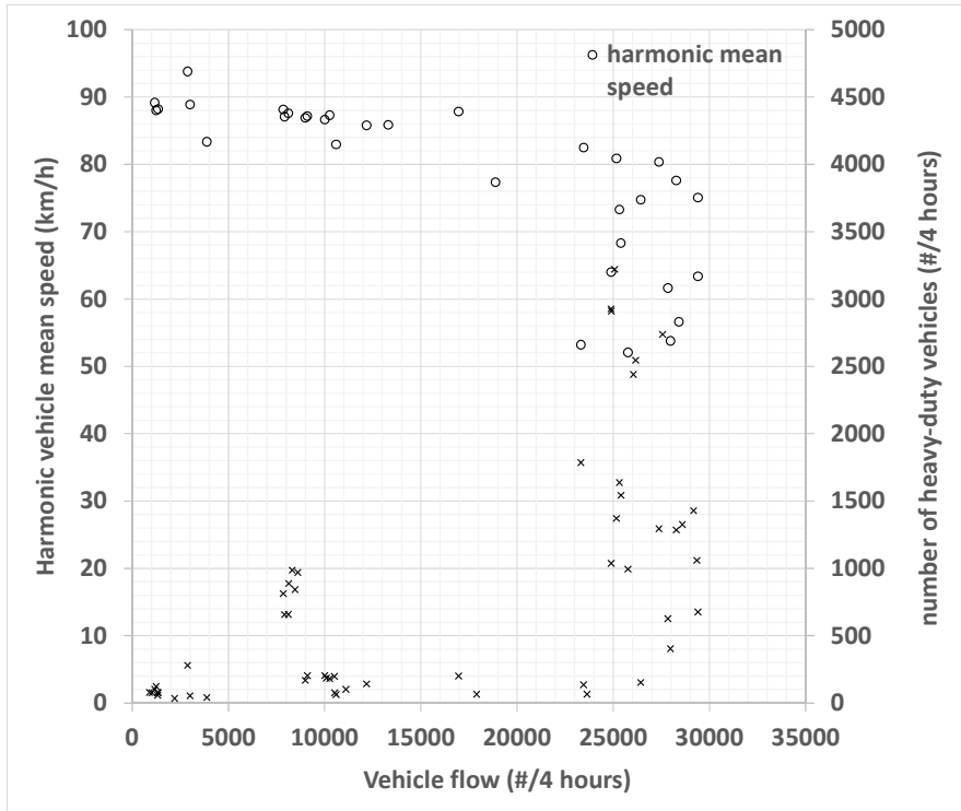
Figure III-1: Harmonic vehicle mean speed (km/h) and number of heavy-duty vehicles versus the vehicle flow per period of 4 hours (corresponding to the sampling periods)
