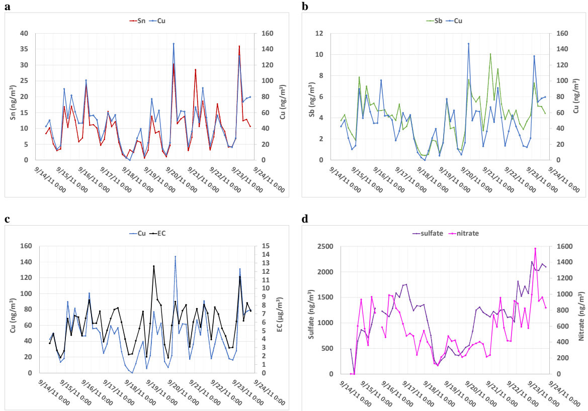
Figure VII-1: 4-hour concentrations measured at the traffic site: a: copper and tin; b: copper and antimony; c: copper and elemental carbon; d: sulfate and nitrate
