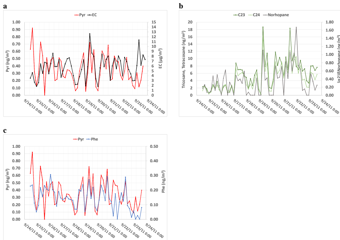
e Figure VII-2: 4-hour concentrations measured at the traffic site: a: elemental carbon and pyrene; b: tricosane, tetracosane and 17α21βNorhopane; c: pyrene and phenanthrene
