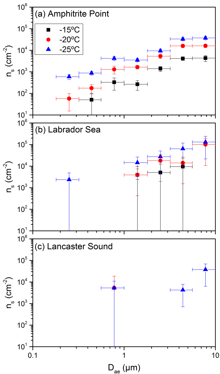
Figure 6. Surface active site density, n_s , as a function of aerodynamic diameter ( D_{ae} ) at -15 °C, -20 °C, and -25 °C, respectively. The plotted x-values represent the midpoints of the size bins from the MOUDI. The x-errors represent the widths of the size bins, and the y-errors are the propagated uncertainties from INP concentrations as a function of size (Fig. 3) and aerosol surface area concentrations as a function of size (Fig. S4b). In some cases, the y-error bars are smaller than the size of the symbols.
