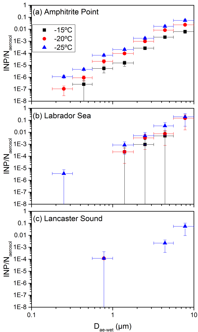
Figure 5. The fraction of aerosol particles acting as an INP ( INP/N_{aerosol} ) plotted as a function of aerodynamic diameter ( D_{ae} ) at -15 °C, -20 °C, and -25 °C, respectively, where N_{aerosol} is the number of aerosol particles in a given size bin. The plotted x-values represent the midpoints of the size bins from the MOUDI. The x-error bars represent the widths of the size bins, and the y-error bars are the propagated uncertainties from INP concentrations as a function of size (Fig. 3) and aerosol number concentrations as a function of size (Fig. S4a). In some cases, the y-error bars are smaller than the size of the symbols.
