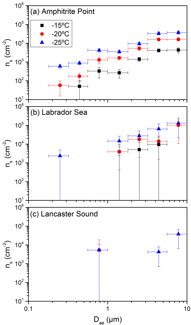
Figure 6. Surface active site density, n_s , as a function of aerodynamic diameter ( D_{ae} ) at -15 °C, -20 °C, and -25 °C, respectively. The x-errors represent the widths of the size bins, and the y-errors are the propagated uncertainties from INP concentrations as a function of size (Fig. 3) and aerosol surface area concentrations as a function of size (Fig. S4b). In some cases, the y-error bars are smaller than the size of the symbols.
