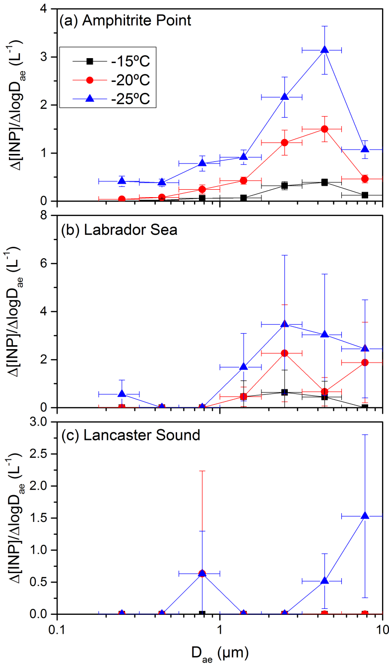
Figure 3. Average INP number concentrations at freezing temperatures of -15 ^{\circ}\text{C} , -20 ^{\circ}\text{C} , and -25 ^{\circ}\text{C} as a function of aerodynamic diameter ( D_{ae} ) for the three sites studied. The x-error bars represent the widths of the size bins from the MOUDI. For the Amphitrite Point samples, standard error of the mean was used to represent the uncertainty of INP concentrations during the month. At both Labrador Sea and Lancaster Sound, only one MOUDI sample was collected, and we assume the monthly INP concentrations have the same normal distribution as the Amphitrite Point samples. Hence for the y-error bars at these locations, we assume the relative standard deviation for supermicron and submicron particles were the same as the relative standard deviation for supermicron and submicron particles observed in the Amphitrite Point data.
