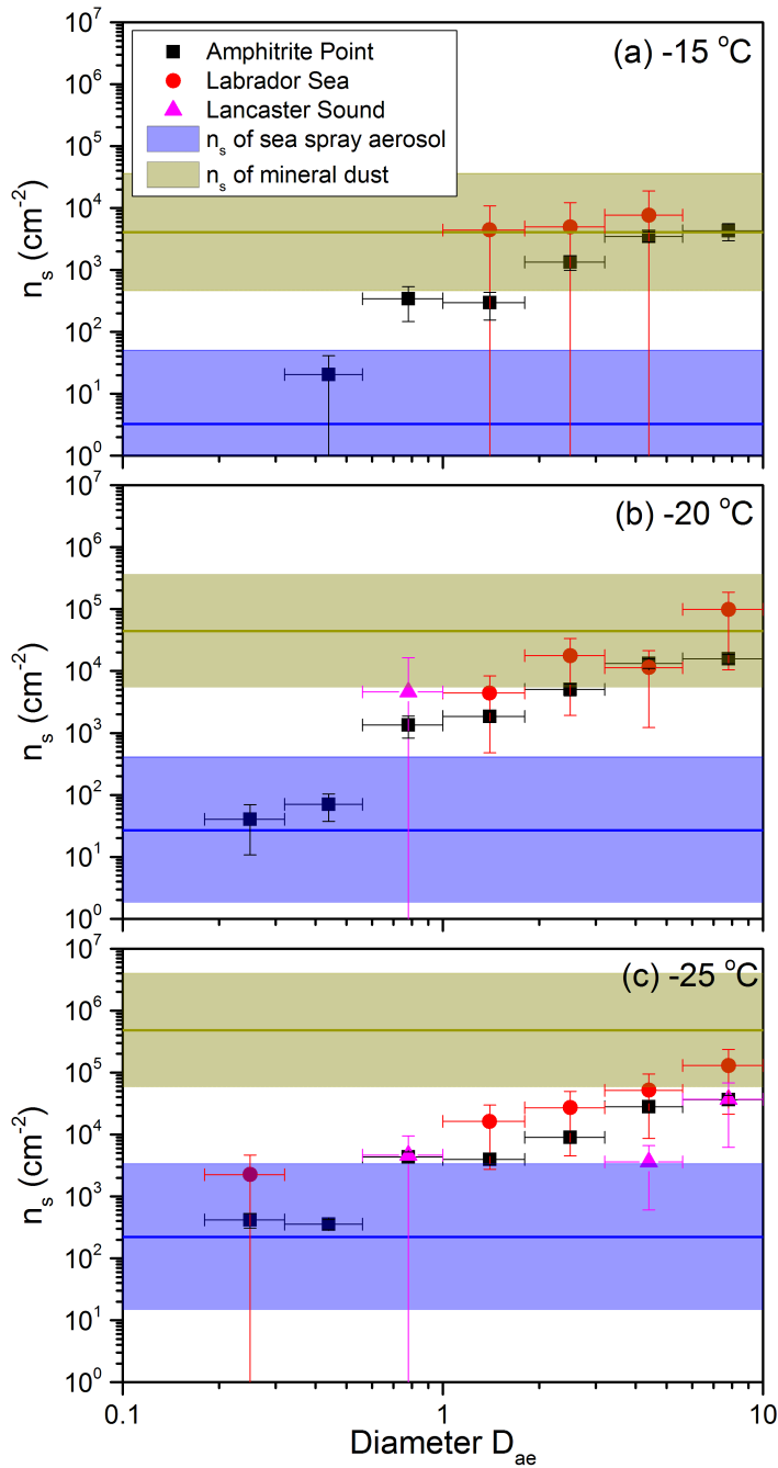
Figure 7. Comparison of measured n_s values with previously reported n_s values of sea spray aerosol and mineral dust at -15\text{ }^\circ\text{C} , -20\text{ }^\circ\text{C} , and -25\text{ }^\circ\text{C} , respectively. The n_s values of sea spray aerosol were taken from DeMott et al. (2016), and the n_s values of mineral dust were taken from Niemand et al. (2012). The horizontal lines represent the calculated n_s values from linear regression, and the coloured bands represent the 95 % prediction bands (see Fig. S5-S6 in the Supplement). Blue represents sea spray aerosol, and light green represents mineral dust.
