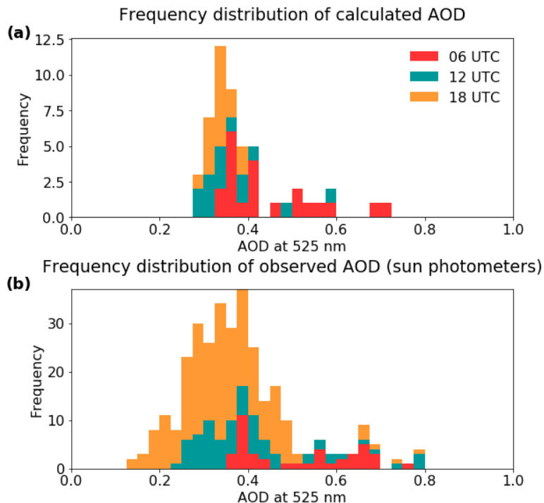
Figure 10. The frequency distributions of calculated AODs from radiosonde RHs, and AODs observed by sun photometers over Savé during the DACCIIWA campaign. Bars shown here are stacked. Values have not been calculated for 00 UTC as this is during the night.
