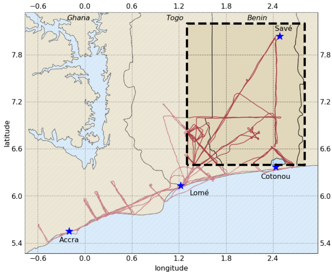
Figure 1. Map of the Twin Otter flight paths. The box represents locations where data was used in this analysis to compare with radiosonde data from the Savé supersite.
