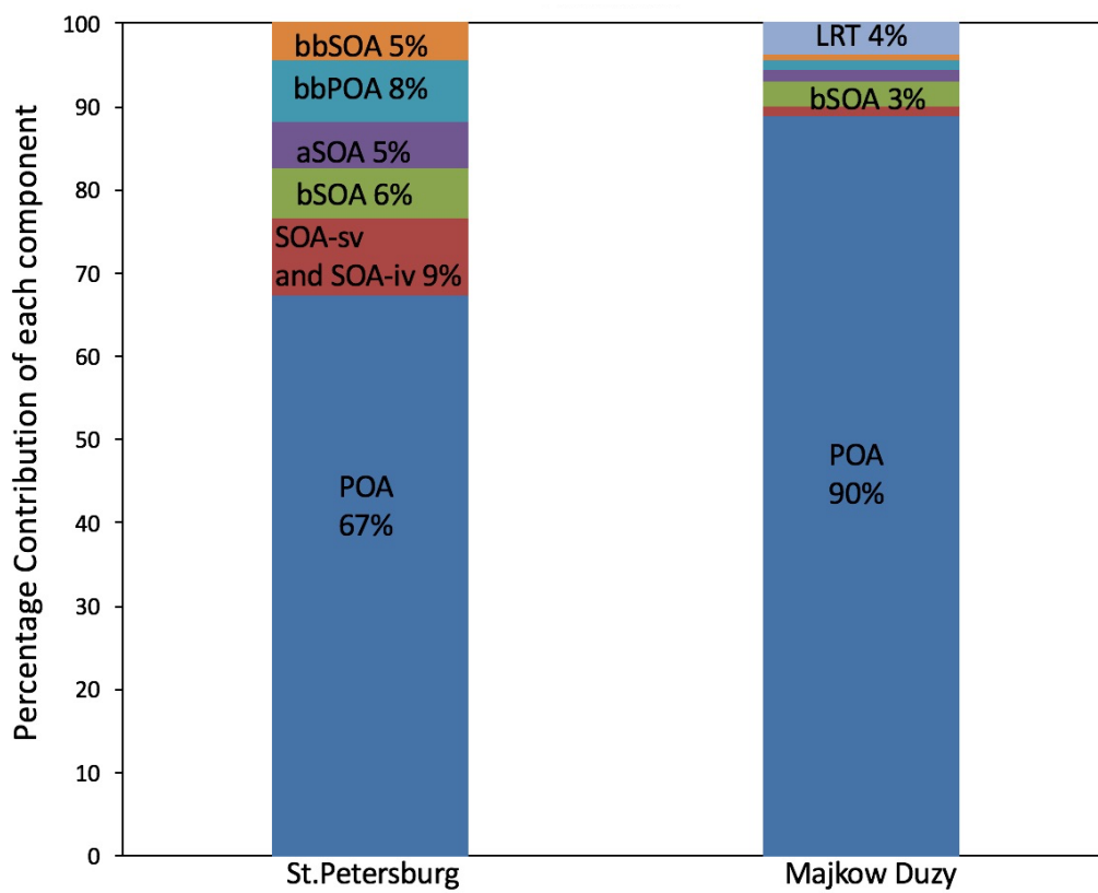
880 Figure 5. Contribution of each OA component to the PMCAM x -SR PMF POA factor in St. Petersburg (Russia) and Majkow Duzy (Poland) during May 2008.
