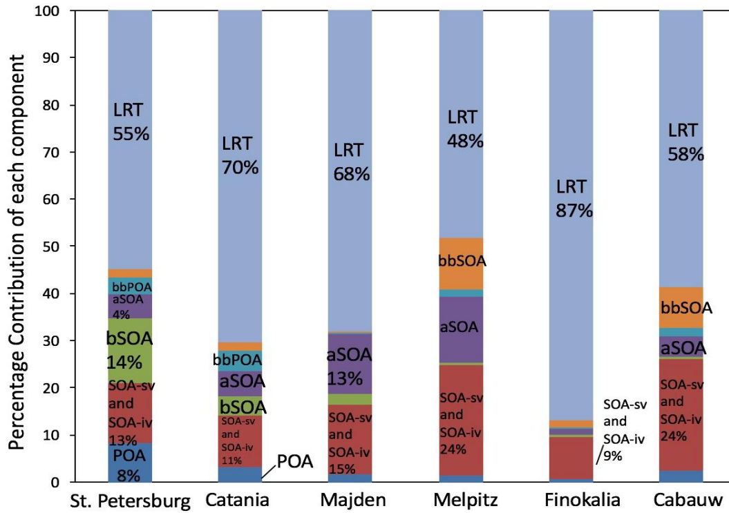
Figure 7. Contribution of each OA component to PMCAM x -SR LRT factor in St. Petersburg, Catania, Majden, Melpitz and Finokalia during May 2008.
