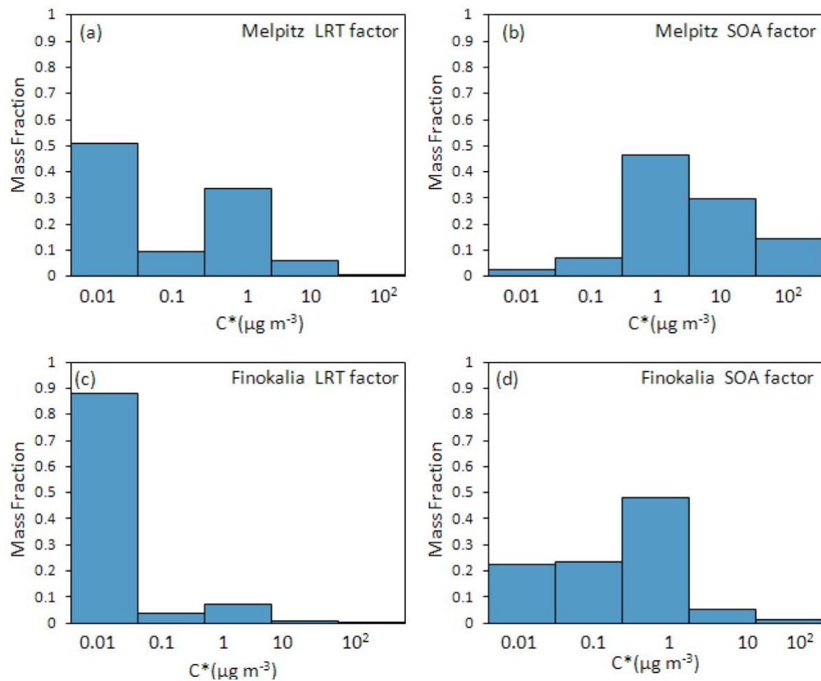
Figure 9. Volatility distribution of the: (a) LRT factor in Melpitz, (b) SOA factor in Melpitz, (c) LRT factor in Finokalia, and (d) SOA factor in Finokalia.
