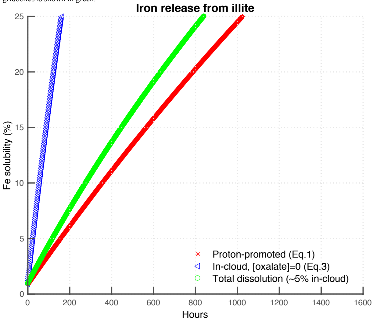
Figure S4: Percent iron solubility from medium soluble iron ( Fe_{med} ) at pH = 2 , T=298 °K (for comparison with Figure S2 from Ito and Shi, 2016). Proton-promoted dissolution applied at all model gridboxes is calculated from Eq. (1) and is shown in red. The iron liberation from in-cloud, organic ligand processing at [C_2O_4^{2-}] = 0 is shown in blue and is only applied in the cloud-fraction of gridboxes within clouds given by Eq. (3). The total iron dissolution for ~ 5% in-cloud to all atmosphere gridboxes is shown in green.
