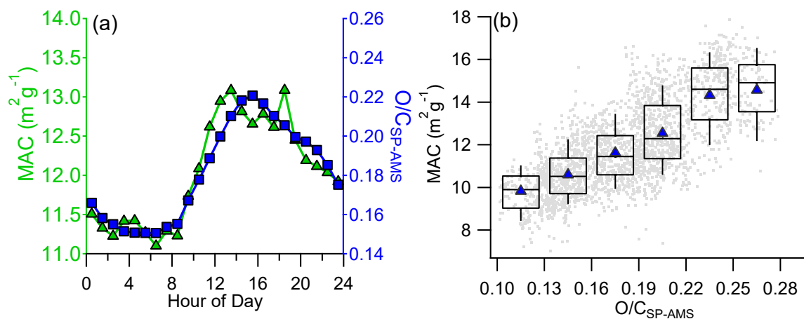
Figure 10. (a) Diurnal cycles of MAC and O/C ratio of SP-AMS, and (b) variations of MAC as a function of O/C SP-AMS . The data are binned according to O/C. The median (horizontal line), mean (triangle), 25 th and 75 th percentiles (lower and upper box), and 10 th and 90 th percentiles (lower and upper whiskers) are also shown.
