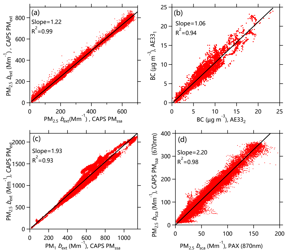
Figure 1. Inter-comparisons of aerosol optical properties and BC: (a) b_{\text{ext}} of \text{PM}_{2.5} from CAPS \text{PM}_{\text{ext}} and CAPS \text{PM}_{\text{ssa}} , (b) BC from two AE33s, (c) b_{\text{ext}} of \text{PM}_{2.5} from CAPS \text{PM}_{\text{ext}} vs. b_{\text{ext}} of \text{PM}_1 from CAPS \text{PM}_{\text{ssa}} , (d) b_{\text{sca}} from CAPS \text{PM}_{\text{ssa}} vs. b_{\text{sca}} from PAX.
