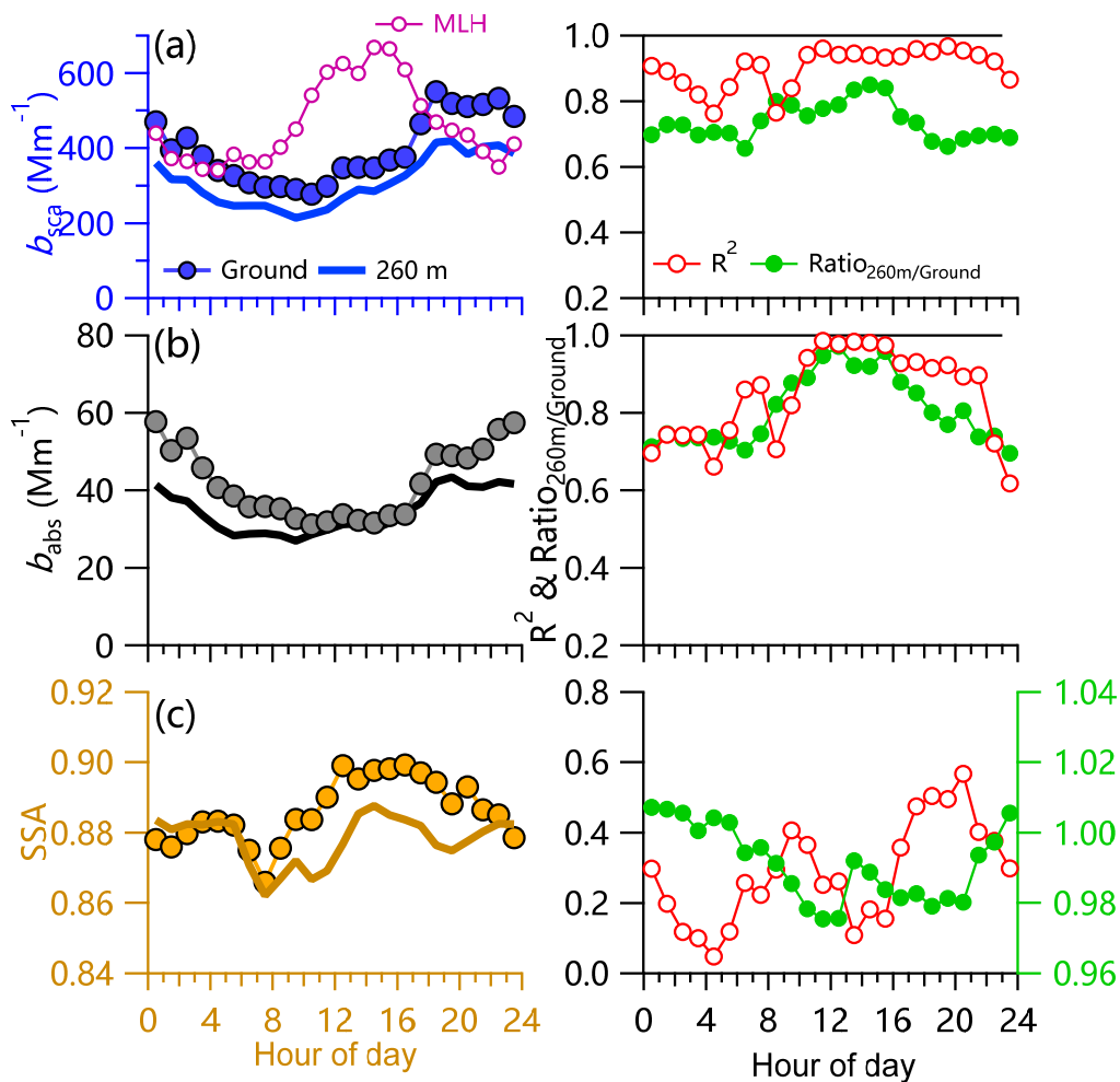
Figure 6. Diurnal cycles of (a) b_{\text{sca}} , (b) b_{\text{abs}} , and (c) SSA at 260 m and ground level for the entire study. Right panel shows the diurnal cycles of correlation coefficients ( R^2 ) and \text{ratio}_{260\text{m}/\text{ground}} for b_{\text{sca}} , b_{\text{abs}} , and SSA. Note that the diurnal cycles above excluded 5 periods with cleaning processes (November 19 1:00 to 9:00, November 26 1:00 to 12:00, November 26 19:00 to November 27 3:00, December 3 20:00 to December 4 16:00, and December 17 00:00 to 12:00) while those of entire study are shown in Fig. S3.
