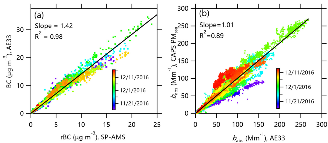
Figure 2. Comparisons of (a) BC measurements between AE33 and SP-AMS, (b) b_{\text{abs}} calculated from the difference of b_{\text{ext}} and b_{\text{sca}} of CAPS \text{PM}_{\text{ssa}} and that was derived from BC.
