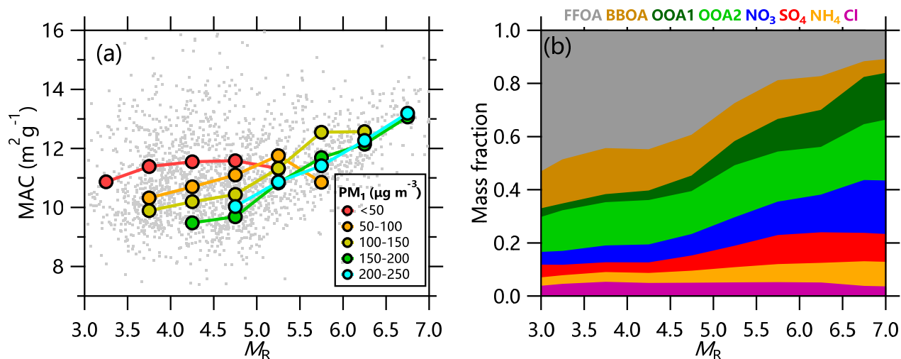
Figure 9. (a) Variations of mass absorption cross-section (MAC) as a function of M_R at different pollution levels and (b) variations of mass fraction of rBC-coated species as a function of M_R .
