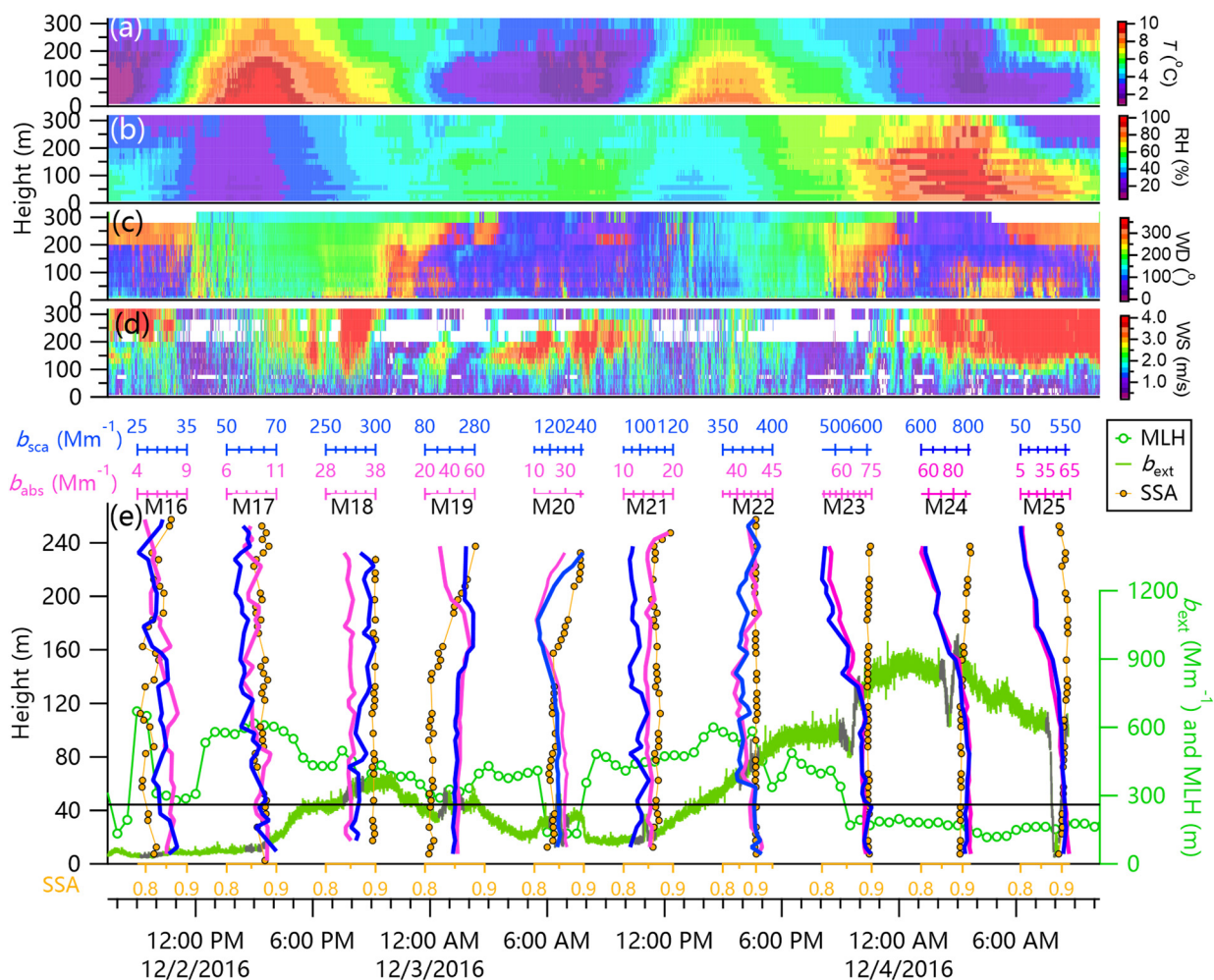
Figure 7. Evolution of vertical profiles of b_{sca} , b_{abs} and SSA during 2 – 4 December. Also shown are (a-d) meteorological variable of T , RH, WD, and WS, and (e) time series of b_{ext} at ground and MLH. M16-M25 refer to the number of vertical profiles.
