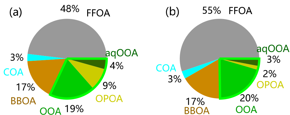
Figure 12. Average contributions of OA sources to BrC absorption at ground level from (a) linear regression model analysis, and (b) positive matrix factorization (Fig. S8). The sources of OA include fossil fuel-related OA (FFOA), cooking OA (COA), biomass burning OA (BBOA), oxygenated OA (OOA), oxidized primary OA (OPOA), aqueous-phase OOA (aq-OOA) (Xu et al. 2018).
