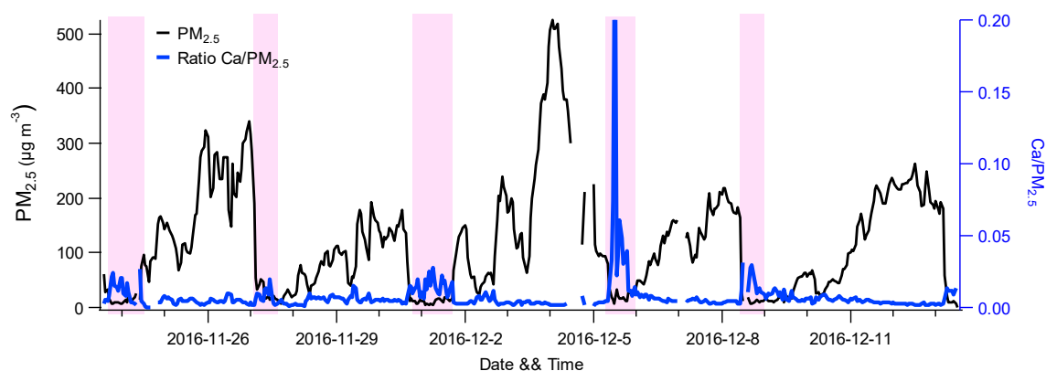
Figure S2. Time series of \text{PM}_{2.5} and Ca content during this study. The periods with high Ca/ \text{PM}_{2.5} (shaded areas) are excluded when calculating the absorption and AAE of BrC.
