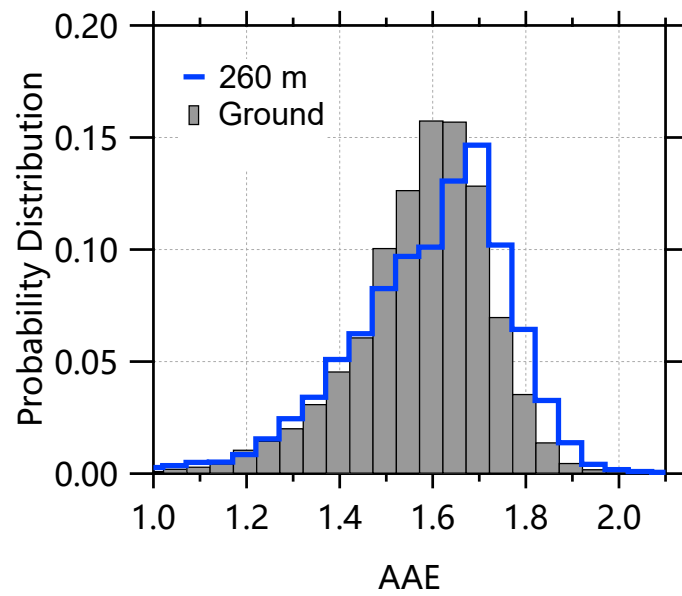
Figure S7. Probability distribution of absorption angstrom exponent (AAE) at ground level and at 260 m.
