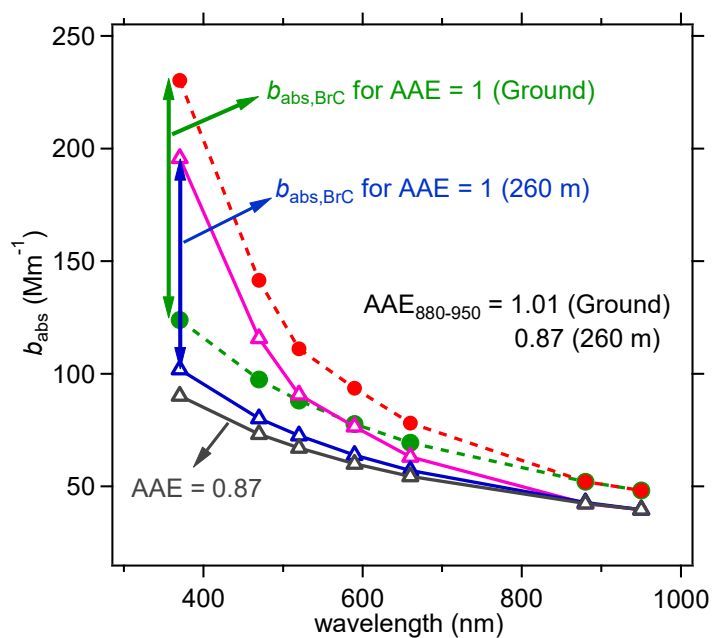
Figure S1. Measured b_{\text{abs}} at ground (red dots) and 260 m (pink triangles) as a function of wavelengths. Estimation of b_{\text{abs}} for pure BC are also shown with the assumption that AAE equal to 1 and values derived from b_{\text{abs}} at 880 and 950 nm.
