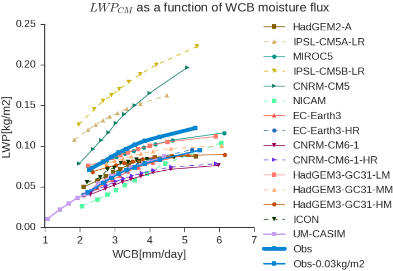
Fig. 1 Cyclone-mean LWP (LWP CM ) as a function of WCB moisture flux in models and observations. LWP CM is shown averaged into 9 equal quantiles for the observations and each GCM. The maximum bias in the observations (~0.03kg/m2) is shown as a lighter blue line.
