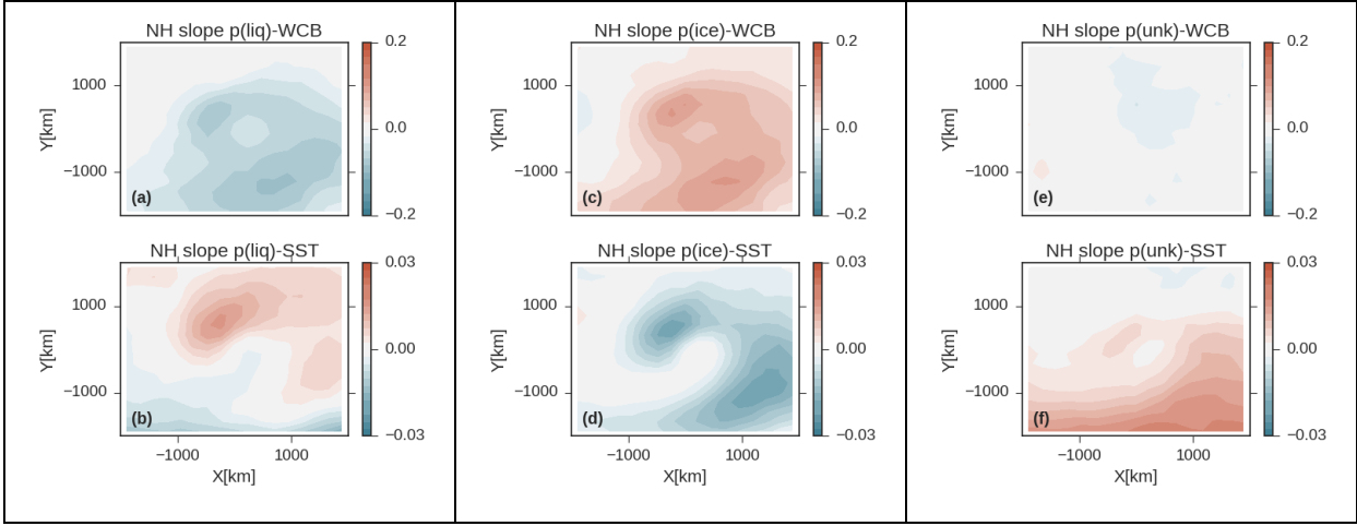
Fig. 11 The coefficients in the multiple linear regression relating the probability of liquid, ice, and unknown cloud top phase to WCB moisture flux (units are day \text{mm}^{-1} ) into the cyclone and \text{SST}_{ij} within the cyclone (units are \text{K}^{-1} , Eq. 6). All data is from the NH. (a and b) relate to the probability of liquid topped clouds, (c and d) relate to ice-topped clouds, and (e and f) to unknown phase. Note that all probabilities are the probability of detecting a specific phase, given that a phase detection has been made. The first row shows the coefficient relating WCB moisture flux into the cyclone to cloud top phase probability. The second row shows the coefficient between \text{SST}_{ij} and cloud top phase.
