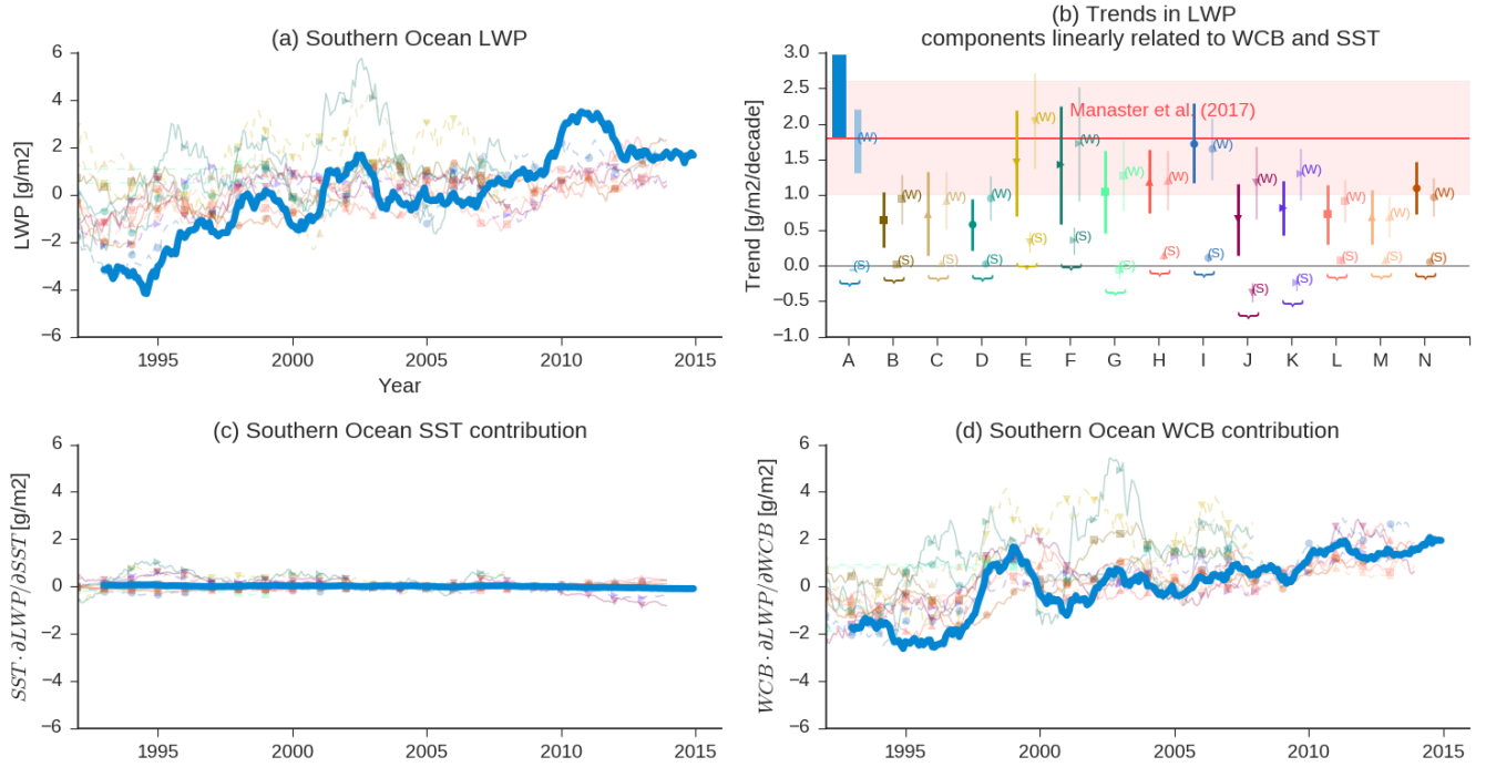
Fig. 4 (a) SH cyclone LWP_{RM} in observations (thick blue line) and models (colors as in Fig. 1) where cyclones are centered between 44.5°S and 59.5°S. A 2-year running mean has been applied to simplify the plot. (b) The red shaded area shows the zonal-mean Southern Ocean LWP trend calculated in Manaster et al. (2017) (Southern Ocean defined as 44.5°S-59.5°S therein). Trends in cyclone LWP_{RM} from observations and models are shown in dark colors (where LWP_{RM} is calculated using cyclones centered in the same region as Manaster et al. (2017)). Models and observations are labelled by a letter on the ordinate (see Table 2). Observations are labelled as 'A'. The 95% confidence in each trend is shown using errorbars. A multiple linear regression of LWP_{CM} on SST_{CM} and WCB moisture flux is used to partition the trend into contributions from WCB and SST changes. The trend in LWP_{RM} predicted by the regression model (Eq. 4) and changes in SST_{RM} is shown in (c), and the trend in LWP_{RM} associated with WCB is shown in (d). The trend from models and observations consistent with their multiple linear regression models and changes in SST_{RM} and WCB is shown in (b) using lighter colors and labelled as (S) for SST, and (W) for WCB.
