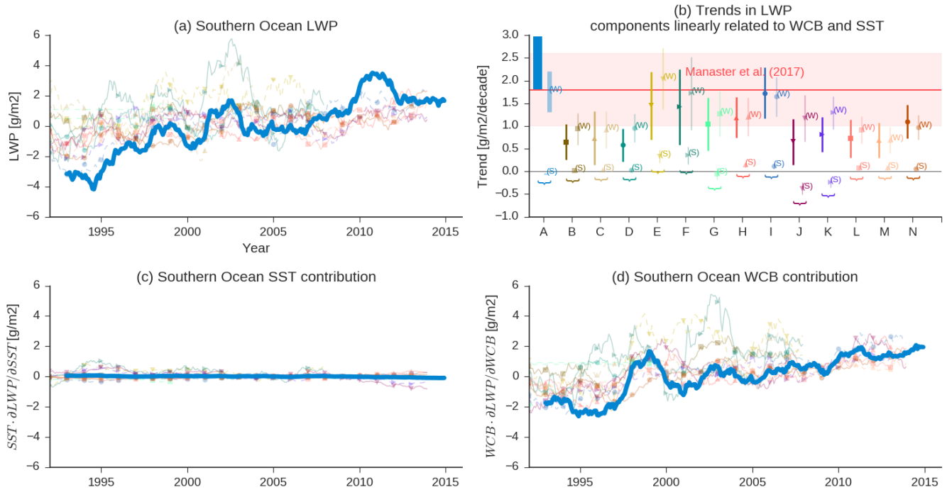
Fig. 4 (a) SH cyclone LWP_{RM} in observations (thick blue line) and models (colors as in Fig. 1 ) where cyclones are centered between 44.5^{\circ}S and 59.5^{\circ}S . A 2-year running mean has been applied to simplify the plot. (b) The red shaded area shows the zonal-mean Southern Ocean LWP trend calculated in Manaster et al. (2017) (Southern Ocean defined as 44.5^{\circ}S - 59.5^{\circ}S therein). Trends in cyclone LWP_{RM} from observations and models are shown in dark colors (where LWP_{RM} is calculated using cyclones centered in the same region as Manaster et al. (2017)). Models and observations are labelled by a letter on the ordinate (see Table 2 ). Observations are labelled as 'A'. The 95% confidence in each trend is shown using errorbars. A multiple linear regression of LWP_{CM} on SST_{CM} and WCB moisture flux is used to partition the trend into contributions from WCB and SST changes. The trend in LWP_{RM} predicted by the regression model (Eq. 4) and changes in SST_{RM} is shown in (c), and the trend in LWP_{RM} associated with WCB is shown in (d). The trend from models and observations consistent with their multiple linear regression models and changes in SST_{RM} and WCB is shown in (b) using lighter colors and labelled as (S) for SST, and (W) for WCB.
