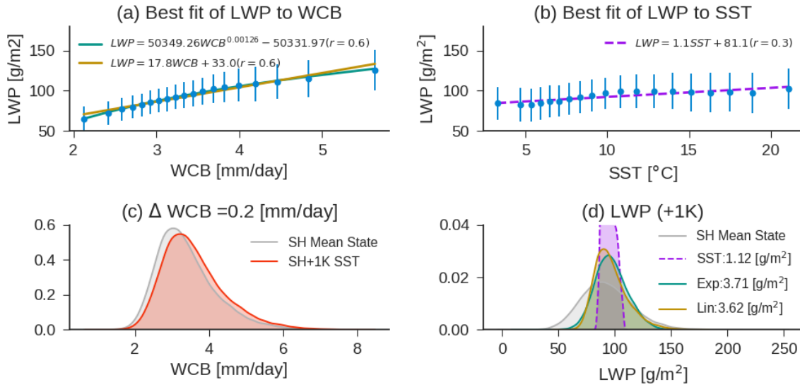
Fig. 6 (a) The LWP_{CM} observed in SH as a function of WCB moisture flux, the best fit line to the observations using the form LWP_{CM} = a \cdot WCB^b + c is shown using a green line. A simple linear fit is shown in yellow. The observations are binned into equal quantiles for visual clarity. Errorbars show a standard deviation within each bin. (b) the fit of cyclone LWP_{CM} to SST_{CM} . (c) The distribution of SH WCB moisture flux in the current climate, and when WVP moisture flux is scaled by 1.06 consistent with a uniform 1K increase in SST. The difference in WCB moisture flux is noted in the title. (d) The distribution of LWP_{CM} in the current climate and as predicted by the fits shown in (a) and (b). The LWP_{CM} when SST is increased by 1K as predicted by the fits in (a) is based on scaling WVP by 1.06. The wh LWP_{CM} predicted by the fit shown in (b) is based on SST increasing uniformly by 1K. The mean difference between LWP_{CM} between the prediction and the climate mean state is noted in the legend.
