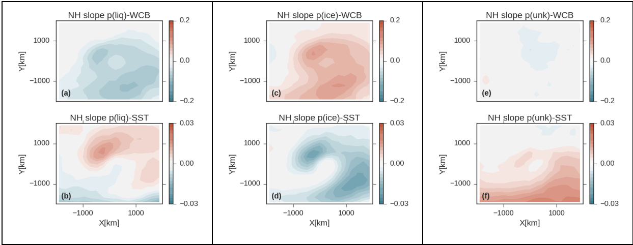
Fig. 11 as in Fig. 11, but showing the coefficients in the multiple linear regression relating the probability of liquid, ice, and unknown cloud top phase to WCB moisture flux (units are \text{day mm}^{-1} ) into the cyclone and \text{SST}_{ij} within the cyclone (units are \text{K}^{-1} , Eq. 6). All data is from the NH. (a and b) relate to the probability of liquid topped clouds, (c and d) relate to ice-topped clouds, and (e and f) to unknown phase. Note that all probabilities are the probability of detecting a specific phase, given that a phase detection has been made. The first row shows the coefficient relating WCB moisture flux into the cyclone to cloud top phase probability. The second row shows the coefficient between \text{SST}_{ij} and cloud top phase.
