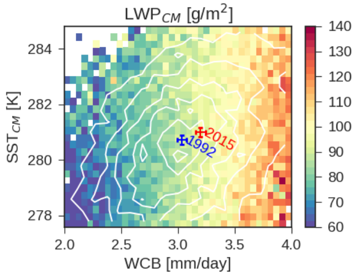
Fig. 5 Average Southern Ocean cyclone LWP CM binned as a function of SST CM and WCB moisture flux for the latitude band 44.5°S to 59.5°S, following Manaster et al. (2017). Contours of cyclone distribution are shown in white. The mean cyclone WCB moisture flux and SST CM for 1992 and 2015 are shown as blue and red points, respectively. Errorbars show the 95% confidence on the mean.
