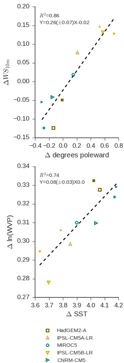
Fig. 9 Changes in cyclone-mean wind speed at 10m ( WS_{10m} ) and the natural log of WVP between AMIP and AMIP+4K simulations plotted against changes in mean poleward cyclone latitude and SST, respectively. Open symbols show the change over the NH and closed symbols show the change over the SH. The best fit line to NH and SH is noted in each plot along with 95% confidence in the slope.
