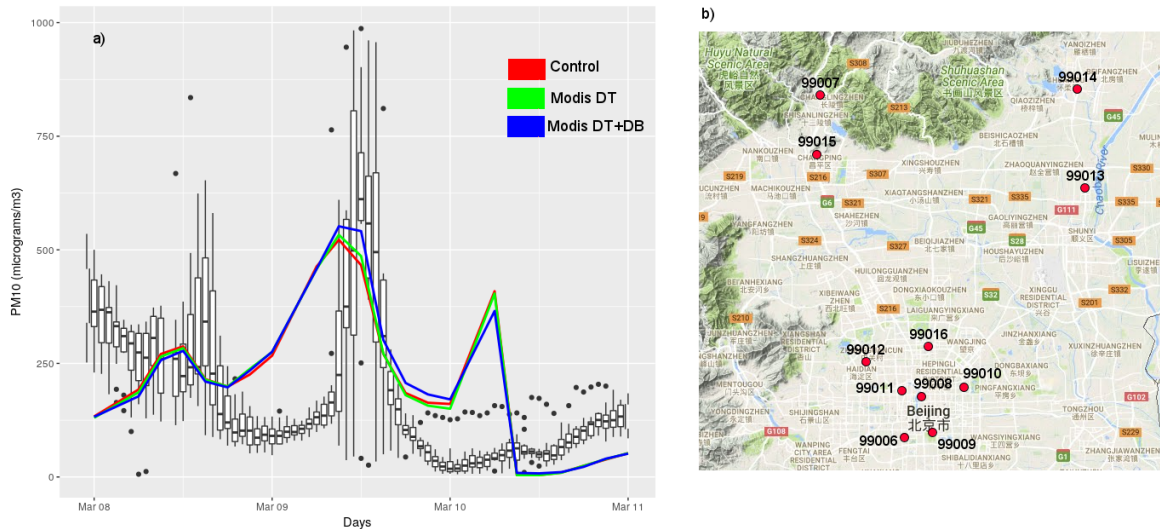
Figure 10. a) March 2013 PM10 time series for the measurements recorded in the 11 stations available in the Beijing municipality and the simulations performed with the ECMWF model in the different configurations (CONTROL in red; DT in green and DTDB in blue). b) location and identification code of the observation stations around the Beijing area.
