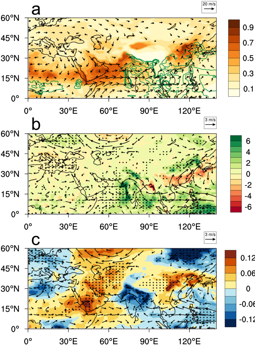
560 Figure 3. (a) Spatial distributions of climatological AOD during July to August, superimposed with precipitation (only those >6 mm day -1 are shown) and 850 hPa wind (arrows, in m s -1 ) (b) Spatial distributions of anomalous ('strong' minus 'weak') precipitation (mm day -1 ) and 850 hPa wind (arrows, in m s -1 ). (c) is same as (b) except the patter is showing anomalous AOD and 850 hPa wind (arrows, in m s -1 ). Dots represent data points with a significance > 95%.
