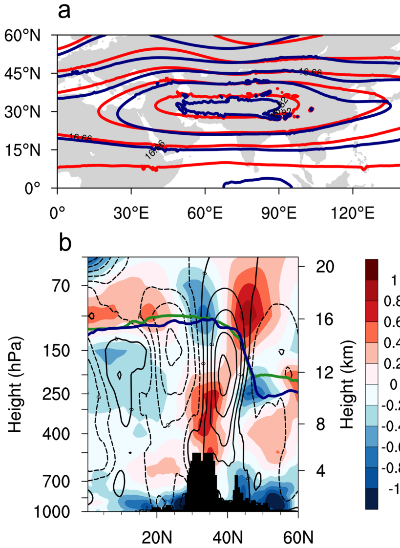
Figure 2. (a) 100-hPa Geopotential height (in km) in strong (weak) monsoon years during July-August is shown in red (blue). (b) Latitude-height cross-section of temperature anomalies (color shaded, in K), zonal wind anomalies (contour lines, in m s -1 ) between strong and weak monsoon years ('strong' minus 'weak'), and tropopause height (thick lines) in strong monsoon years (green) and weak monsoon years (blue) over the Indian subcontinent (80°E-85°E) during July-August.
