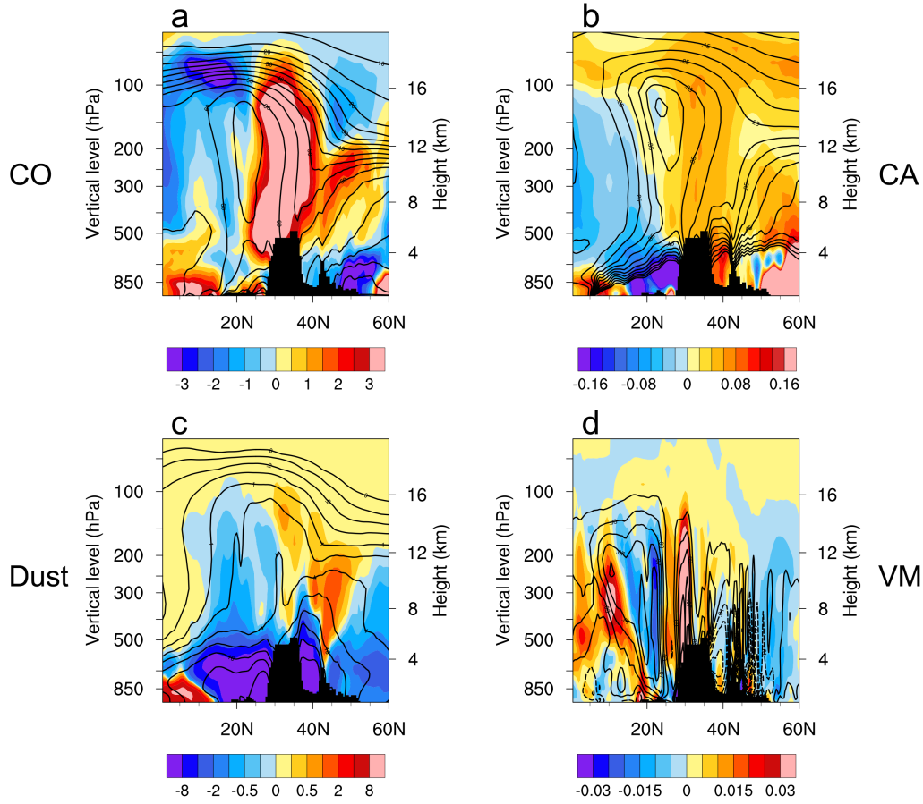
605 Figure 6. Latitude-height cross-sections (0°N-60°N) of (a) CO (ppbv), (b) CA (ppbm), (c) dust (ppbm), and (d) vertical motion ( \text{Pa s}^{-1} ) anomalies between strong and weak monsoon years ('strong' minus 'weak') averaged over the HGP region (80°E-85°E) during July-August, superimposed with the climatological mean of weak monsoon years (black contours). For vertical motions in (d), solid (dashed) contours indicating ascent (descent).
