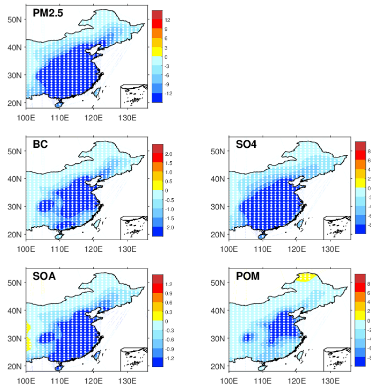
Figure 2. Simulated linear trends of the total PM 2.5 surface concentration as well as
