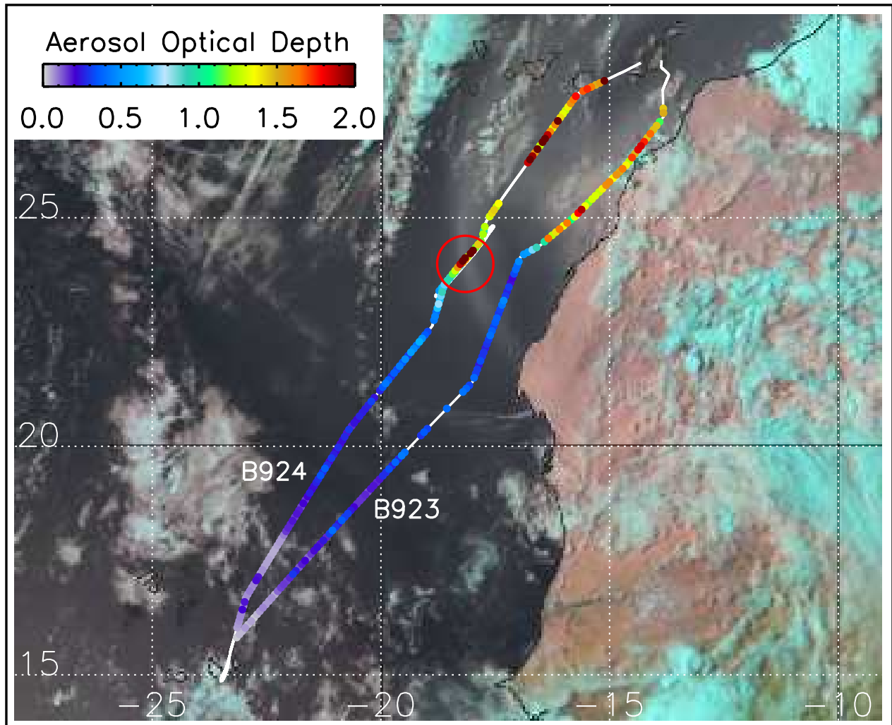
Figure 3. Meteosat Second Generation “321 RGB” image for 12 August at 16:30UTC, showing the extent of the dust plume advected off the West coast of Africa. The track of flights B923 and B924 is overplotted. A colour scale depicts the lidar-derived AOD, and a red circle indicates the location where the aircraft descended to sample the heavy dust in situ. A SLR at 30 m altitude was performed between 15:52 and 16:04UTC (run 4), and a SLR at 1,000 m took place between 16:09 and 16:29UTC (run 5).
