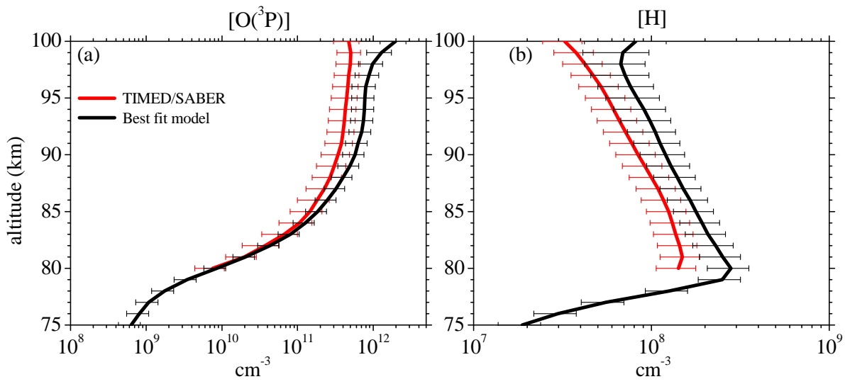
Figure 6 : Vertical profiles of a) [O(^3P)] and b) [H] derived from SABER OH(9-7)+OH(8-6) VER observations (Mlynczak et al., 2018) and our Best fit model by fitting SABER OH(9-7)+OH(8-6) VER and OH(5-3)+OH(4-2) VER as well as SCIAMACHY OH(6-2) VER and OH(3-1) VER. Shown are averages of night-time mean zonal means of co-location measurements (see Sect. 2.2) from 2003 to 2011 between 0^\circ and 10^\circ N. Error bars show the 1\sigma uncertainty due to chemical and physical processes.
