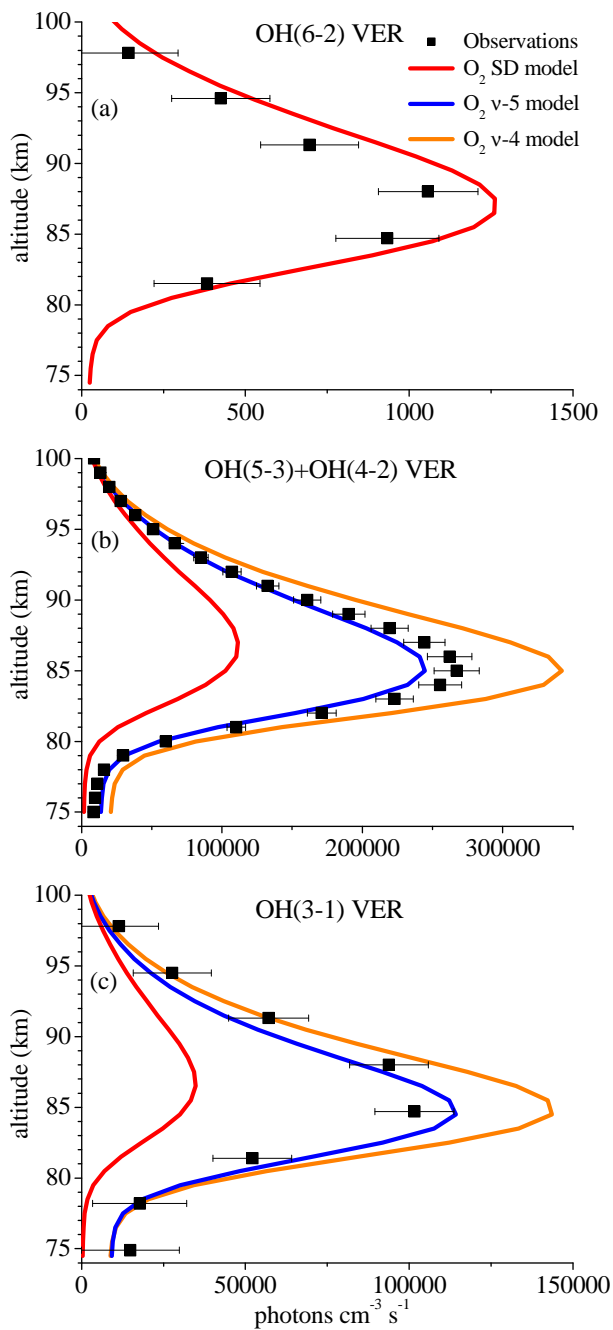
Figure 3 : Same as Fig. 1 but for the O 2 SD model, the O 2 v-5 model, and the O 2 v-4 model. Note that the results of these three models are identical in case of OH(6-2) VER.
