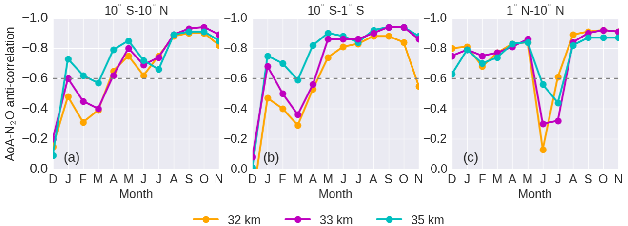
Figure 10. \text{N}_2\text{O} -AoA anti-correlation as a function of month averaged for the period January 2004–April 2012 for (a) 10^\circ\text{S} - 10^\circ\text{N} , (b) 10^\circ\text{S} - 1^\circ\text{S} , and (c) 1^\circ\text{N} - 10^\circ\text{N} . Colour coding indicates altitude: 32 km (orange), 33 km (magenta), and 35 km (cyan). The dashed horizontal lines indicate an arbitrary threshold of moderate correlation, which was selected to be the value of -0.6.
