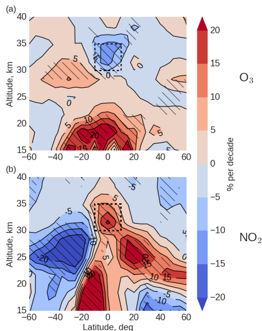
Figure 2. Latitude-altitude distribution of (a) O_3 and (b) NO_2 changes (% per decade) from MLR applied to SCIAMACHY measurements for the January 2004–April 2012 period. Hatched areas show changes significant at the 2\sigma level. The dashed rectangle indicates the region of the tropical mid-stratosphere investigated in this paper.
