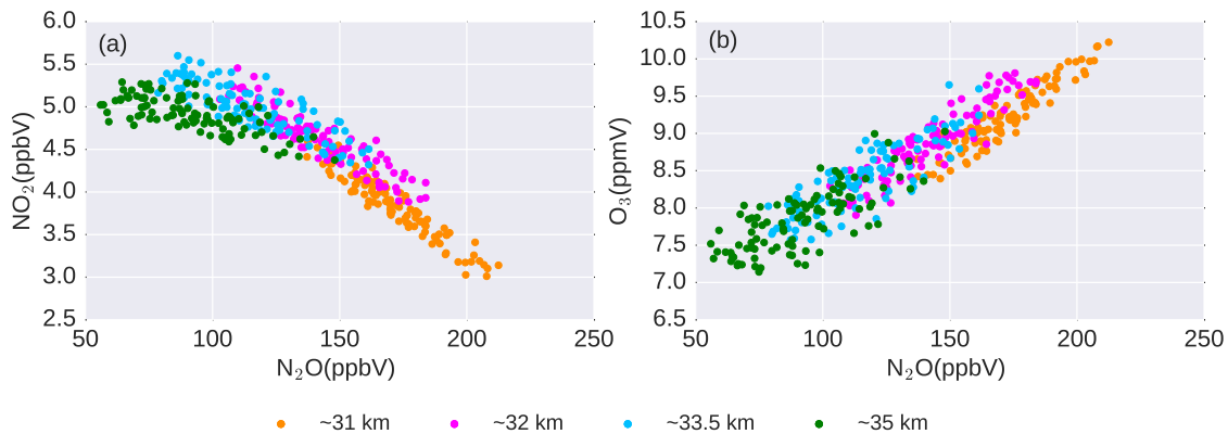
Figure 4. Scatter plots of monthly mean (a) N_2O versus NO_2 and (b) N_2O versus O_3 in the tropical mid-stratosphere during January 2004–April 2012 from TOMCAT simulation CNTL. Colour coding classifies data according to altitude: 31 km (orange), 32 km (magenta), 33.5 km (sky blue), and 35 km (green).
