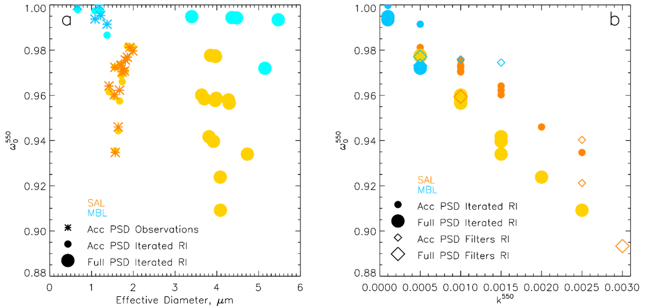
5 Figure 13: Contribution to single scattering albedo from particle size (a: SSA vs d_{\text{eff}} ) and from composition (b: SSA vs k^{550} ), separated by SLRs in the SAL (orange and yellow) and MBL (blue). Small data points represent the ACC PSD only, large data points represent the FULL PSD. Asterixes in (a) are direct observations behind inlets. Circles represent calculations using the RI derived from Mie iterations; diamonds represent calculations using RI derived from composition data from filter samples assuming internal mixing (4 samples). For the FULL PSD with the iterated RI, the same accumulation mode RI is extended to the coarse mode. For the filters RI, size-specific RI is used for the accumulation mode and the full PSD (as given in Table 7).
