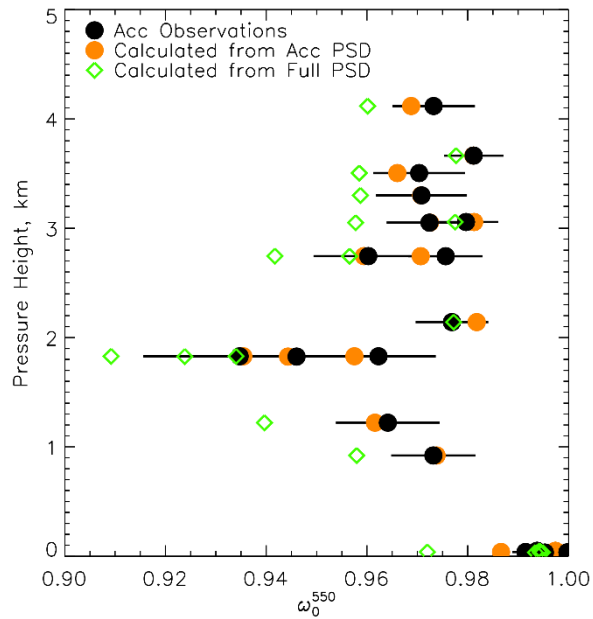
5 Figure 12: Variation of SSA at 550nm with altitude for SLRs. Black circles indicate direct measurements taken in-cabin behind inlets and therefore represent the accumulation mode (ACC PSD) only. Orange circles indicate calculated properties, representative of the same conditions in-cabin behind inlets for the ACC PSD. Green diamonds indicate values calculated using the 2DS-XY FULL PSD covering size ranges 0.1 to 200 \mu\text{m} . Green and orange data points are from Mie calculations, black represents measurements.
