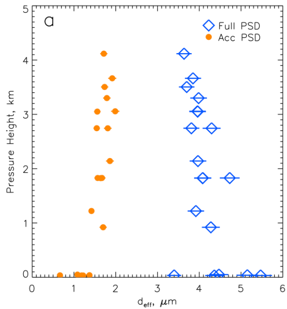
Figure 8: Variation of size with altitude for SLRs: (a) effective diameter; (b) maximum diameter measured by the 2DS XY instrument. Orange circles represent accumulation mode only, blue diamonds represent the full PSD.
