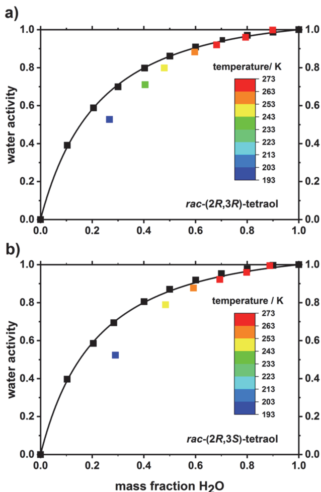
Figure 3. Measured water activity of mixtures of (a) rac -(2R,3R)-tetraol with water and (b) rac -(2R,3S)-tetraol with water at 298.15 K (black squares) and at their ice melting points (colored squares). The curves are fits to the data: for details see main text.
