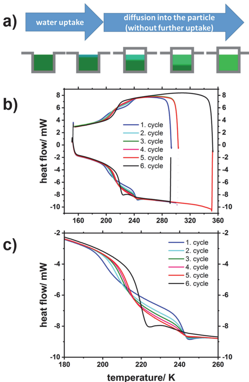
5 Figure 7. (a) Illustration of water uptake by a hygroscopic substance and subsequent water diffusion within it for a sample inside a DSC sample pan. (b/c) DSC thermograms showing several consecutive cooling/heating cycles of wetted rac-(2R,3R)-tetraol (b), with a close-up view of the glass transition region (c). After each of the first 4 cycles the temperature was held constant at 303.15 K for 20 minutes before the next cycle was initiated. After the 5 th cycle the temperature was raised to 353.15 K and held constant for 20 minutes before the last 6 th cycle was initiated.
