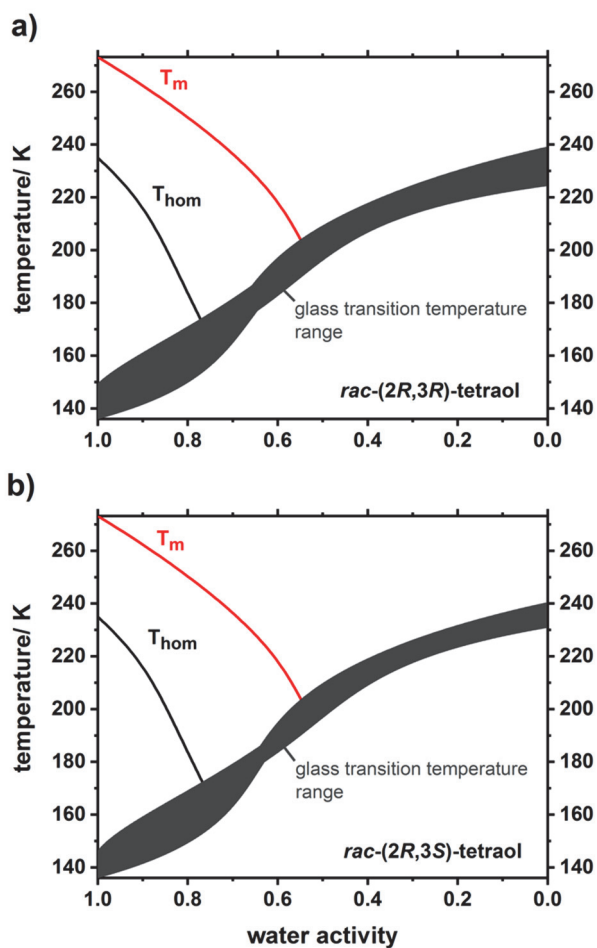
5 Figure 4. Partial phase diagrams of mixtures of rac -(2R,3R)-tetraol with water (a) and rac -(2R,3S)-tetraol with water (b) plotted as a function of water activity. In addition to the ice melting point line ( T_m ; red line) the homogeneous ice nucleation temperatures ( T_{hom} ; black line) are shown. The dark grey area indicates the glass transition temperatures and their uncertainty; see text for details.
