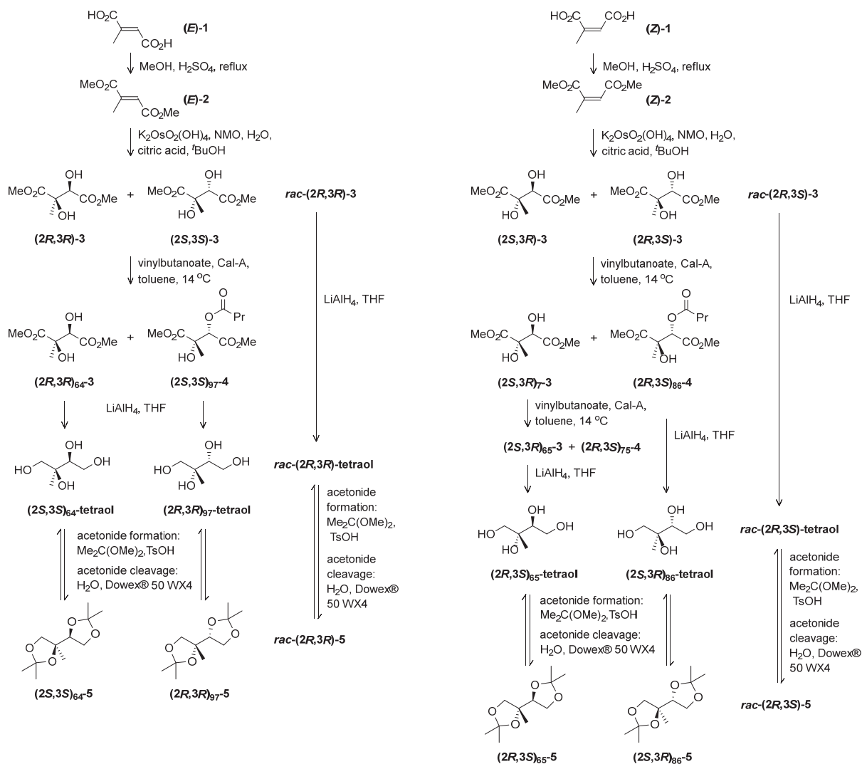
Scheme 1: Synthesis of the racemic and enantiomerically enriched tetraols. NMO indicates N-methylmorpholine-N-oxide. The reaction was performed at room temperature, if no other temperature is given in the scheme.
