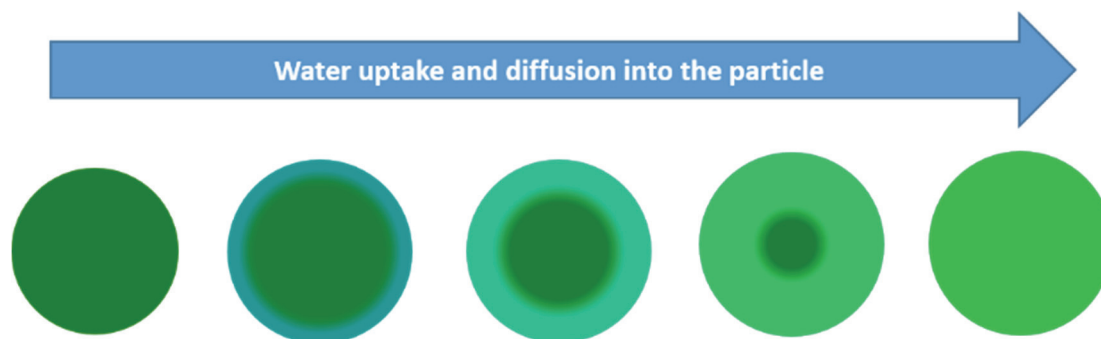
25 Figure 5. Schematics of water uptake and diffusion into an aerosol particle with a sharp transition line distinguishing two homogeneous domains during diffusion: the dark green organic core and the light green organic/water shell.
