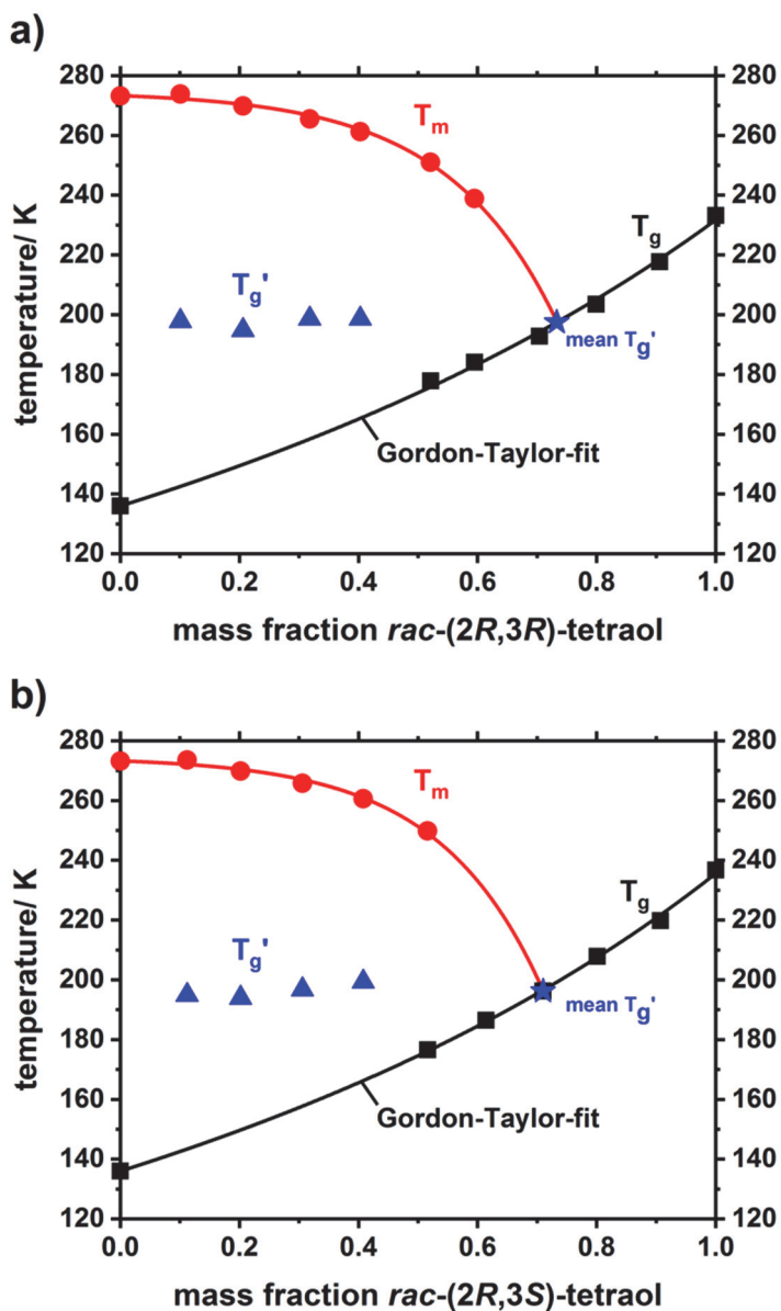
5 Figure 2. Partial phase diagram of mixtures of rac -(2R,3R)-tetraol with water (a) and rac -(2R,3S)-tetraol with water (b). Shown are the ice melting temperatures T_m (red circles), glass transition temperatures T_g (black squares) and maximally freeze-concentrated glass transition temperatures T_g' (blue triangles). The melting temperatures are fitted with an exponential function and the glass transition temperatures are fitted with the Gordon-Taylor equation yielding a Gordon-Taylor constant of k_{GT} = 1.53 \pm 0.08 (a) and k_{GT} = 1.58 \pm 0.05 (b), respectively. The T_g' values are plotted at the overall mass fraction of the solution before cooling. The composition of the amorphous fraction of a sample after the water partly crystallized is depicted as the mean T_g' shifted towards the Gordon-Taylor fit (blue star).
