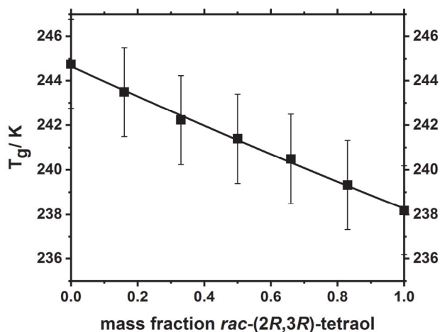
Figure 1. Glass transition temperatures of mixtures of rac -(2 R ,3 S )-tetraol and rac -(2 R ,3 R )-tetraol. The T_g values show a nearly linear relationship with a Gordon-Taylor constant k_{GT} of 0.92.
