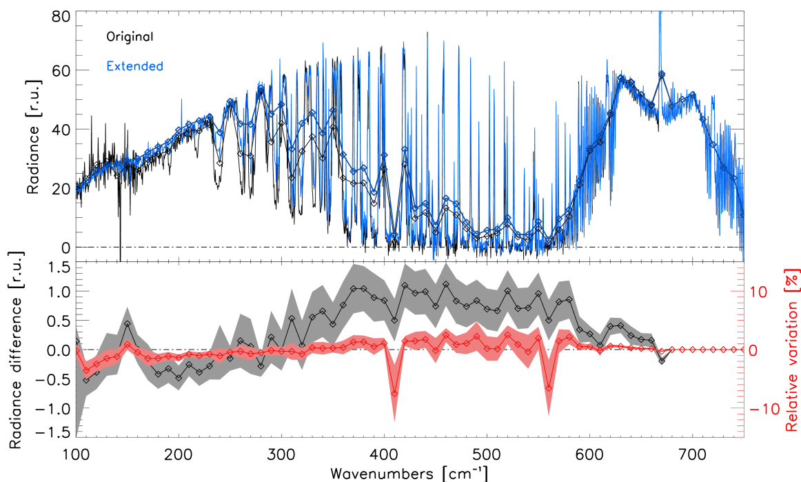
Figure 4. Far-infrared extension based on REFIR-PAD data. (a) Example of a spectrum (black) and its extension (blue) below 667\text{ cm}^{-1} . The same spectra integrated over 10\text{ cm}^{-1} bands are also shown by the diamond lines. (b) Mean difference (black) and relative variation (red) between the original and the extended spectra at 10\text{ cm}^{-1} resolution calculated over the entire test set. Shaded areas are the associated standard errors.
