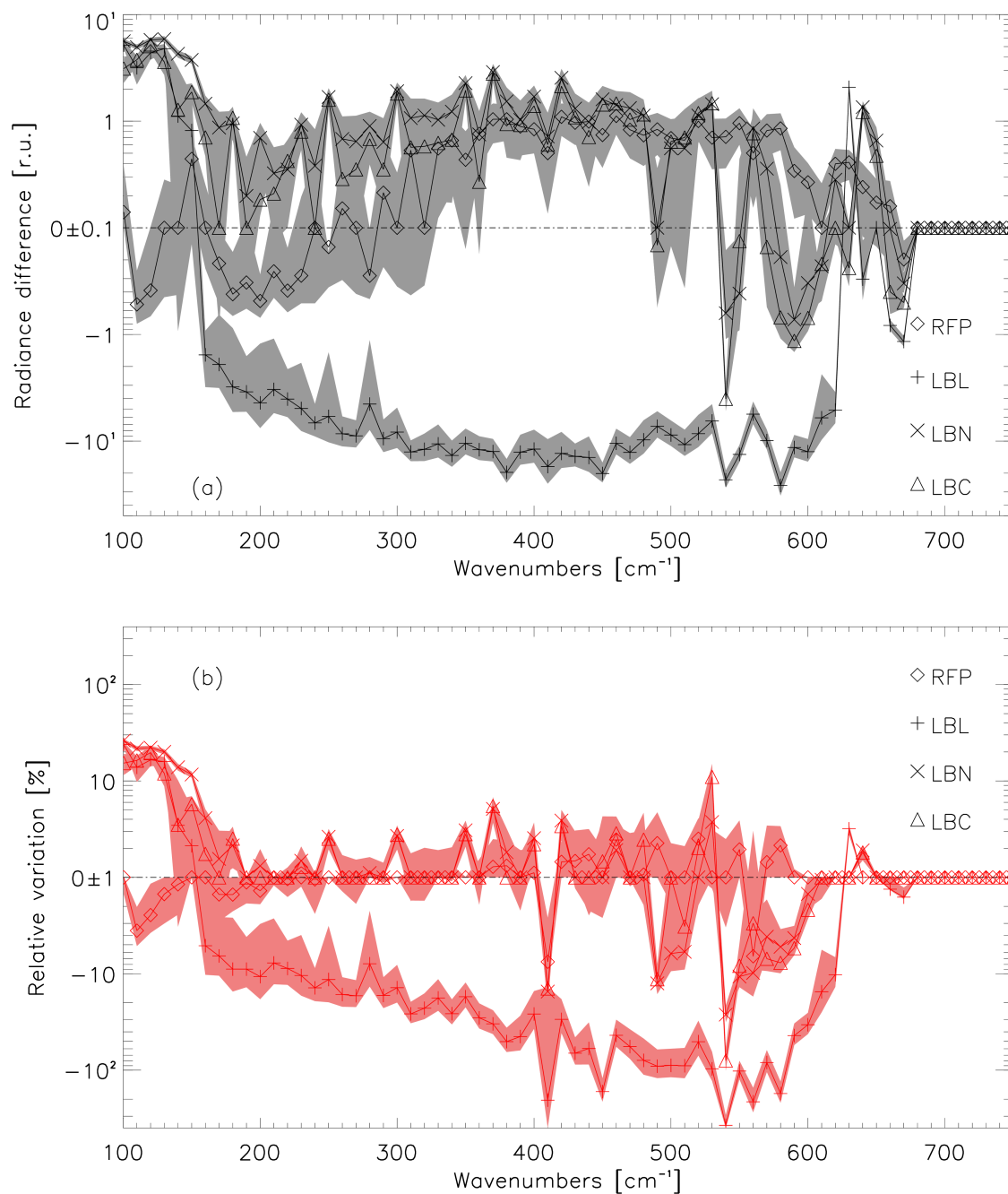
Figure 6. As figure 4(b) for all cases of extension, with (a) the radiance difference and (b) the relative variation, using \diamond for REFIR-PAD (RFP), + for LBLRTM (LBL), \times for LBLRTM with noise (LBN), \Delta for coupled LBLRTM (LBC).
