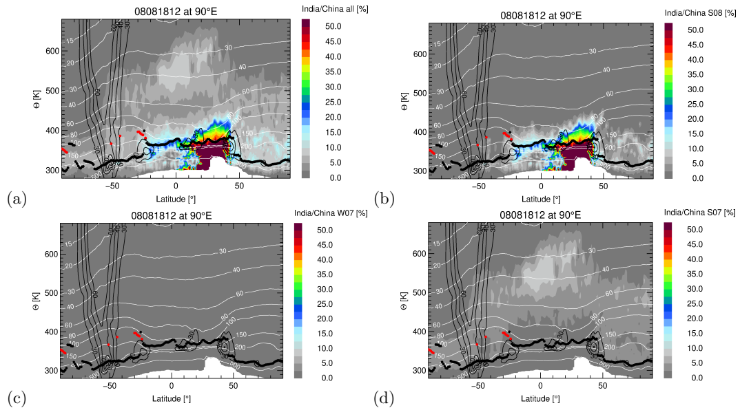
Figure 9. Latitude–theta cross sections at 90^{\circ}\text{E} for the fraction of the India/China tracer for the simulation period (1 May 2007 - 18 August 2008 labeled as ‘all’) (a), for the Summer 08 (S08) pulse (b), for the Winter 07/08 (W07) pulse (c), and for the Summer 07 (S07) pulse (d) on 18 August 2008. The thermal tropopause (primary in black dots and secondary in red dots) and absolute horizontal winds (black lines for 30, 40, 50, and 60 m/s) are shown. The levels of pressure are marked by thin white lines. Note that the maximum value for the Winter 07/08 (W07) pulse (c) is 2.4%.
