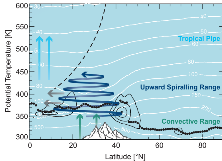
Figure 14. Latitude-theta cross section at about 90^{\circ}\text{E} : The transport of air masses from the region of the Asian monsoon into the tropical pipe occurs in three distinct steps: first, very fast uplift within the convective range up to \approx 360 K within the Asian monsoon anticyclone and outside in the tropical adjacent regions (within a few days); second, uplift above 360 K (up to \approx 460 K) within the upward spiralling range (within a few months), and third, transport within the tropical pipe to altitudes higher than 460 K associated with the large-scale Brewer-Dobson circulation (within \sim one year). The thermal tropopause (black dots) and horizontal winds (black lines) are shown. The horizontal winds mark the edge of the anticyclone at its northern and southern flank. The levels of pressure are marked by thin white lines. Large grey arrows indicate isentropic transport from the Asian monsoon anticyclone into the tropics. The dashed line marks the tropical pipe, which largely isolates tropical air masses from isentropic mixing with mid-latitude air (e.g., Plumb, 1996; Volk et al., 1996).
