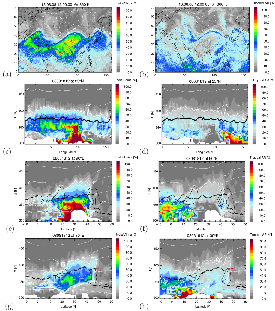
Figure 2. Horizontal distribution of the fraction of air originating in India/China (left) and in tropical adjacent regions (right) at 360 K potential temperature, longitude–theta cross sections at 25°N and latitude–theta cross sections at 90°E (eastern part of the anticyclone) and 30°E (western part of the anticyclone) on 18 August 2008. The horizontal winds are indicated by white arrows (maps) or by black thin lines (cross sections) (shown are 30, 40, 50, and 60 m/s). The primary thermal tropopause is marked by black dots, the secondary thermal tropopause by red dots, and the levels of pressure are marked by thin white lines. The contour line of 20% of the India/China tracer is shown by thick white lines (cross sections).
