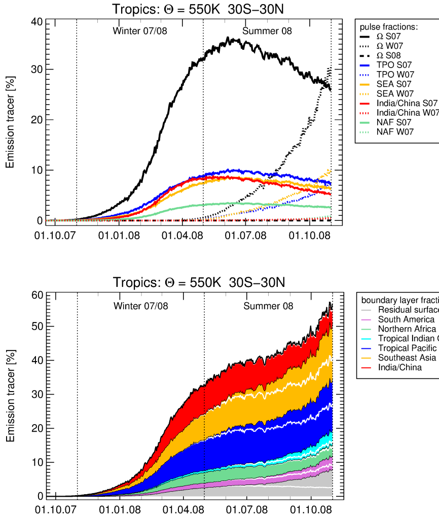
Figure 13. Top: The contribution of the three different time pulses S07, W07, and S08 (each set for a time period of 6 months marked by the vertical dotted lines) for the entire Earth’s surface ( \Omega_{S07} , \Omega_{W07} , \Omega_{S08} ) to the tropical pipe between 30^\circ\text{S} and 30^\circ\text{N} at 550 K potential temperature from 1 October 2007 until the end of the simulation period (31 October 2008) (top, black lines). Emission tracers released during S08 have no contribution to the tropical pipe at 550 K by October 2008. The contribution of several tracers of air mass origin to the individual pulses are shown in colours.
