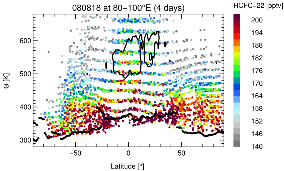
Figure 12. Latitude–theta cross sections of MIPAS HCFC-22 measurements crossing the eastern ( 80^{\circ}\text{E} - 100^{\circ}\text{E} ) mode of the anticyclone up to 680 K potential temperature on 18 August 2008. The thermal tropopause is indicated by black dots. The contour line of 6% of the India/China tracer for the Summer 07 pulse is shown by thick black lines as shown in Fig. 9. To highlight the MIPAS HCFC-22 signal within the tropical pipe the plot range of the data is up to 200 pptv. Note that the maximum values of MIPAS HCFC-22 in the troposphere are higher than 200 pptv.
