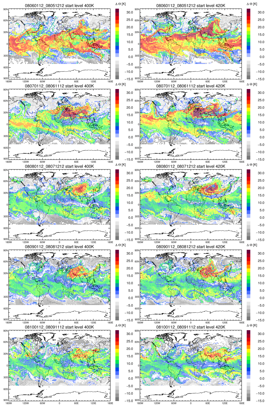
Figure A1. The change in potential temperature ( \Delta\Theta ) along 20-day backward trajectories are shown for different levels of potential temperature (400 K and 420 K) for different days from monsoon-onset until post-monsoon (1st June, 1st July, 1st August, 1st September, and 1st October 2008).
