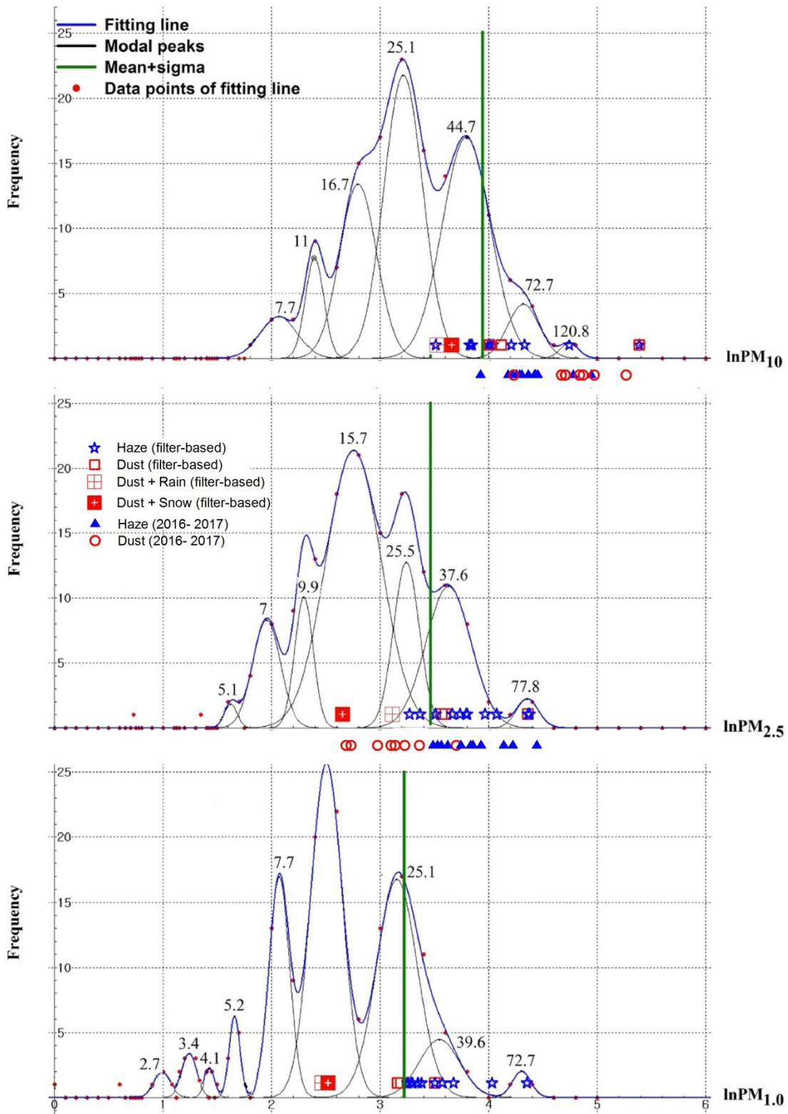
Figure 5. Frequency distributions of \text{PM}_{10} , \text{PM}_{2.5} and \text{PM}_{1.0} mass concentrations for all measurements. Mass concentrations are given as \ln values in x-axis. The green lines stand for mean+SD. The individual samples collected during dust or haze events are marked as different
