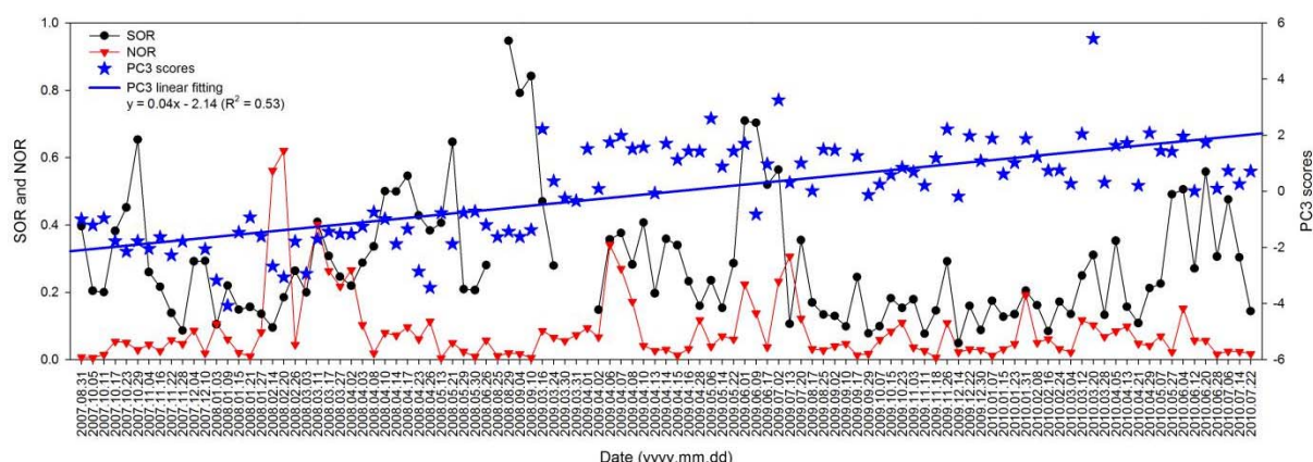
Time series of SOR, NOR, PC3 scores, and linear fitting of PC3.
