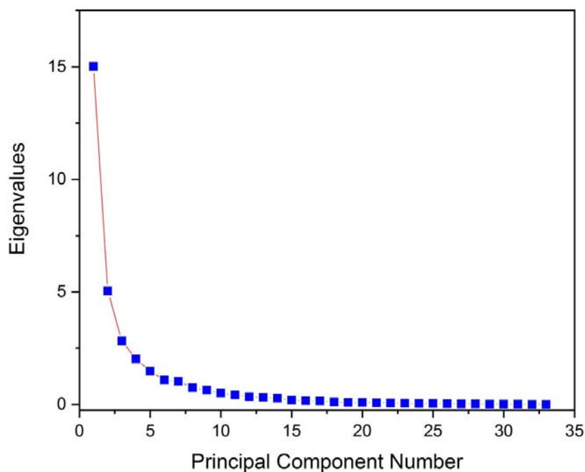
SI 3. Eigenvalues according to the number of principal components.
