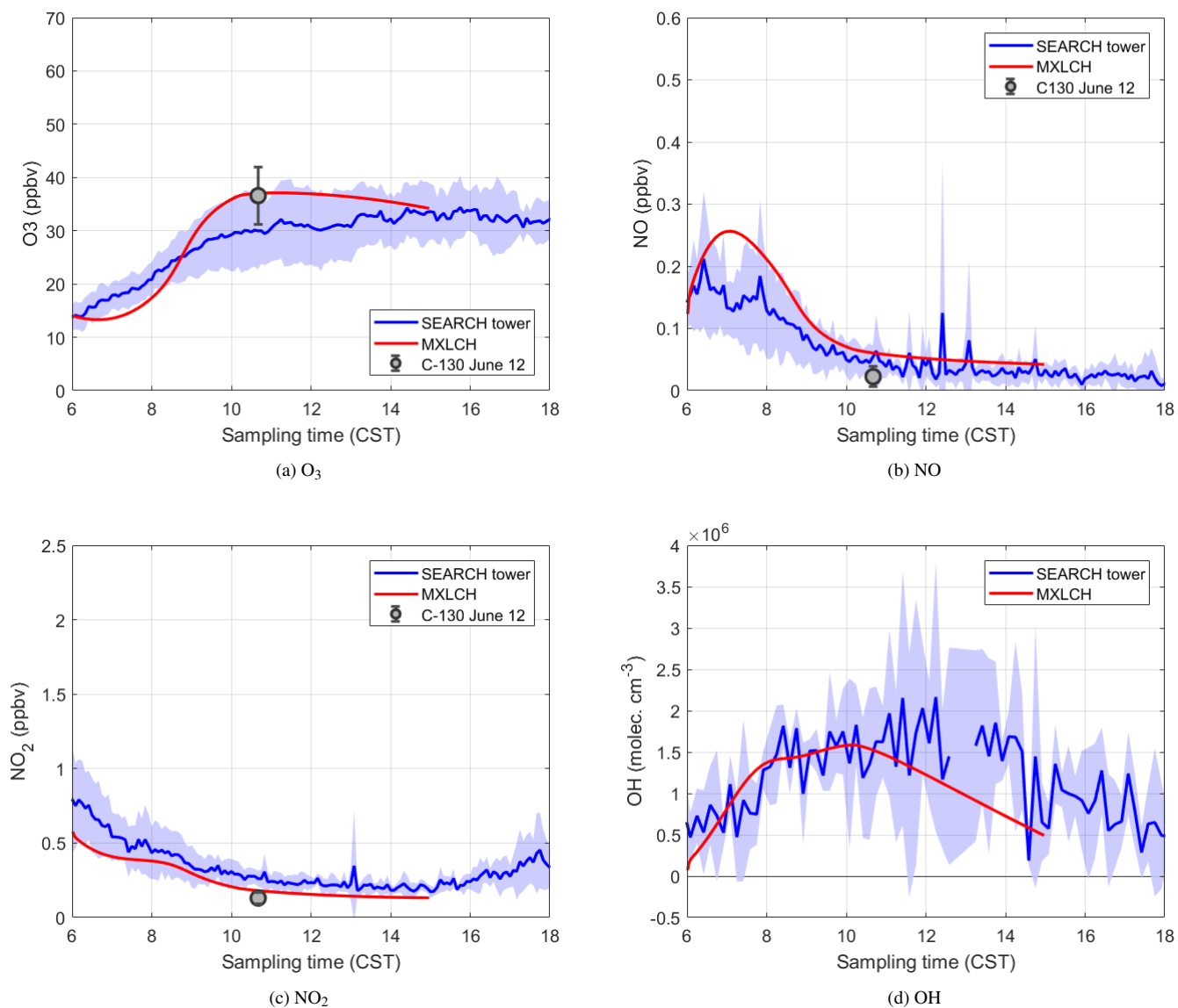
Figure C1. (a) Ozone, (b) nitrogen oxide, (c) nitrogen dioxide and (d) hydroxide (OH) mixing ratio measured (blue) at SOAS super site versus modelled by MXLCH-SOA model (red) over the SOAS super site during the SOAS measurement campaign for the days 5, 6, 8, 10-13 June, 2013.
