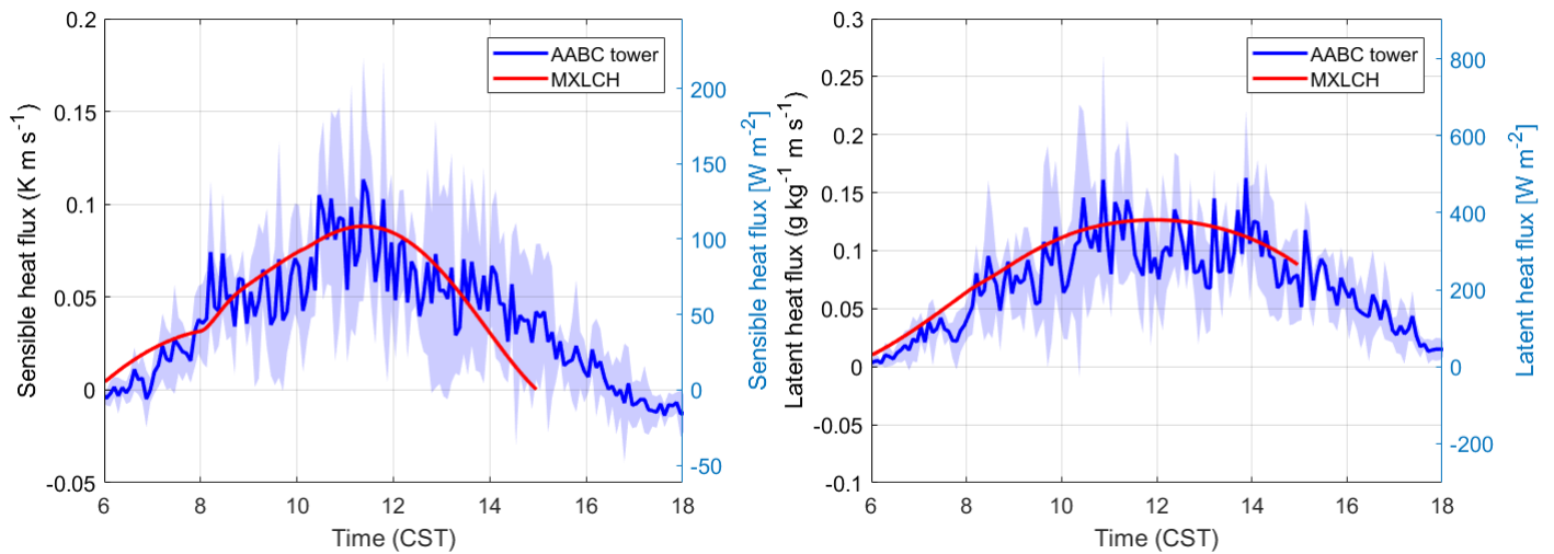
Figure 2. (a) Sensible and (b) latent heat flux measured (blue) and modelled (red) at the Alabama Aquatic Biodiversity Centre (AABC) eddy-covariance tower. The blue shaded area represents the data variability over over June 5, 6, 8, 10-13, 2013, while the solid blue shows the average over these days.
