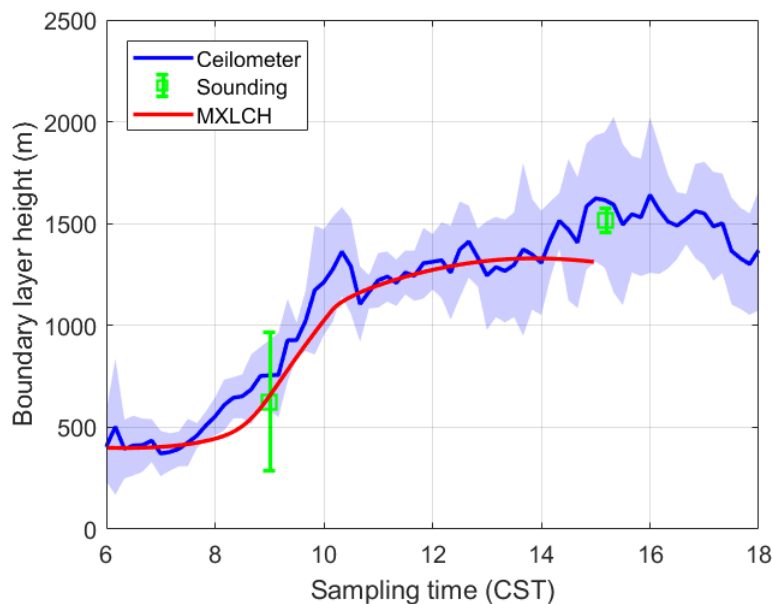
Figure 3. Boundary layer height measured (blue and green) versus modelled by MXLCH-SOA model (red) over the SOAS super site during the SOAS measurement campaign for the days 5, 6, 8, 10-13 June, 2013.
