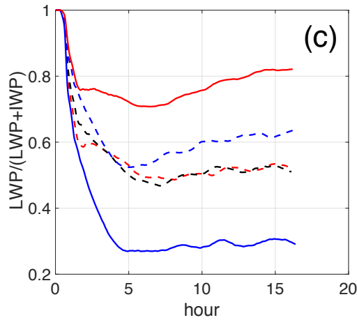
Figure 6: Time series from runs varying CCN concentrations with “linear” ice formation. a) LWP, in units of \text{g m}^{-2} . b) IWP, in units of \text{g m}^{-2} . c) Liquid water fraction for ConIce (dashed) and LinIce (solid). For CCN and INP factors 0.5 (red), 1.0 (black), and 2.0 (blue).
