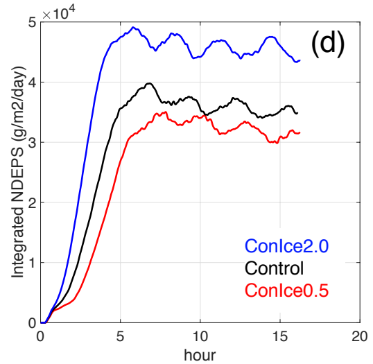
Figure 5: Time series from runs varying CCN concentrations with “constant” ice formation. a) Maximum effective radius, in units of microns. b) Cloud mixed-layer liquid-ice water static energy, in units Kelvin. c) Cloud base ice plus snow number concentration, in units of L^{-1} . d) Vertically integrated net deposition rate, in units of g\ m^{-2}\ day^{-1} . For CCN factors 0.5 (red), 1.0 (black), and 2.0 (blue).
