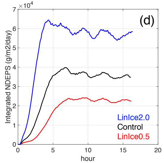
3 Figure 7: Time series from runs varying CCN concentrations with “linear” ice formation. a) 4 4 Maximum effective radius, in units of microns. b) Cloud mixed-layer liquid-ice water static 5 5 energy, in units Kelvin. c) Cloud base ice plus snow number concentration, in units of L^{-1} . d) 6 6 Vertically integrated net deposition rate, in units of g\ m^{-2}\ day^{-1} . For CCN and INP factors 0.5 7 7 (red), 1.0 (black), and 2.0 (blue).
