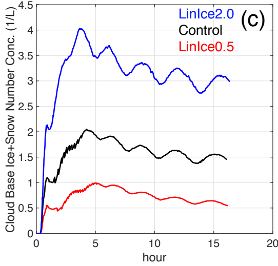
3 Figure 7: Time series from runs varying CCN concentrations with “linear” ice formation. a) 4 4 Maximum effective radius, in units of microns. b) Cloud mixed-layer liquid-ice water static 5 5 energy, in units Kelvin. c) Cloud base ice plus snow number concentration, in units of L^{-1} . d) 6 6 Vertically integrated net deposition rate, in units of g\ m^{-2}\ day^{-1} . For CCN and INP factors 0.5 7 7 (red), 1.0 (black), and 2.0 (blue).
