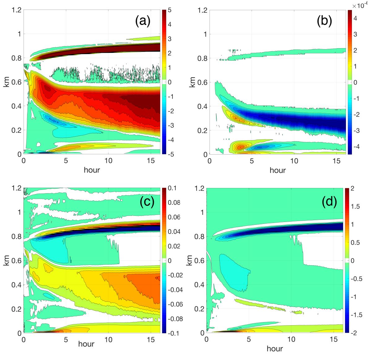
Figure 4: Impact of increasing CCN by 2X (ConIce2.0 minus ConIce1.0) on (a) relative humidity, (b) sublimation rate, (c) water vapor mixing ratio, and (d) temperature, in units of percent, \text{g m}^{-3} \text{s}^{-1} , \text{g kg}^{-1} , ^{\circ}\text{C} , respectively.
