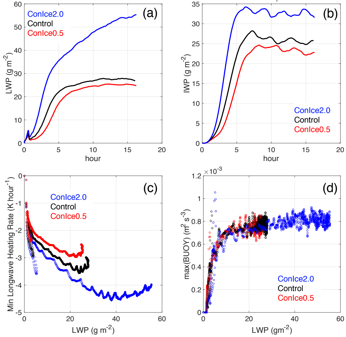
Figure 3: Time series from runs varying CCN concentrations with “constant” ice formation. a) LWP, in units of \text{g m}^{-2} . b) IWP, in units of \text{g m}^{-2} . c) Scatterplot of minimum longwave heating rate vs LWP, in units of \text{K hour}^{-1} and \text{g m}^{-2} , respectively. d) Scatterplot of integrated buoyancy vs LWP, in units of \text{m}^2 \text{s}^{-3} and \text{g m}^{-2} , respectively. For CCN factors 2.0 (blue), 1.0 (black), and 0.5 (red).
