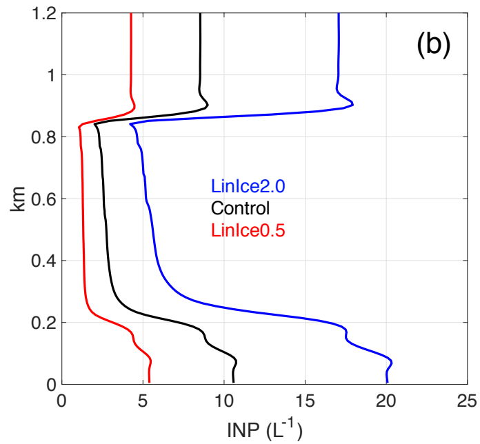
Figure 8: (a) CCN and (b) INP in “linear” ice runs at hour 10, in units of \text{cm}^{-3} and \text{L}^{-1} , respectively. For CCN and INP factors 0.5 (red), 1.0 (black), and 2.0 (blue).
