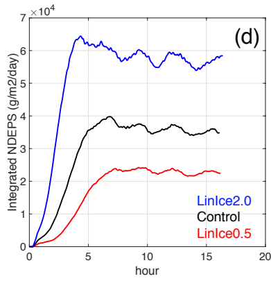
3 Figure 7: Time series from runs varying CCN concentrations with “linear” ice formation. a) 4 Maximum effective radius, in units of microns. b) Cloud mixed-layer liquid-ice water static 5 energy, in units Kelvin. c) Cloud base ice plus snow number concentration, in units of L^{-1} . d) 6 Vertically integrated net deposition rate, in units of g\ m^{-2}\ day^{-1} . For CCN and INP factors 0.5 7 (red), 1.0 (black), and 2.0 (blue).
