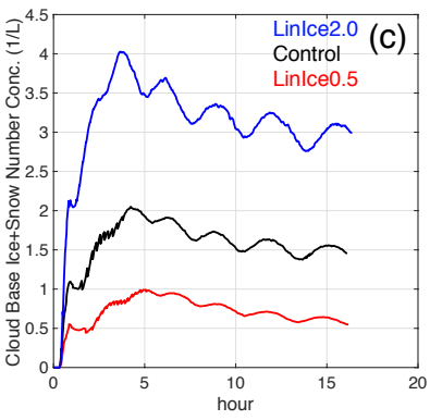
3 Figure 7: Time series from runs varying CCN concentrations with “linear” ice formation. a) 4 Maximum effective radius, in units of microns. b) Cloud mixed-layer liquid-ice water static 5 energy, in units Kelvin. c) Cloud base ice plus snow number concentration, in units of L^{-1} . d) 6 Vertically integrated net deposition rate, in units of g\ m^{-2}\ day^{-1} . For CCN and INP factors 0.5 7 (red), 1.0 (black), and 2.0 (blue).
