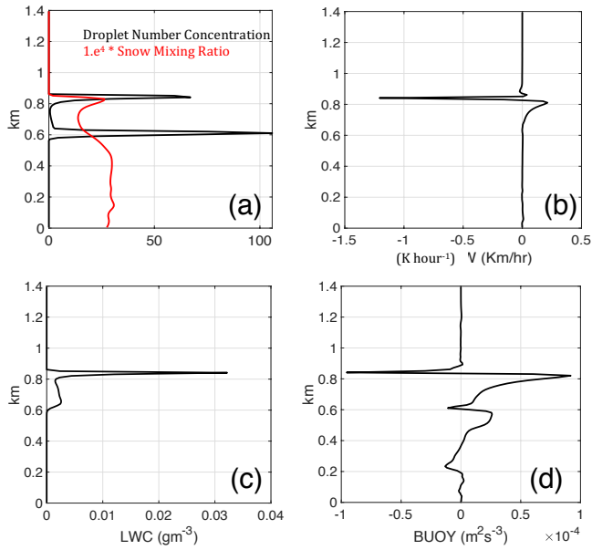
Figure 9: Impact of prognostic CCN (LinIce2.0-FixCCN2.0) over hour 10. a) Droplet number concentration (black) and snow mixing ratio (red), in units of cm -3 and 1.e 4 *g kg -1 , respectively. b) Longwave radiative heating rate, in units of K hour -1 . c) Liquid water content, in units of g m -3 . d) Buoyancy, in units of m 2 s -3 .
