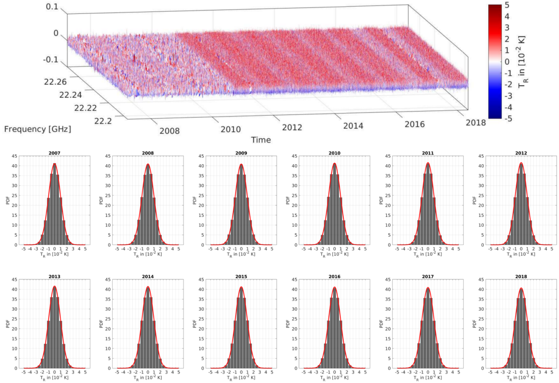
Figure 1. The 3-D plot in the top shows the temporal evolution of the MIAWARA residuals (difference between measured difference spectrum and modeled spectrum) as residuum brightness temperature fluctuations T_R in [10^{-2} \text{ K}] within the frequency range of 22.195 GHz to 22.275 GHz (80 MHz bandwidth) from 2007 to 2018.
