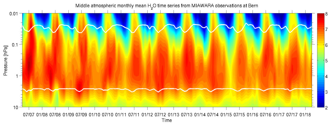
Figure 2. Monthly mean water vapor time series in [ppm] obtained by the MIAWARA instrument located at the Zimmerwald observatory near Bern between April 2007 and May 2018. The horizontal upper and lower white lines indicate the pressure layer within which the measurement response is higher than 80%. This data set is used as input for the trend model.
