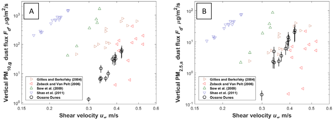
5 Figure 2: The vertical dust mass flux as a function of shear velocity within (A) the PM_{10,g} geometric diameter range and (B) the PM_{2.5,a} aerodynamic diameter range. Each of the two plots includes measurements at Oceano (black open circles), and previously published field studies of natural dust emissions from non-sandy soils (open triangles). These latter measurements were compiled in Kok et al. (2014a), which corrected these measurements to the PM_{10,g} geometric diameter range following the procedure described in that work. Furthermore, we corrected these measurements to the PM_{2.5,a} aerodynamic diameter range assuming that their PSDs follow the prediction of brittle fragmentation theory generated by aggregate fragmentation (Kok, 2011). Error bars on the Oceano measurements were obtained through error propagation (details in Supplement). 10
