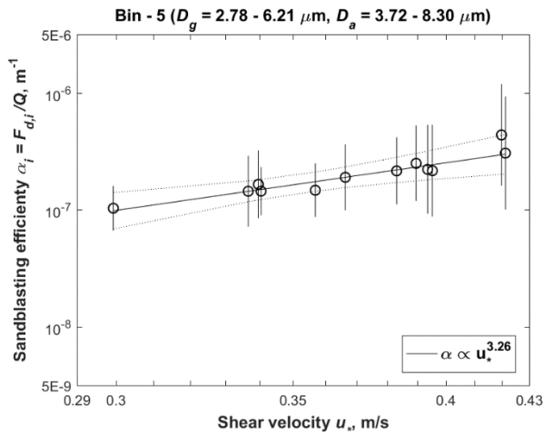
Figure 6: The sandblasting efficiency \alpha_i ( \text{m}^{-1} ) of the six size bins at Oceano as a function of shear velocity. The linear-least squares fit (black line) indicates that \alpha_i varies as a power law in shear velocity with an exponent of 4.71 \pm 0.97 , 5.00 \pm 1.37 , 5.22 \pm 1.63 , 6.12 \pm 2.11 , 3.26 \pm 1.90 , and -2.89 \pm 1.94 for the six respective size bins. Error bars were obtained by propagating errors from the sensor intercalibration process, the regression used in the gradient method, and the subtraction of the sea-salt deposition flux (see Supplement). The two black dotted lines denote the 95% confidence range of the fit. The geometric and the aerodynamic diameter ranges of the vertical dust mass flux F_{d,i} are noted at the top of each of the six plots, and Q is the total horizontal sand flux integrated over all sand grain sizes (Martin et al., 2018).
