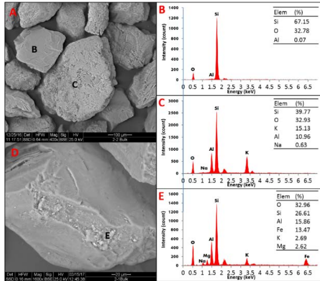
5 Figure 8: (A) Scanning Electron Microscopy (SEM) image of an Oceano sand sample. (B) Energy Dispersive X-ray Spectroscopy (EDS) chemical composition (percentage by mass) of a quartz grain in image A (the location of the analysis is marked by the black letter “B”). (C) EDS chemical composition of a K-rich feldspar in image A marked by “C”. (D) Close-up image of a quartz sand grain with mineral coatings. (E) EDS chemical composition of the mineral coatings in image D marked by “E”.
