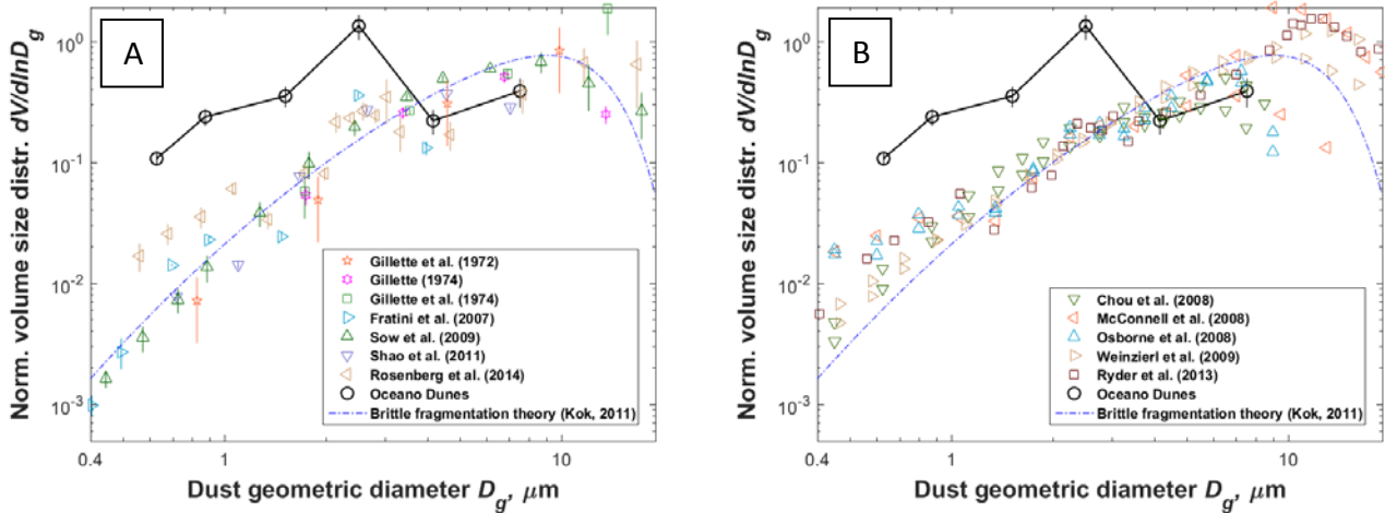
15 Figure 3: Normalized volume particle size distribution (PSD) of dust at emission as a function of dust aerosol geometric diameter averaged over all measurements at Oceano (black open circles). Plotted for comparison are measurements compiled by Kok et al. (2017) of (A) the emitted dust PSDs from non-sandy soils in the U.S. (Gillette et al., 1972; 1974; Gillette, 1974), China (Fratini et al., 2007), North Africa (Sow et al., 2009; Rosenberg et al., 2014), and Australia (Shao et al., 2011), and (B) in situ aircraft measurements of dust-dominated
