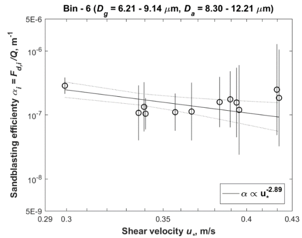
Figure 6: The sandblasting efficiency \alpha_i ( \text{m}^{-1} ) of the six size bins at Oceano as a function of shear velocity. The linear-least squares fit (black line) indicates that \alpha_i varies as a power law in shear velocity with an exponent of 4.71 \pm 0.97 , 5.00 \pm 1.37 , 5.22 \pm 1.63 , 6.12 \pm 2.11 , 3.26 \pm 1.90 , and -2.89 \pm 1.94 for the six respective size bins. Error bars were obtained by propagating errors from the sensor intercalibration process, the regression used in the gradient method, and the subtraction of the sea-salt deposition flux (see Supplement). The two black dotted lines denote the 95% confidence range of the fit. The geometric and the aerodynamic diameter ranges of the vertical dust mass flux F_{d,i} are noted at the top of each of the six plots, and Q is the total horizontal sand flux integrated over all sand grain sizes (Martin et al., 2018).
