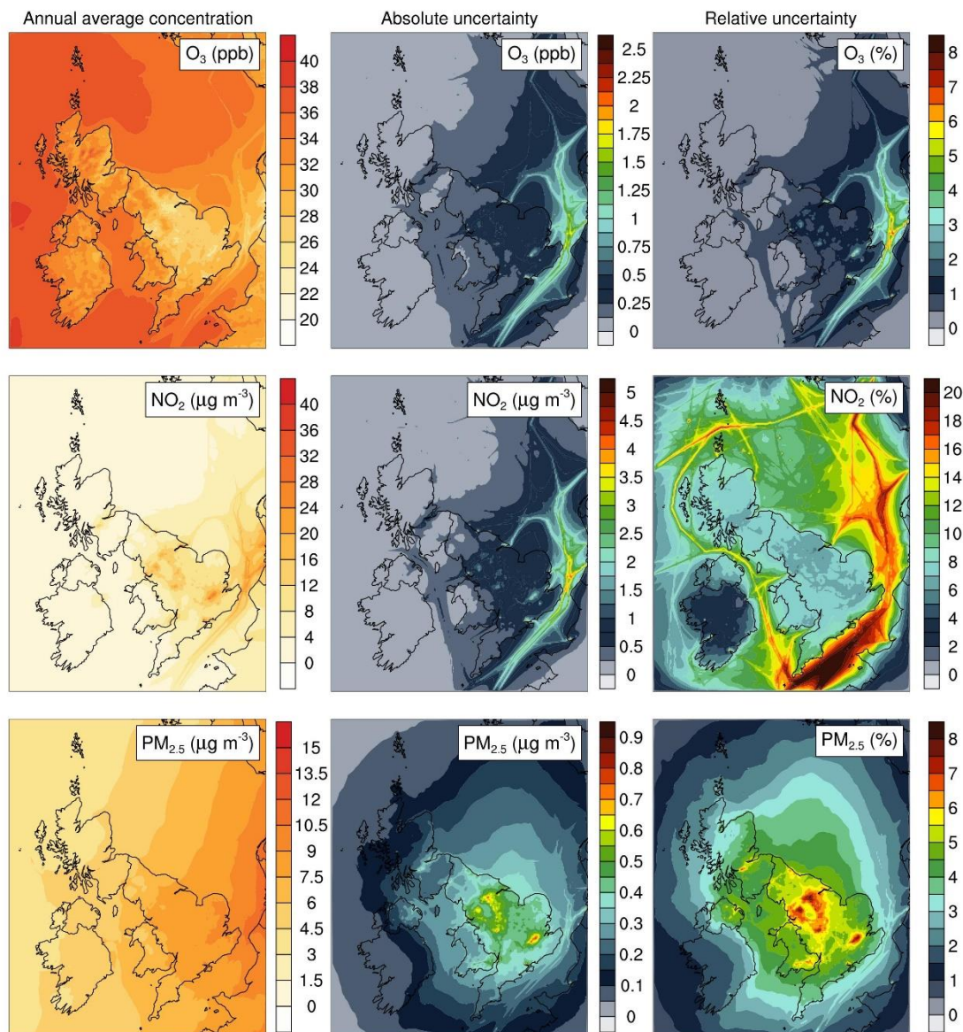
Figure 2 Baseline surface concentrations of O_3 , NO_2 , and PM_{2.5} , and their respective spatial distributions of the absolute and relative uncertainties (at the 5\ km \times 5\ km model grid resolution, year 2012) for the specified uncertainties in UK emissions. The uncertainty values are represented as a range of \pm the baseline value and represent the 95% confidence interval.
