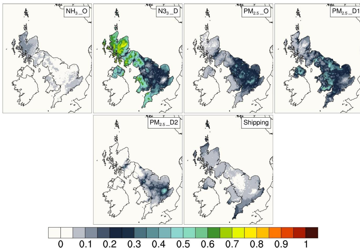
5 Figure 5 Spatial distributions (at the 5km×5km model grid resolution) of the first-order sensitivity indices for modelled surface concentrations of \text{PM}_{2.5} . D indicates emissions from a dominant sector and O indicates grouped emissions from the rest of the sectors. For \text{NH}_3 emissions dominant sector is agriculture, for \text{PM}_{2.5} dominant sectors are residential and non-industrial combustion (D1) and road transport (D2). Shipping emissions variable combines emissions of all relevant pollutants.
