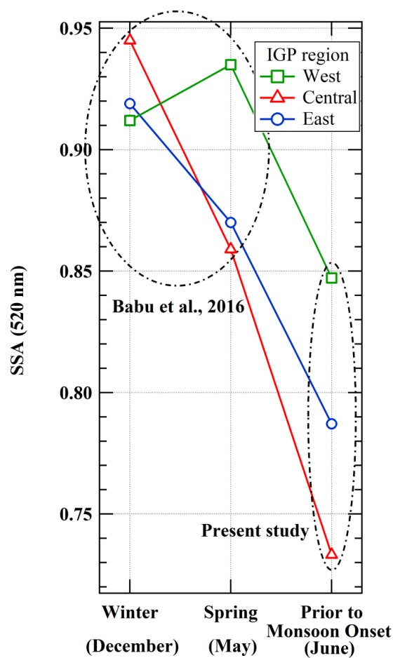
Figure 6: Seasonal variation of columnar (500 m - 3000 m) SSA over different regions of the IGP: west (square), central (triangle), and east (circle). Values in the upper left circle are taken from Babu et al., 2016.
