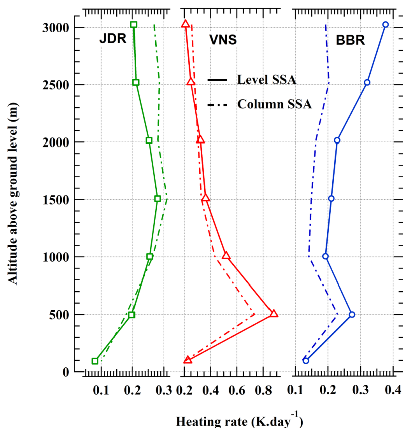
5 Figure 9: Altitudinal heating rate profiles for the stations i) JDR (left), ii) VNS (center), and BBR (right). Solid lines are for heating profiles calculated using in-situ aircraft profile data and layer averaged aerosol properties. Dash dot line represent heating profiles calculated using in-situ aircraft profile data and column averaged aerosol SSA.
