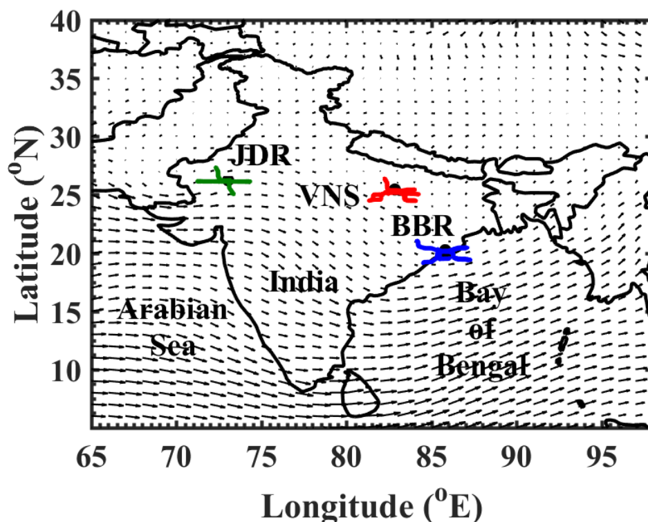
10 Figure 1: Geographical location of the aircraft campaign stations (solid circle) in the Indo Gangetic Plain superimposed on the mean wind field at 850 hPa during the campaign period. JDR, VNS & BBR stands for Jodhpur, Varanasi and Bhubaneswar, respectively. Daily flight tracks are superimposed on the stations JDR (green), VNS (red) and BBR (blue), from left to right, respectively. Each measurement track has a horizontal span of ~ 150 km from the base station.
