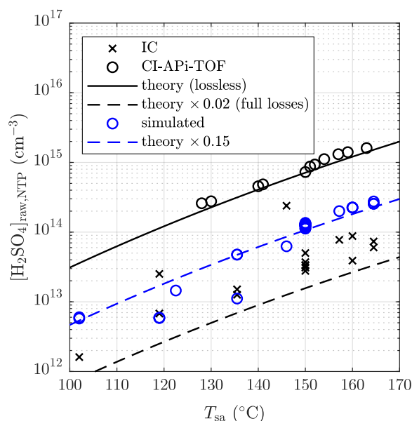
Figure 10. Simulated sulfuric acid concentrations in the raw sample compared with the measured and the theoretical concentrations with different sulfuric acid evaporator temperatures.
