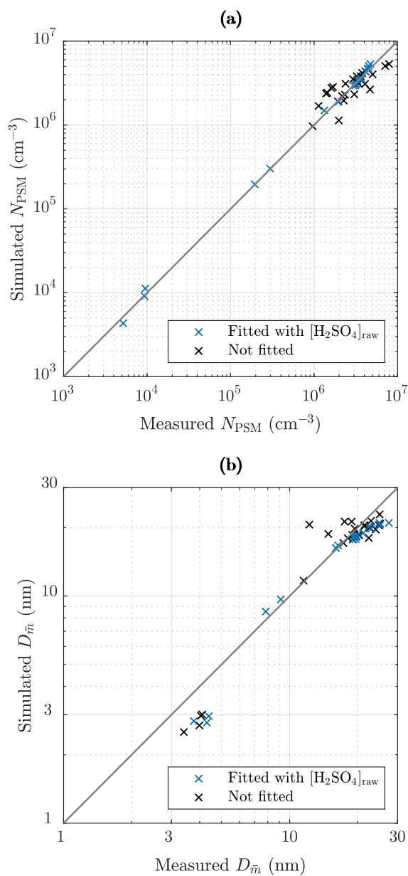
Figure 14. Comparison of the simulated and the measured (a) number concentrations of the particles larger than \sim 1.3 nm and (b) the diameters with the average mass after the ED. The blue crosses represent the cases for which N_{\text{PSM}} and D_{\bar{m}} were obtained by fitting the value of [\text{H}_2\text{SO}_4]_{\text{raw}} . The black crosses represent the cases of the measurement sets 2 ... 4 in which the values of [\text{H}_2\text{SO}_4]_{\text{raw}} originated from an another case of the measurement set having the same T_{\text{sa}} value.
