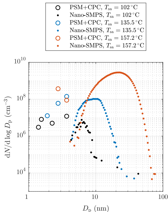
Figure 5. Examples of particle size distributions after the ED measured with different \text{H}_2\text{SO}_4 evaporator temperatures in the measurement set 1. The data are corrected with the DR of the BD and with the diffusional losses in the sampling lines after the ED. The concentrations are multiplied with the total DR of the sampling system.
