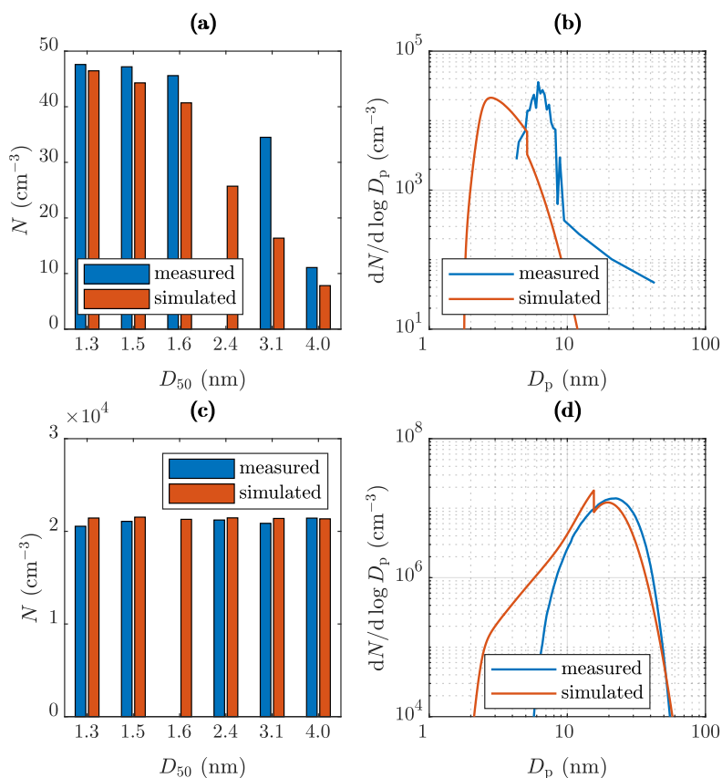
Figure 11. Examples of measured and simulated (a) number concentrations from the PSM and the CPC 3775 with T_{sa} = 102^\circ\text{C} , (b) size distributions from the Nano-SMPS with T_{sa} = 102^\circ\text{C} , (c) number concentrations from the PSM and the CPC 3775 with T_{sa} = 157.2^\circ\text{C} , and (d) size distributions from the Nano-SMPS with T_{sa} = 157.2^\circ\text{C} . The D_{50} values in the range of 1.3...3.1 nm represent the cut-sizes of the PSM with different saturator flow rates and the D_{50} value of 4.0 nm represents the cut-size of the CPC 3775.
