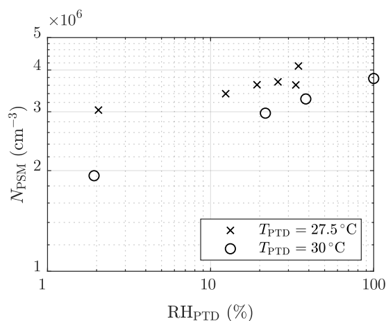
Figure 7. The measured number concentrations of the particles larger than \sim 1.3 nm of the measurement set 2 as a function of the RH of the PTD dilution air. The concentrations are multiplied with the total DR of the sampling system.
