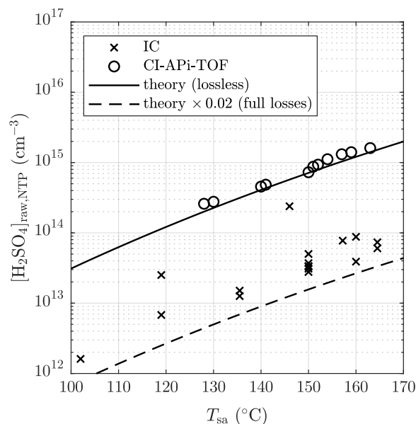
Figure 4. Measured and theoretical sulfuric acid concentrations in the raw sample with different sulfuric acid evaporator temperatures. The lossless theoretical level represents the concentrations if the diffusional losses onto the sampling lines between the \text{H}_2\text{SO}_4 evaporator and the [\text{H}_2\text{SO}_4]_{\text{raw}} measurement point are neglected. The theoretical level with full losses represent the concentrations if the sampling lines are fully condensing.
