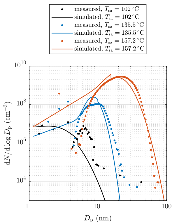
Figure 12. Examples of measured and simulated particle size distributions after the ED. The measured data are corrected with the DR of the BD and with the diffusional losses in the sampling lines after the ED. Additionally, all concentrations are multiplied with the total DR of the diluting sampling system.
