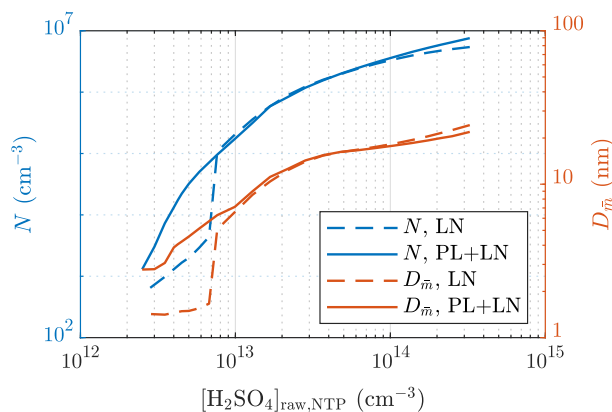
Figure 13. Comparison of the particle number concentrations and the diameters with the average mass after the ED simulated using the LN distribution only and using both the PL and the LN distributions.
