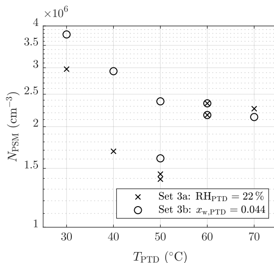
Figure 8. The measured number concentrations of the particles larger than \sim 1.3 nm of the measurement set 3 as a function of the T of the PTD dilution air. The concentrations are multiplied with the total DR of the sampling system.
