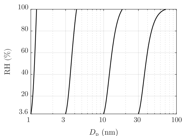
Figure 9. Examples of particle diameters in different humidities in the temperature of 23^\circ\text{C} . The lowest RH value represents the RH of the dilution air of the ED.
