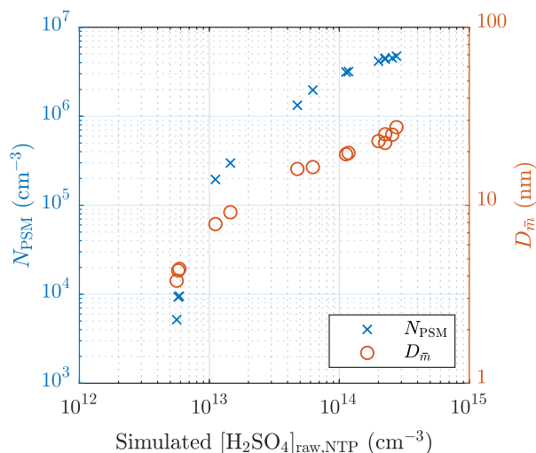
Figure 6. The measured number concentrations of the particles larger than \sim 1.3 nm and the diameters with the average mass of the measurement set 1 as a function of the simulated \text{H}_2\text{SO}_4 concentration in the raw sample. The concentrations are multiplied with the total DR of the sampling system.
