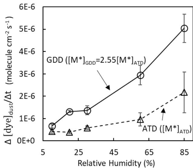
Figure 3: The dye degradation rate in the presence of ATD or GDD particles measured using a UV flow chamber under RH levels ranging from 10% to 85%. As a control, the photodegradation of malachite green in the absence of dust was measured, but the degradation was negligible. The error bars represent the standard deviations.
