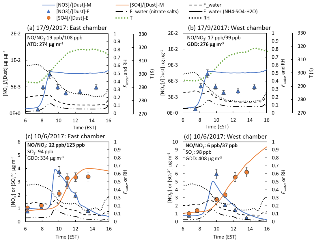
Figure 4: Simulation of the outdoor chamber data using the AMAR model for (A) ATD (2017-09-17) and (B) GDD (2017-09-17) particles in the presence of \text{NO}_x and \text{SO}_2 oxidation on GDD particles in the presence of (C) high \text{NO}_x (2017-06-10) and (D) low \text{NO}_x (2017-06-10) concentrations. F_{\text{water}}(\text{nitrate salts}) and F_{\text{water}}(\text{NH}_4^+-\text{SO}_4^{2-}-\text{H}_2\text{O}) are the second and third terms in Eq. (1) and represent the additional absorbed water by alkaline nitrate salts and the ammonium sulfate system, respectively. The simulation result was not correct for particle loss.
