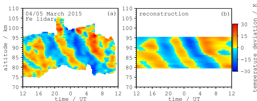
Figure 6. Temperature observations with the Fe lidar (a) and the reconstruction using the 4 harmonic components (b) derived in the analysis.
