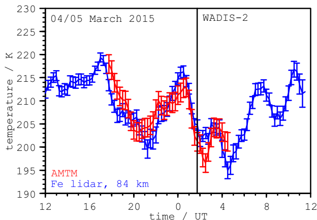
Figure 9. Time series of OH temperatures (red) in comparison with the Fe lidar temperatures (blue). Lidar temperatures are averaged in altitude with a Gaussian weighting of 9 km FWHM and peak altitude of 84 \pm 1 km. Temperatures of the AMTM are taken from a sub-array of 9 \times 9 pixels at the locations of the Fe lidar and smoothed by a 60 min running mean.
