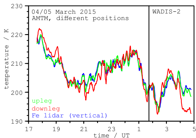
Figure 8. Temporal evolution of AMTM temperature observations derived from sub-arrays of 9 \times 9 pixels (about 5 \times 5 \text{ km}^2 ) at the centre (blue), the rocket upleg (green), and the rocket downleg (red), respectively. The time series is smoothed with a Hanning filter of 5 min width.
