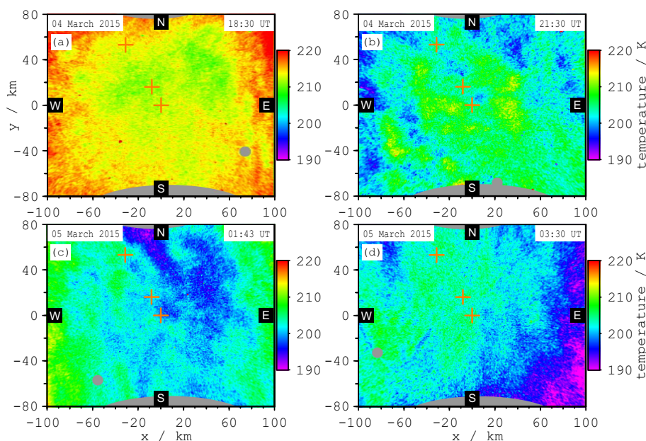
Figure 7. Temperature maps measured with the AMTM. In (a), (b) and (d) the typical situation during the observation time is shown. (c) shows the situation at the rocket launch time. Very little gravity wave activity is apparent, which was the typical condition during this night.
