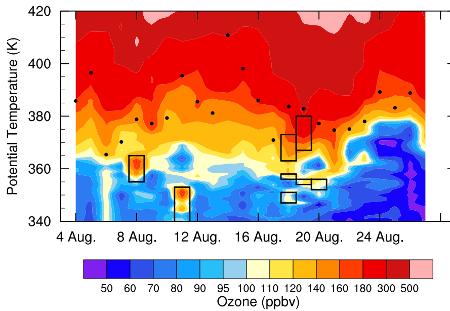
Figure 1. Daily variations of ozone mixing ratios (OMR) between 340 K and 420 K during 4–27 August 2013 from balloon measurements launched in Lhasa. The black dots represent the lapse rate tropopause. High tropospheric ozone is shown by the black rectangle.
