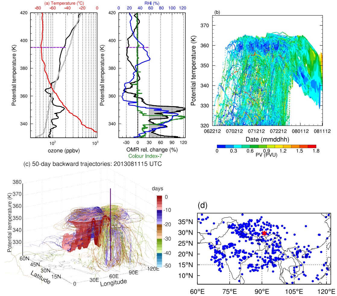
Figure 3. The same as Fig. 2 except for (c) but on 11 August 2013. (a) Colour index (CI) minus 7 ( \text{CI}-7 > 0 marks the cirrus cloud layer, green line). (c) Three-dimensional backward trajectories colour-coded by days.
