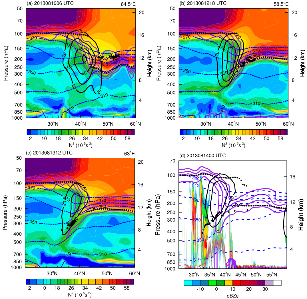
Figure 9. Latitude–pressure cross section of the square of the Brunt–Vaisala frequency ( N^2 ) along the average longitude of the bottom air parcels in Fig. 5b on (a) 10 August at 06:00 UTC, (b) 12 August at 18:00 UTC, (c) 13 August at 12:00 UTC with potential temperature (blue dashed lines, K), PV (purple lines, PVU), tropopause (black dots, hPa), zonal wind (black lines) from ERA-Interim , and air parcels (diamonds) from CLaMS trajectory model . (d) The same as Figure 6a except for radar reflectivity (dBZe) but on 14 August at 00:00 UTC from CloudSat .
