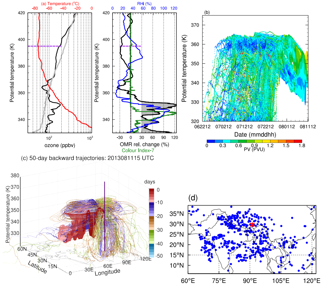
Figure 3. The same as Fig. 2 except for (c) but on 11 August 2013. (a) Colour - Colour index (CI) minus 7 (CI-7>0 marks the cirrus cloud layer, green line). (c) 3-dimensional - Three-dimensional backward trajectories colour-coded by days.
