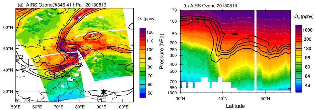
Figure 8. (a) Ozone volume mixing ratio for 346.41 hPa on 13 August at about 06:00 UTC from AIRS satellite. (b) Latitude–pressure cross section of ozone along 70° E with PV (2, 4, 6, and 8 PVU, black line).
