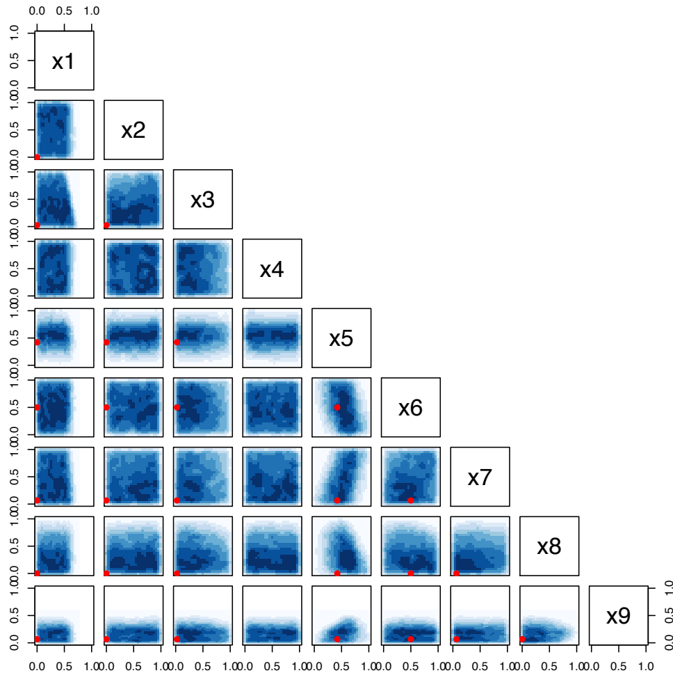
Figure 5. Pairs density plots for input parameters, showing The blue shading in each panel indicates the density of plausible cases, for each pair of input parameters ( x_1 - x_9 ). Plausible cases are defined as the subset of n = 100,000 emulated samples that have with SS > 0.85 , and AOD < 0.08 . Darker shading indicates higher density, and white areas indicate very low density. The default values for each parameter in CAM4 are indicated by red lines-dots in the panel each panel (except for x_4 , which has no default).
