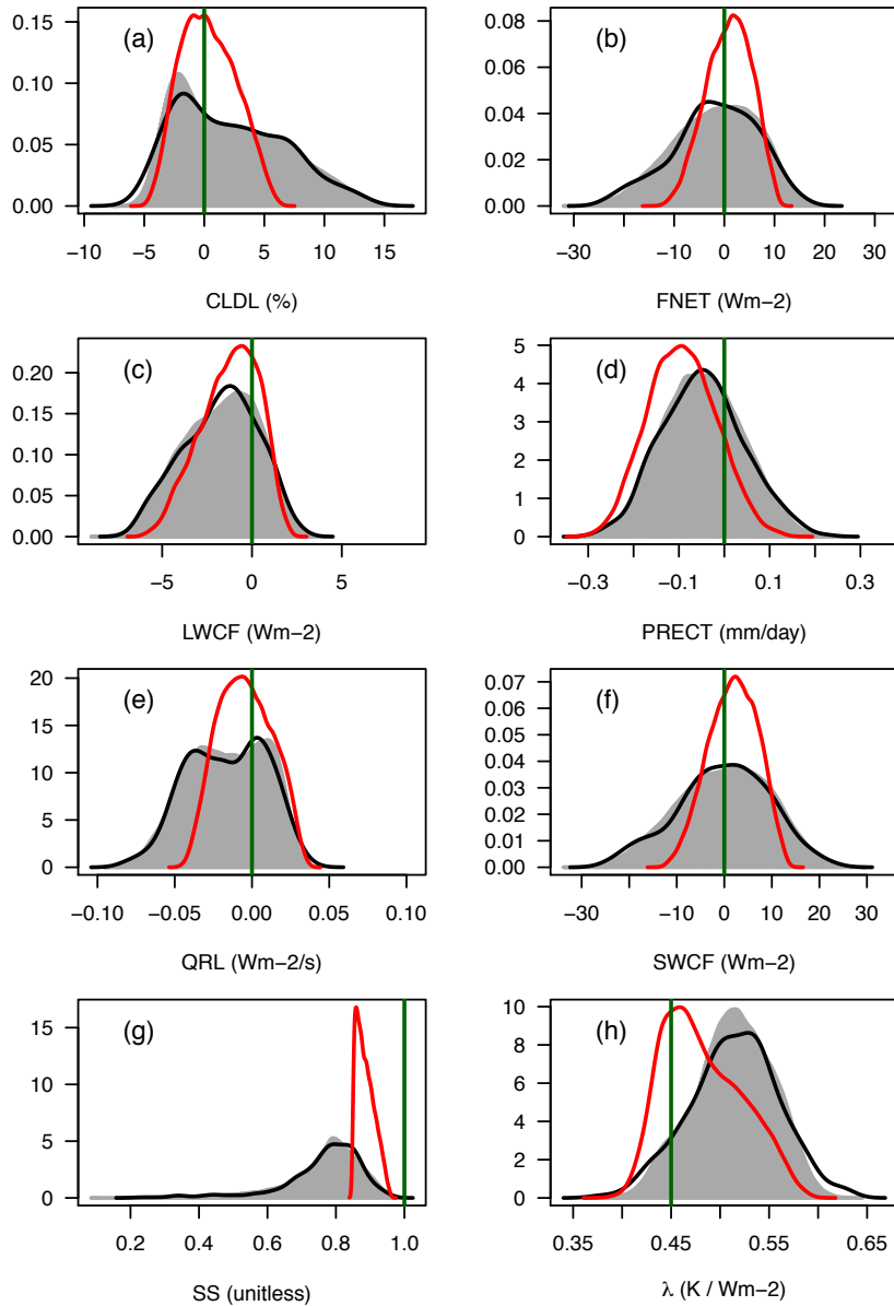
Figure 2. The black line in each panel shows the density distribution of simulated values from CAM4 for each output variable in (a) CLDL, (b) FNET, (c) LWCF, (d) PRECT, (e) QRL, (f) SWCF, (g) multivariate skill score (SS), and (h) Cess climate sensitivity ( \lambda ), from the n = 350 training cases (variable names are defined in the text). The gray shaded region shows the density distribution from 100,000 emulated samples of each output variable, and the red line shows the density distribution for the subset of emulated samples that is most plausible (see Section 4.3). Note the different x-axis scales in each panel, and (for the upper six panels only) a value of zero corresponds to a perfect representation of the global mean in the default model. The dark green vertical line in each panel indicates the default model value location of ESCAM4 with its default parameter settings.
