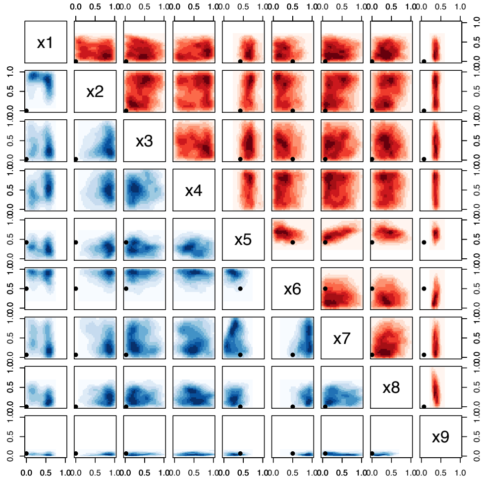
Figure 6. As Fig. 5, except only that panels with blue shading (lower triangle) are for the subset of cases in the lowest 2.5% with values of the distribution of Cess climate sensitivity ( \lambda < 0.418 \text{ K/Wm}^{-2} ), and panels with red shading (upper triangle) are for the subset of cases with high values of \lambda ( \lambda > 0.538 \text{ K/Wm}^{-2} ). The default values for each parameter in CAM4 are indicated by black dots in each panel (except for x_4 , which has no default).
