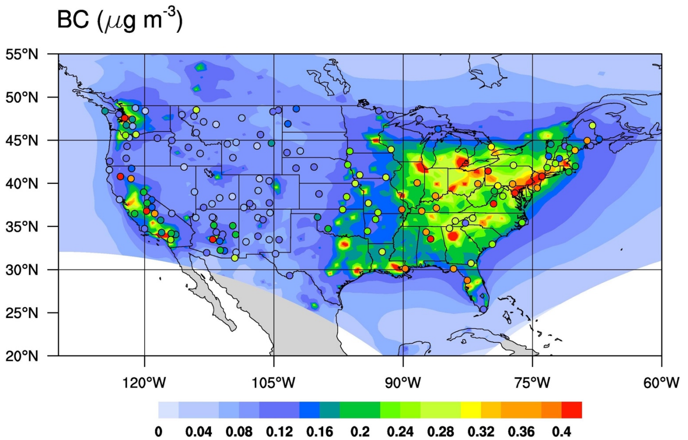
Figure 7: Annual average surface BC concentration over the U.S. The simulated BC concentration (solid contours) for April 2008 to Mar 2009 are compared to observations (circles) from IMPROVE network. The circles indicate IMPROVE sites with the color representing the BC concentration in \mu\text{g/m}^3 . This figure is generated using NCAR Command Language (NCL) version 6.3.0, open source software free to public, by UCAR/NCAR/CISL/TDD, http://dx.doi.org/10.5065/D6WD3XH5 .
