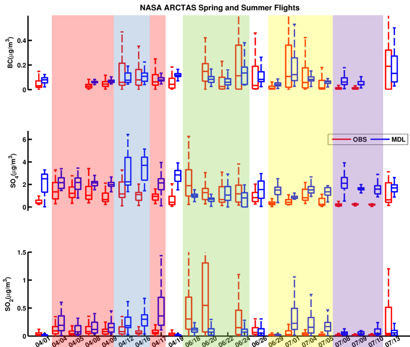
Figure 3: Comparison of BC, sulfate ( \text{SO}_4 ), and \text{SO}_2 for NASA ARCTAS spring and summer flights. Flight categories are shaded same as figure 3. Each flight category is shaded with a different color and the spring and summer transition flights are not shaded. Spring Alaska local flights and spring Greenland flights are shaded blue and red respectively. Green, yellow, and purple shades denote the summer California flights, summer Canada flights, and summer Canada Greenland flights. In each box whisker panel, the middle line denotes the median value, while the edges of the box represent 25th and 75th percentile values respectively. The whiskers denote the maximum and minimum values.
