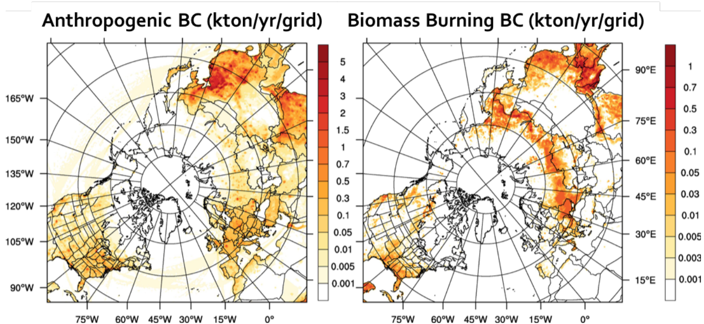
Figure 1: Spatial distribution of anthropogenic BC emissions (left) and wildfire BC emissions (right) in Gg/yr/grid. This figure is generated using NCAR Command Language (NCL) version 6.3.0, open source software free to public, by UCAR/NCAR/CISL/TDD, http://dx.doi.org/10.5065/D6WD3XH5 .
