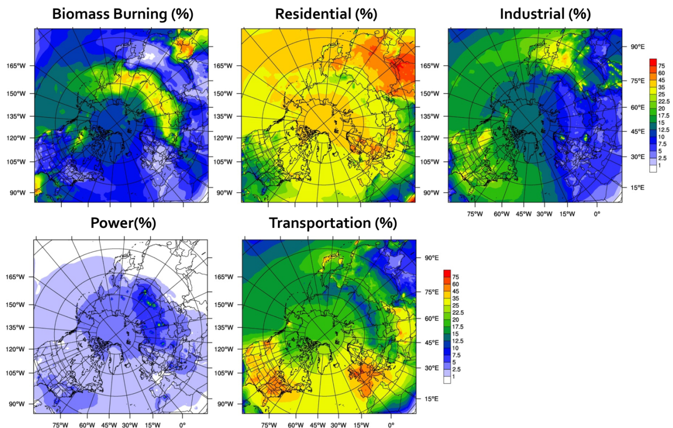
Figure 9: Spatial distribution of source sector contributions (%) to annual BC surface concentration over the entire domain. This figure is generated using NCAR Command Language (NCL) version 6.3.0, open source software free to public, by UCAR/NCAR/CISL/TDD, http://dx.doi.org/10.5065/D6WD3XH5 .
