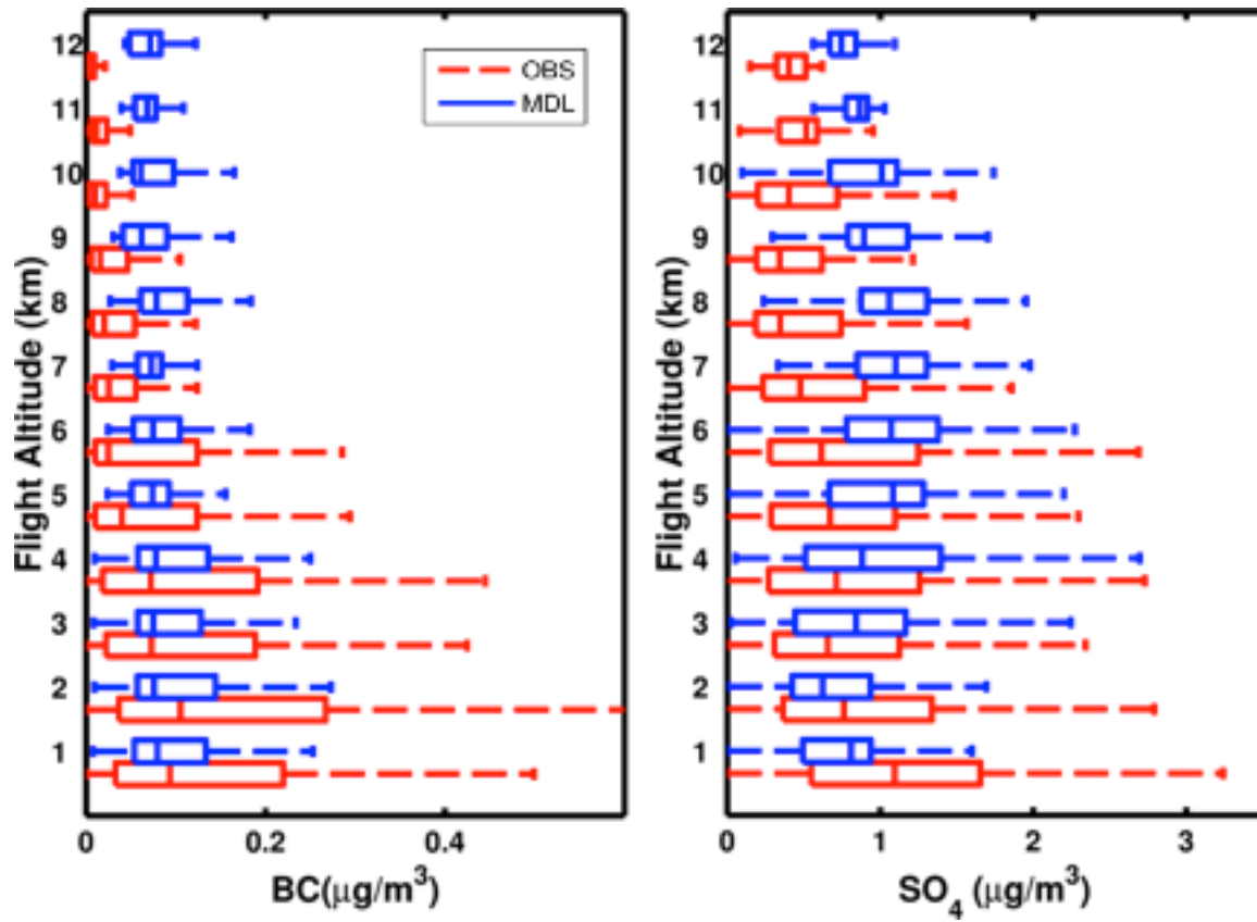
Figure 4: Comparison of model and observation BC and sulfate ( \text{SO}_4 ) for all ARCTAS flights. In each box whisker panel, the middle line denotes the median value, while the edges of the box represent 25 th and 75 th percentile values respectively. The whiskers denote the maximum and minimum values.
